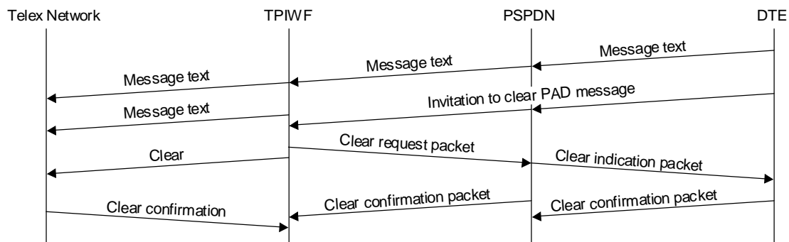
a) Invitation to clear PAD message from DTE
