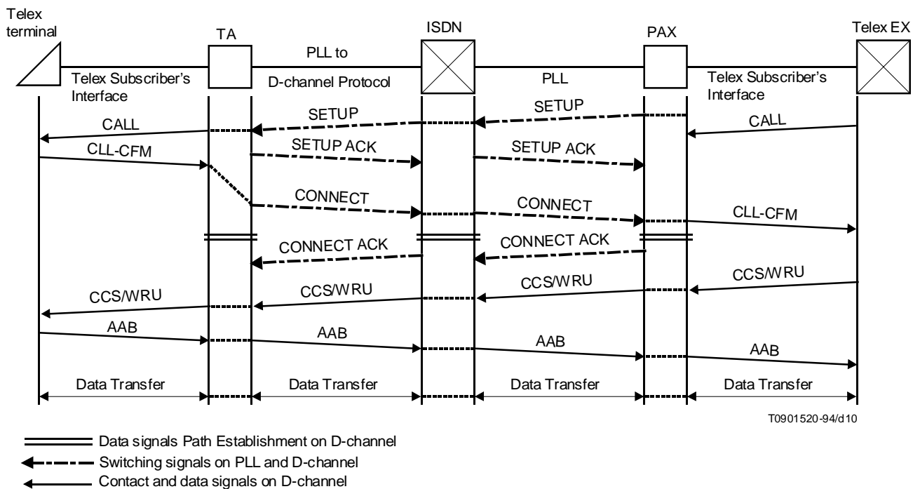
FIGURE 10/U.202 Call establishment sequence in the direction of a telex network to an ISDN (minimum integration model)
