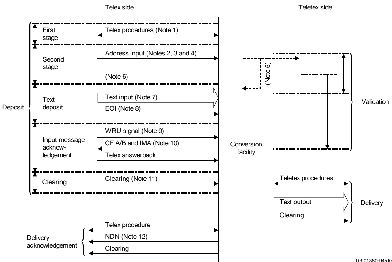
FIGURE 6/U.201 Interworking in the telex-to-Teletex direction using two-stage selection procedure (case of telex automatic emitting devices)
