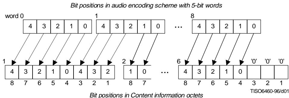
Figure 1 – Example of mapping between audio encoding and content information
