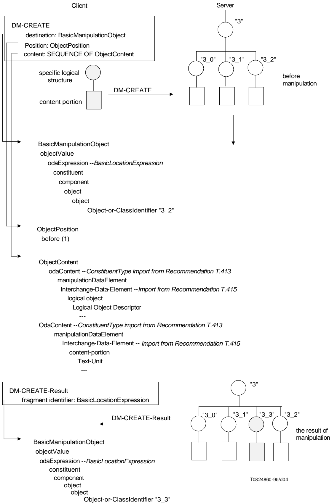
FIGURE A.1/T.191 DM-CREATE abstract service
