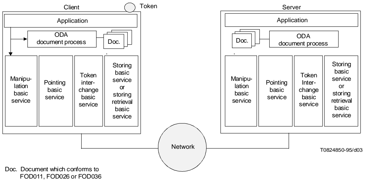
FIGURE 3/T.191 The summary of modules for joint synchronous editing (point-to-point)
