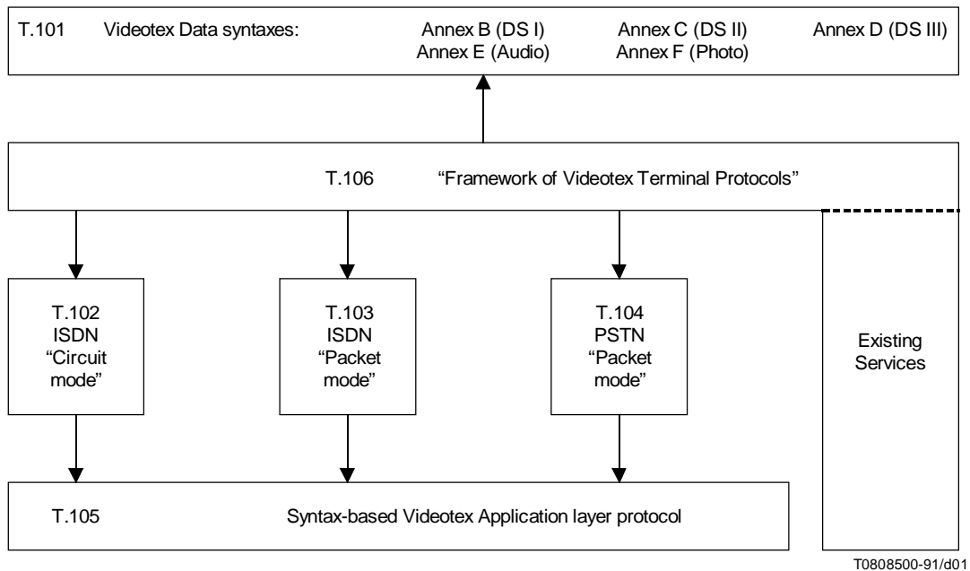
FIGURE 1/T.106 Relationships between videotex Recommendations
