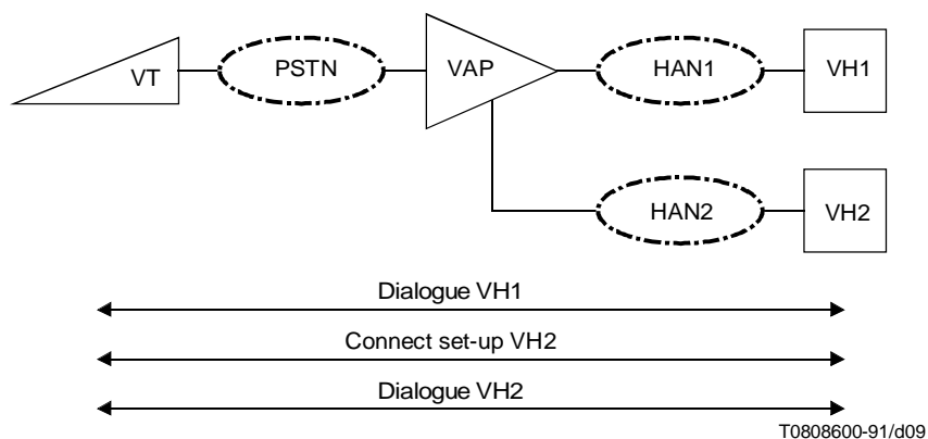
FIGURE A.8/T.104 Distributed hosts via two VC s initiated by the VT
