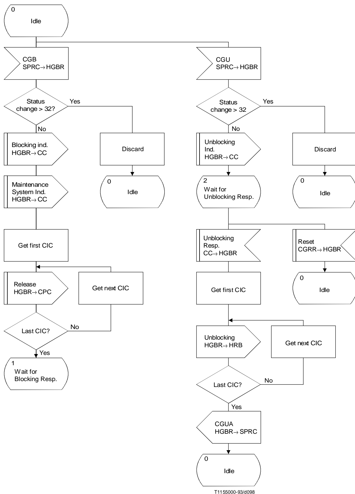
FIGURE H.34/Q.764 (sheet 1 of 2) Hardware Failure Oriented Circuit Group Blocking/Unblocking Reception (HGBR)
