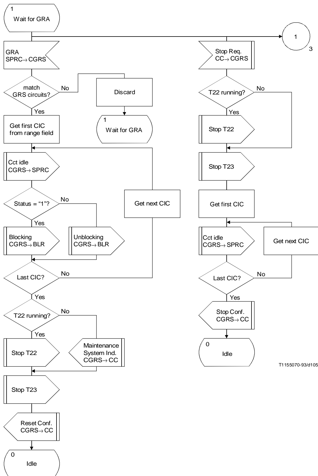
FIGURE H.37/Q.764 (sheet 2 of 3) Circuit Group Reset Sending (CGRS)
