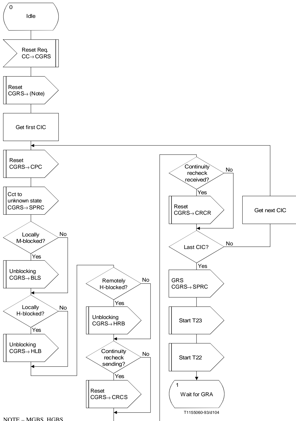
FIGURE H.37/Q.764 (sheet 1 of 3) Circuit Group Reset Sending (CGRS)
