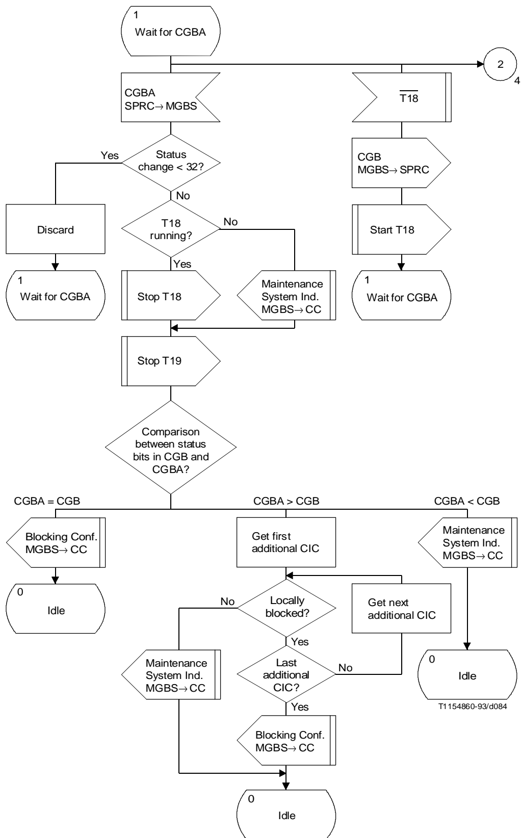
FIGURE H.29/Q.764 (sheet 3 of 6)
