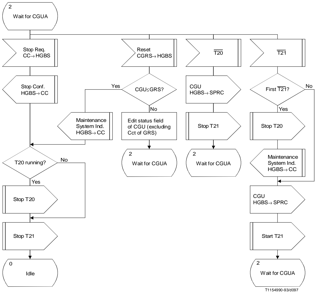
FIGURE H.33/Q.764 (sheet 6 of 6)
