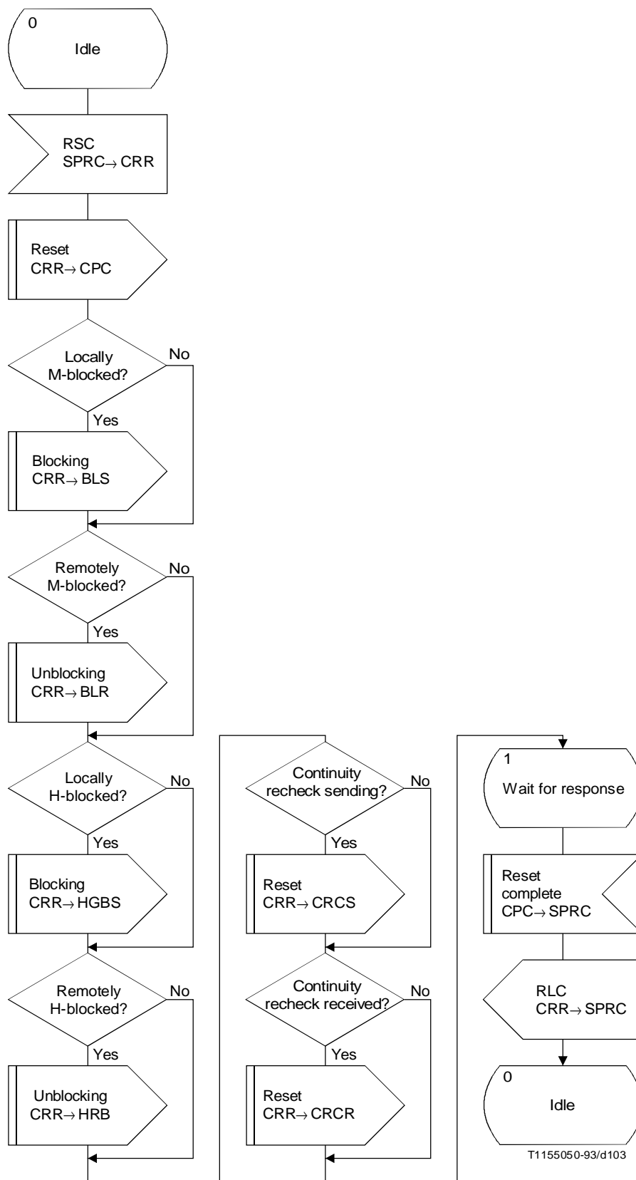
FIGURE H.36/Q.764 Circuit Reset Reception (CRR)
