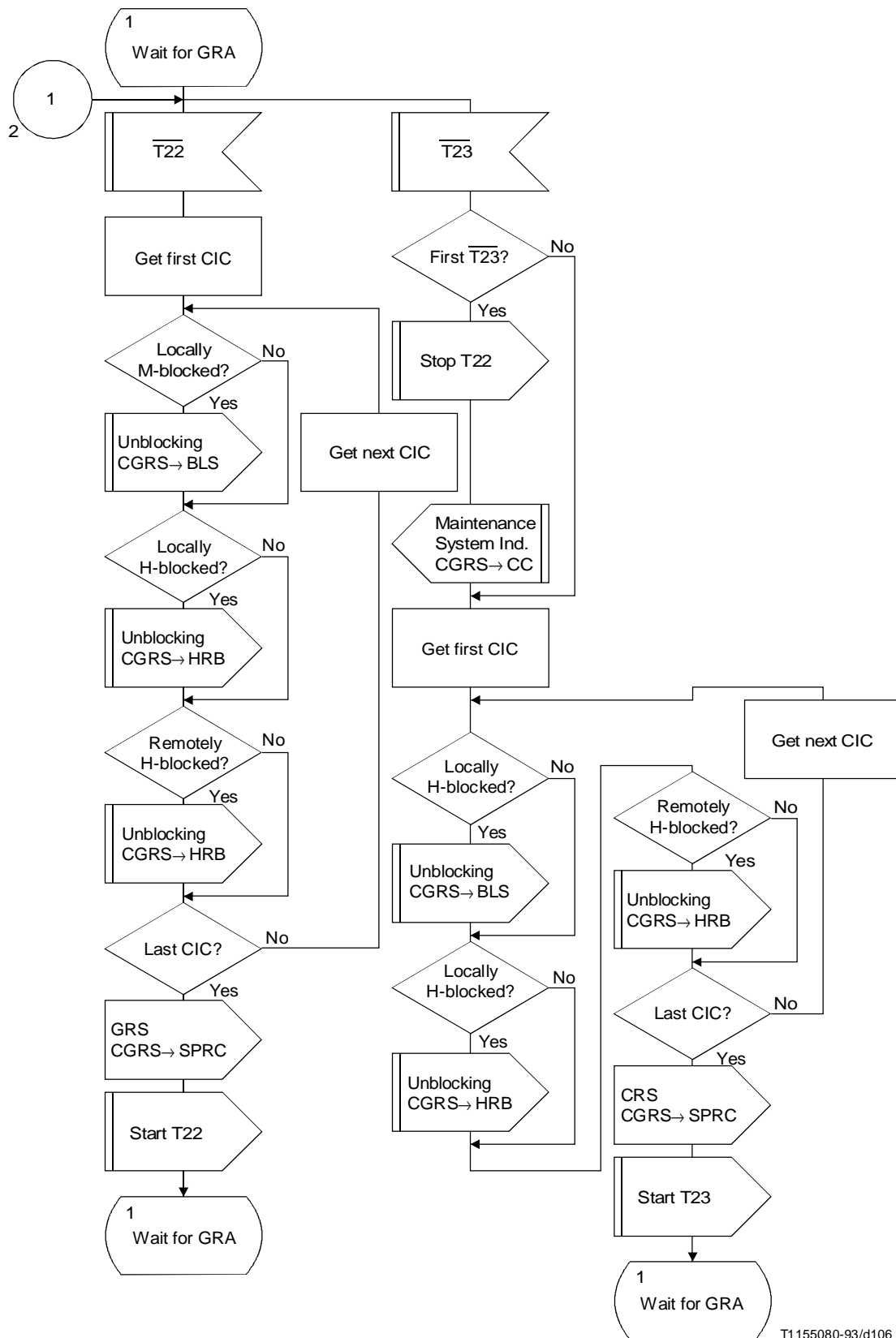
FIGURE H.37/Q.764 (sheet 3 of 3) Circuit Group Reset Sending (CGRS)
