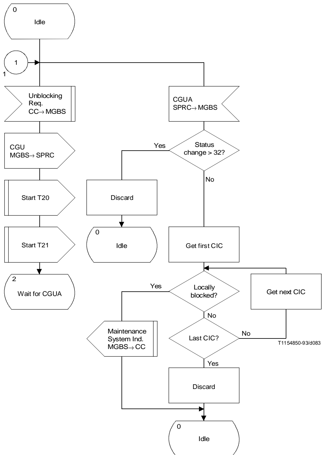
FIGURE H.29/Q.764 (sheet 2 of 6) Maintenance Oriented Circuit Group Blocking/Unblocking Sending (MGBS)
