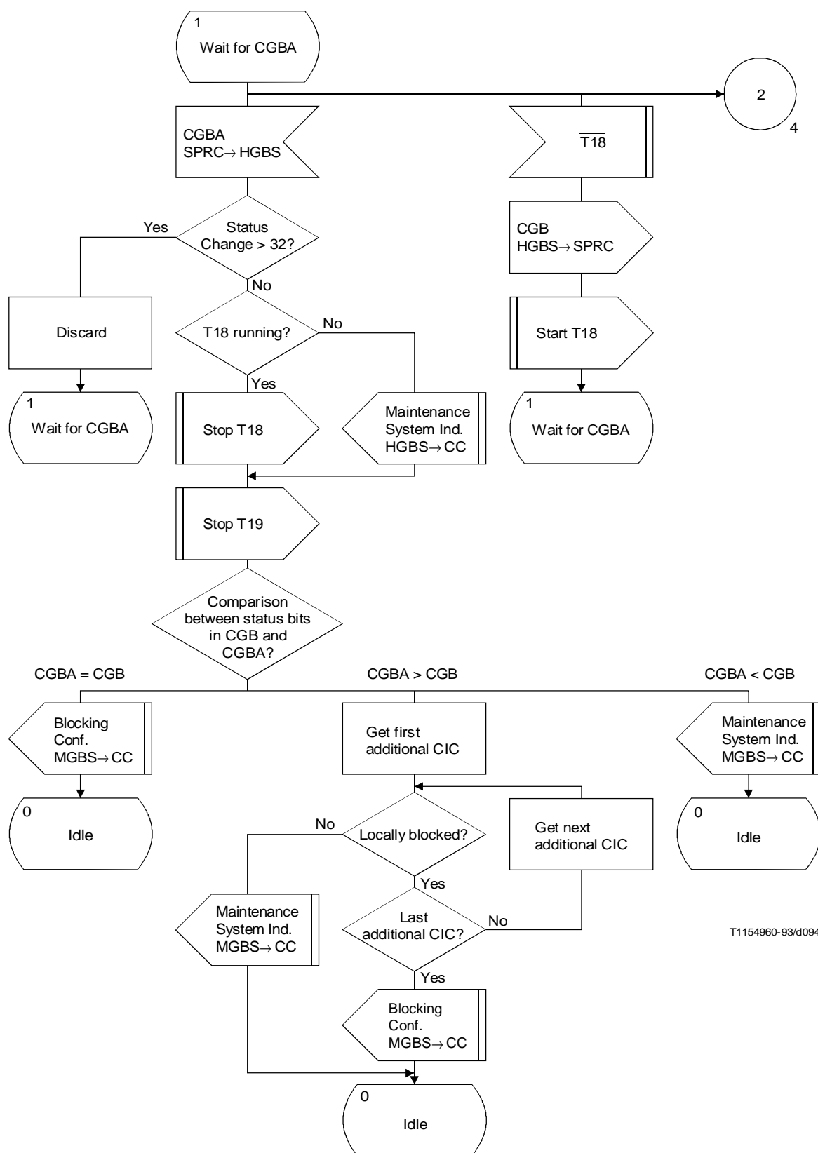
FIGURE H.33/Q.764 (sheet 3 of 6) Hardware Failure Oriented Circuit Group Blocking/Unblocking Sending (HGBS)
