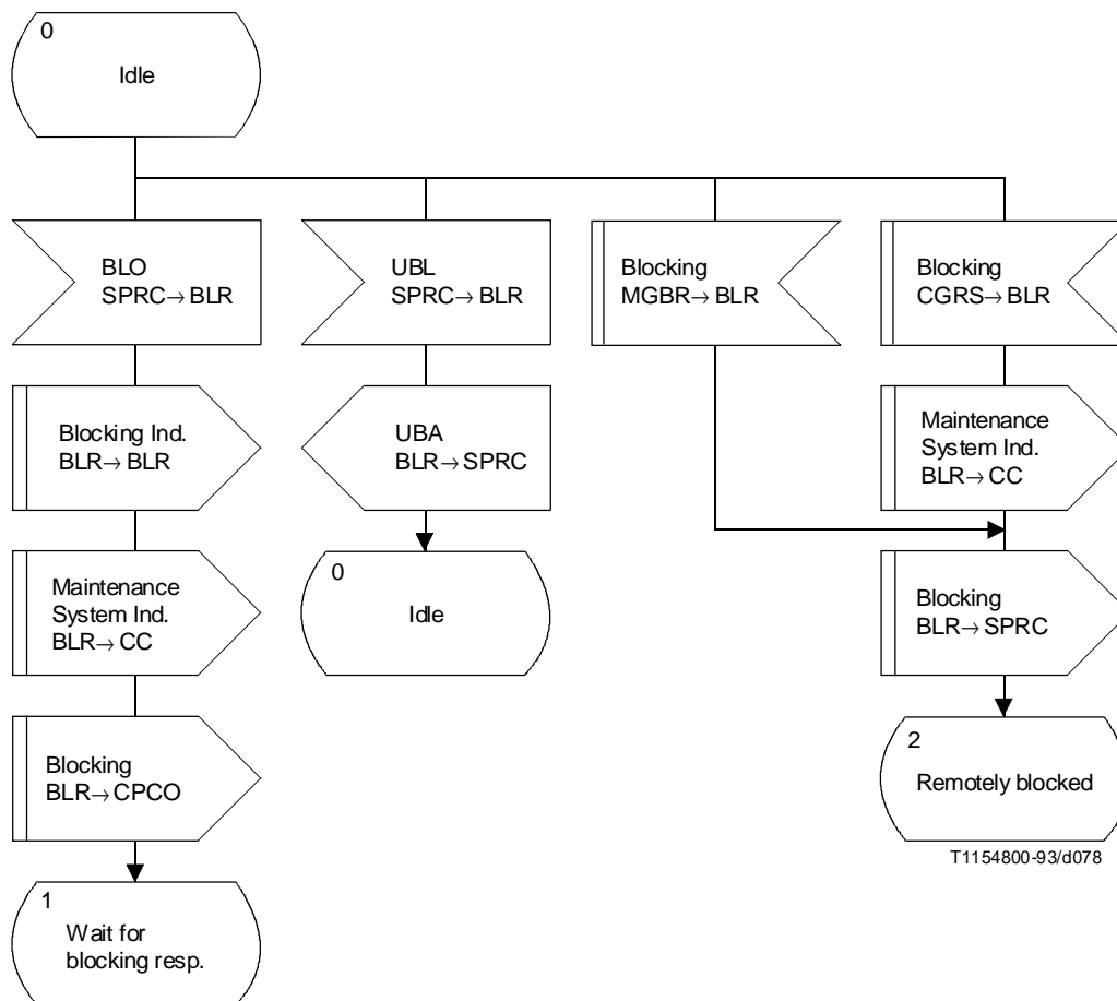
FIGURE H.28/Q.764 (sheet 1 of 4) Blocking/Unblocking Message Reception (BLR)
