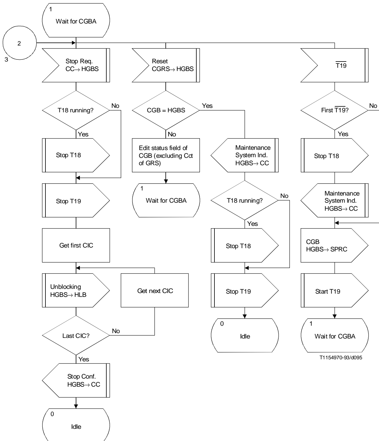
FIGURE H.33/Q.764 (sheet 4 of 6)
