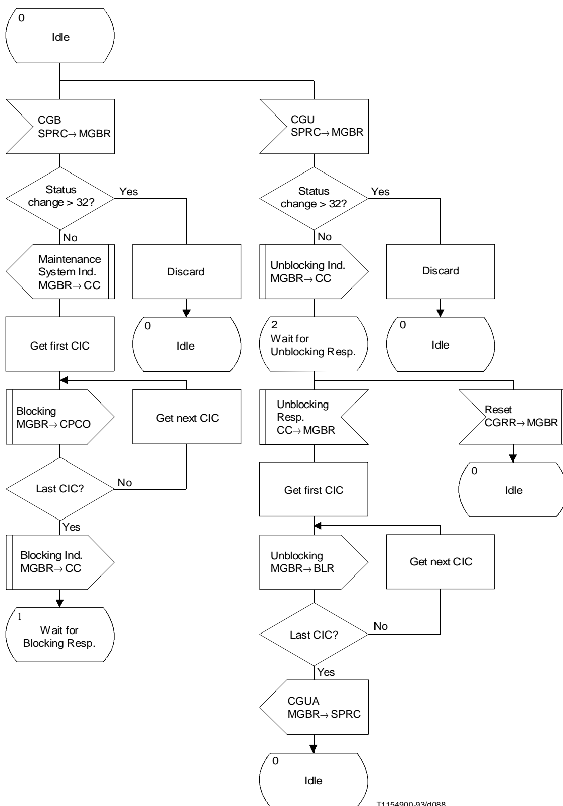
FIGURE H.30/Q.764 (sheet 1 of 2) Maintenance Oriented Circuit Group Blocking/Unblocking Reception
