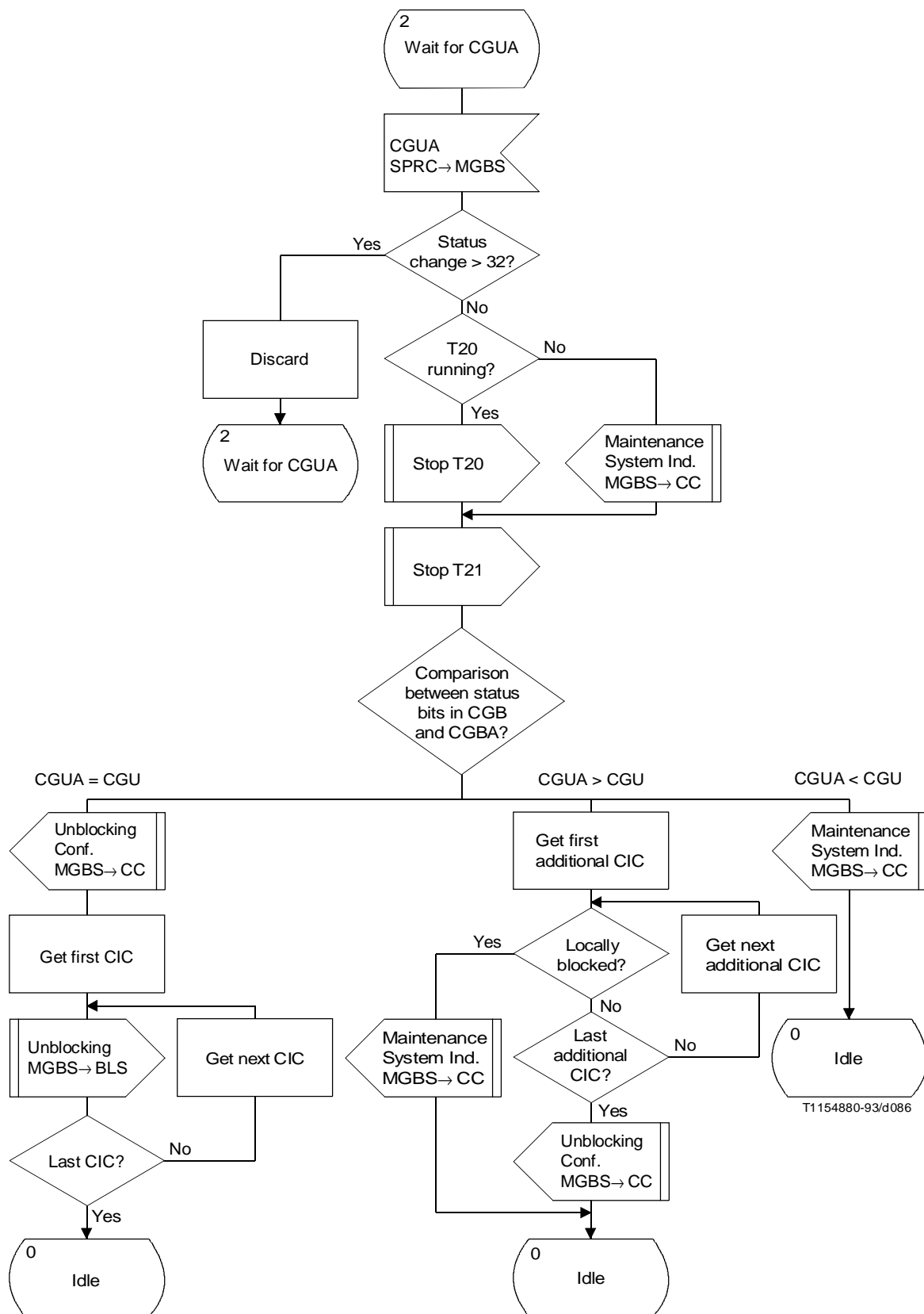
FIGURE H.29/Q.764 (sheet 5 of 6) Maintenance Oriented Circuit Group Blocking/Unblocking Sending (MGBS)
