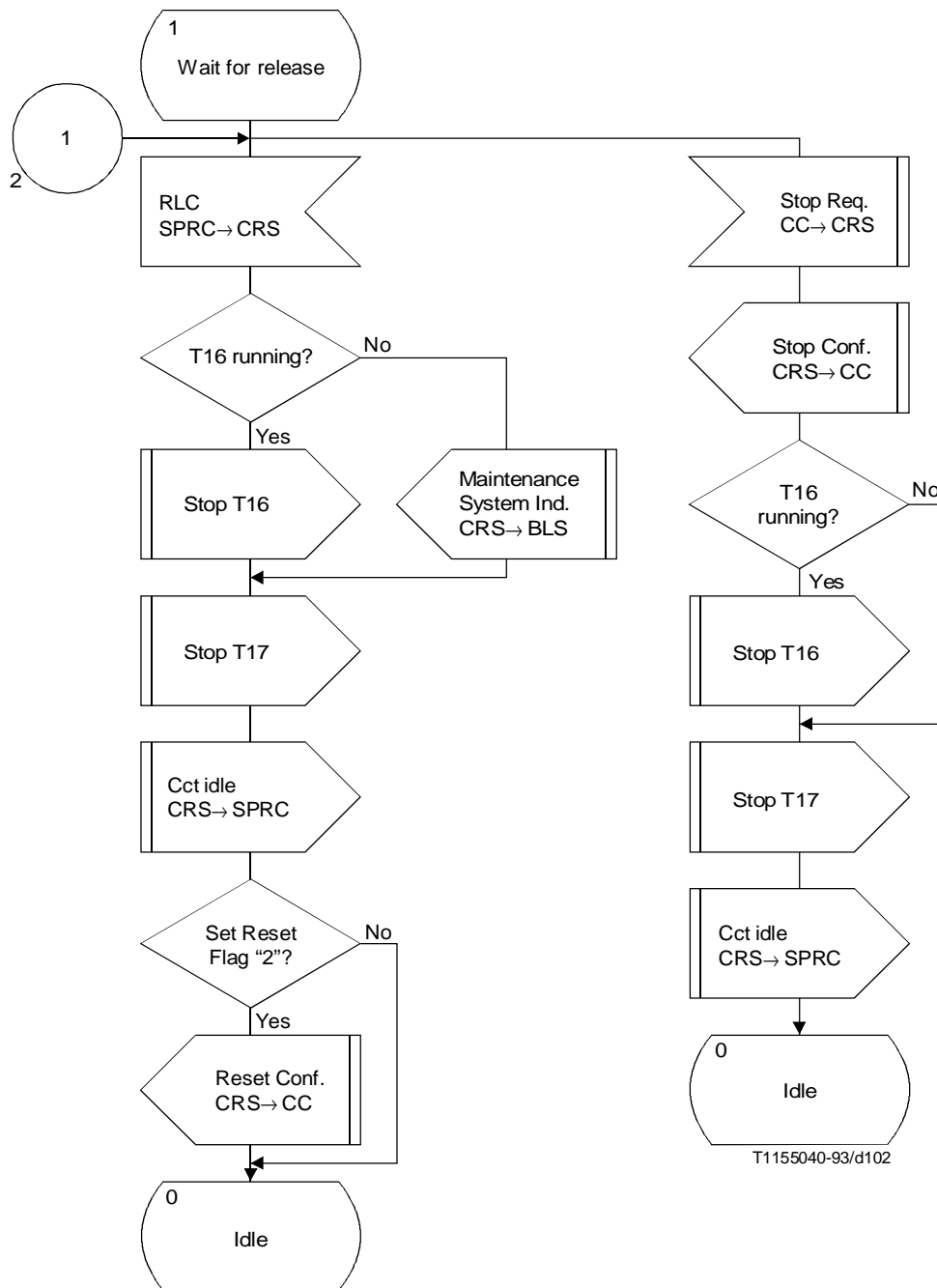
FIGURE H.35/Q.764 (sheet 3 of 3) Circuit Reset Sending (CRS)
