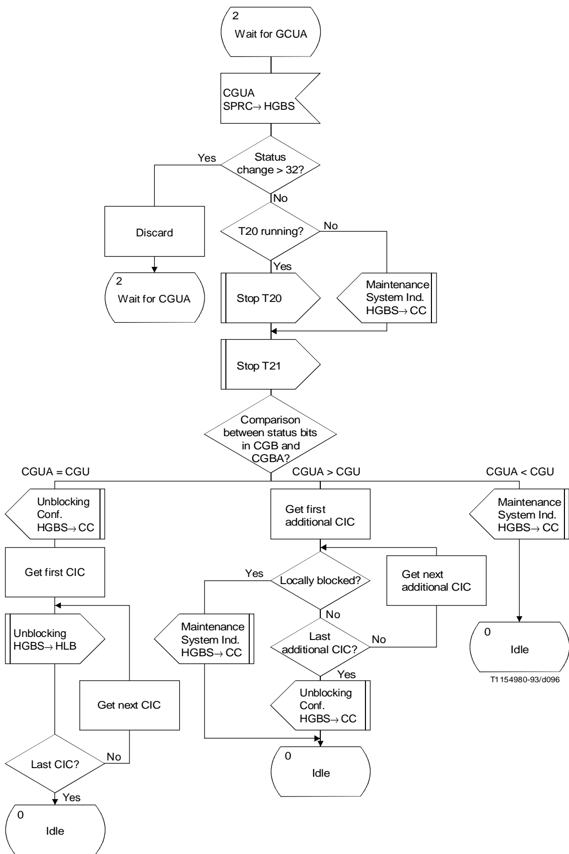
FIGURE H.33/Q.764 (sheet 5 of 6)
