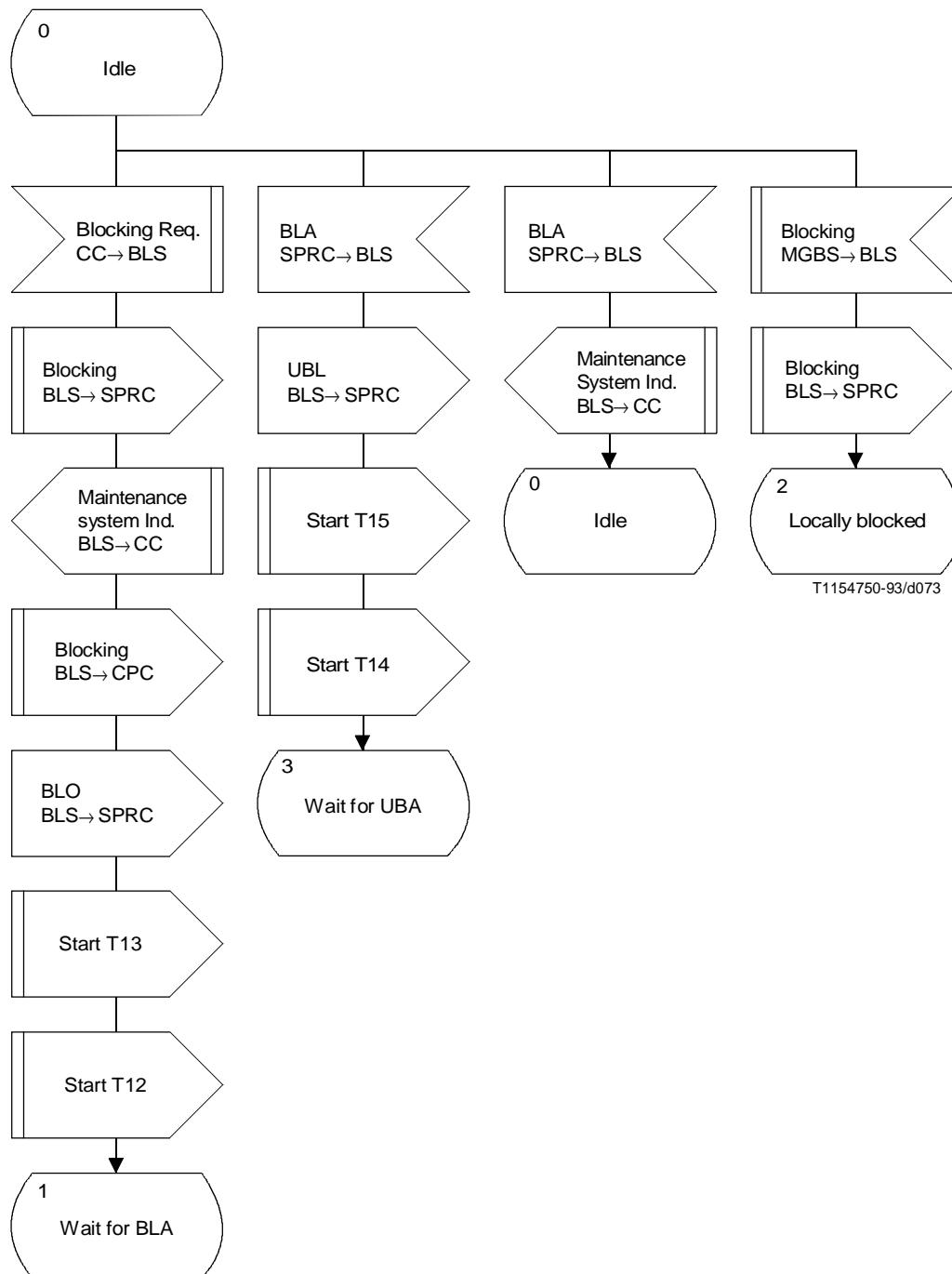
FIGURE H.27/Q.764 (sheet 1 of 5) Blocking/Unblocking Message Sending (BLS)
