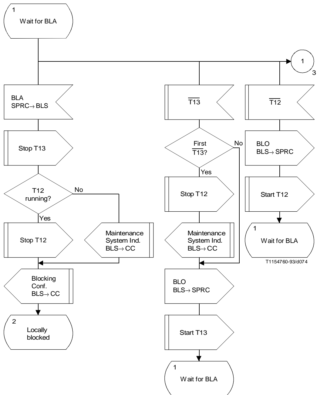
FIGURE H.27/Q.764 (sheet 2 of 5) Blocking/Unblocking Message Sending (BLS)
