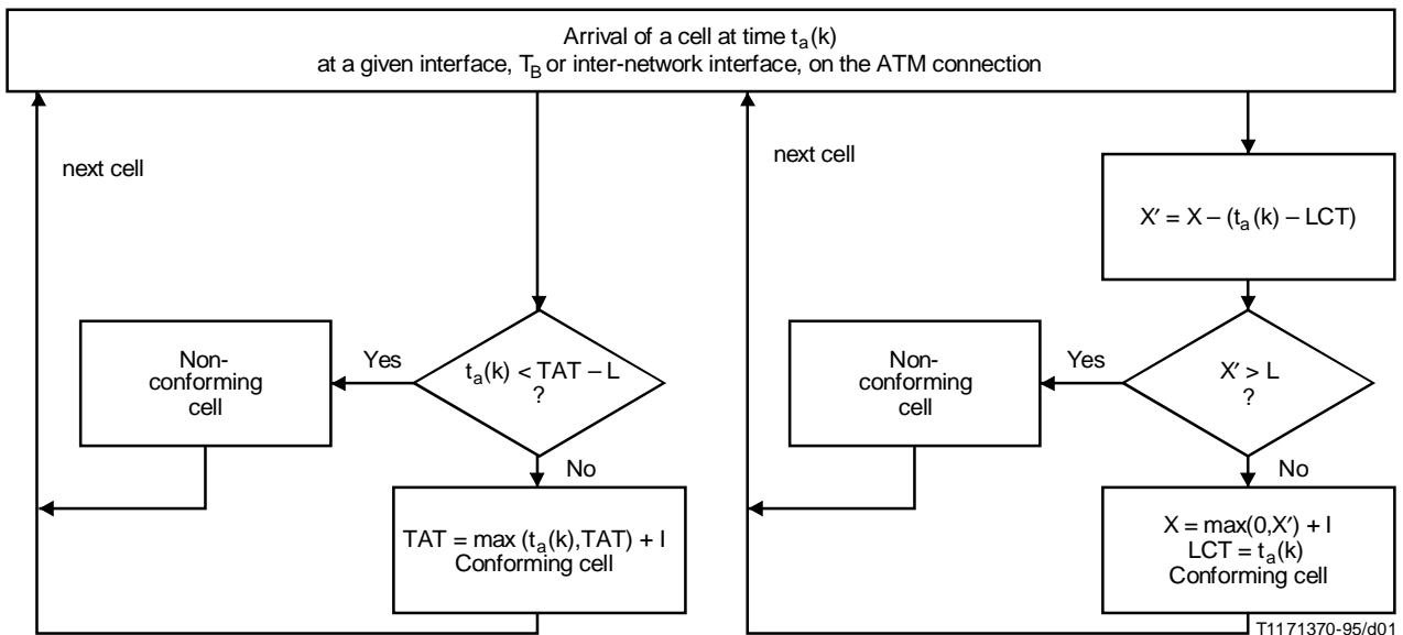
Virtual scheduling algorithm
