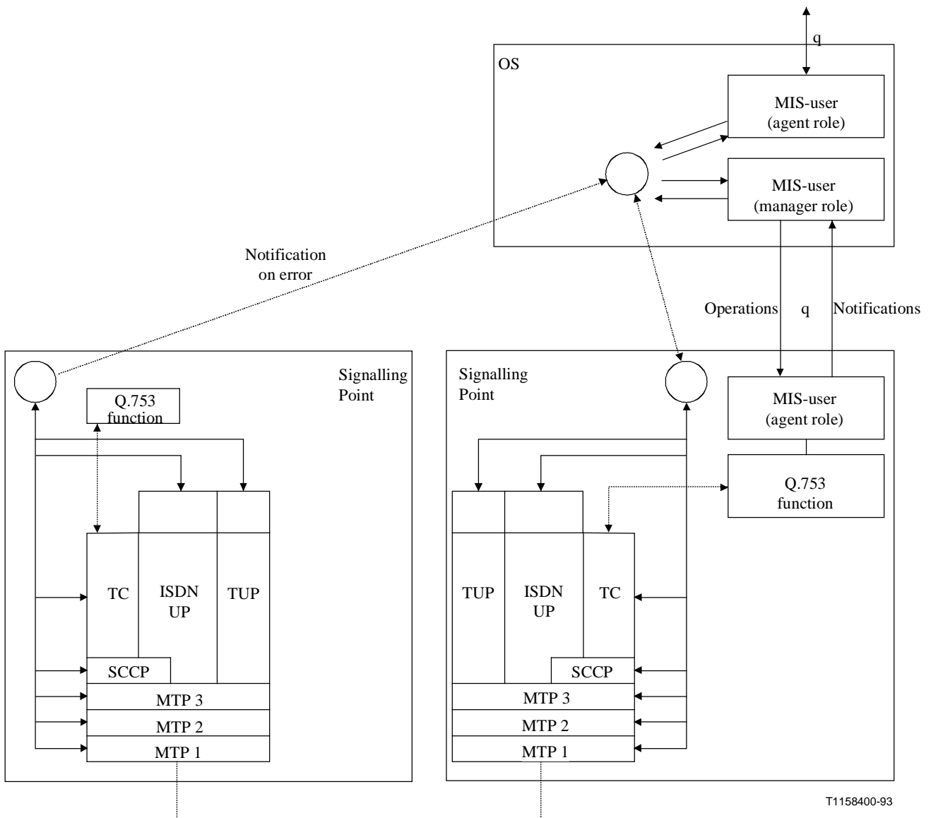
Figure 4/Q.750 – Managed objects using internal communication
