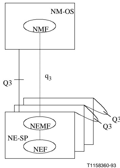
Figure 2/Q.750 (sheet 1 of 3) – Example physical realization for SS No. 7 management
