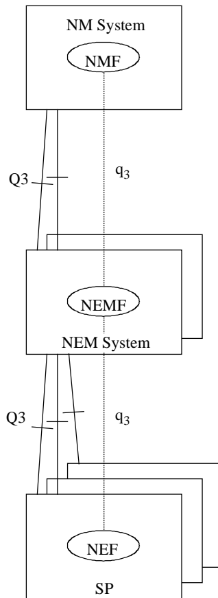
Figure 2/Q.750 (sheet 2 of 3) – Example physical realization for SS No. 7 management
