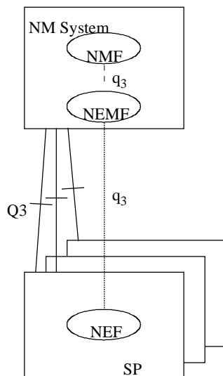
Figure 2/Q.750 (sheet 3 of 3) – Example physical realization for SS No. 7 management
