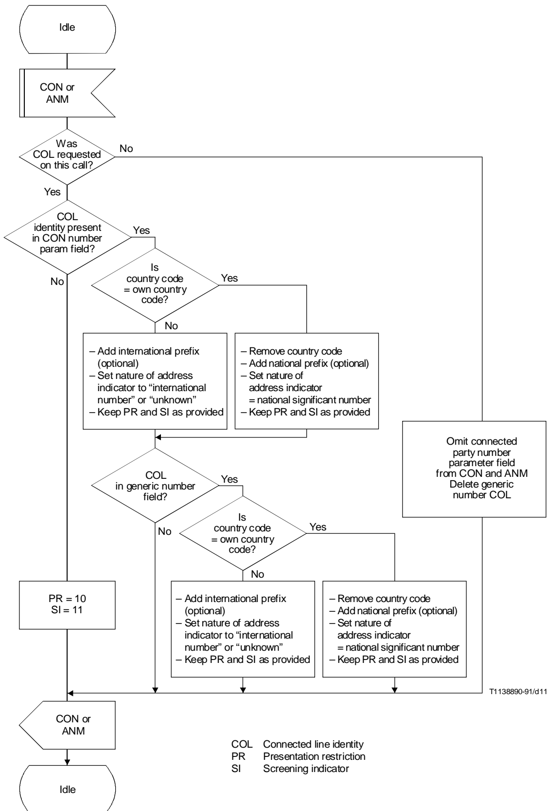
FIGURE 5-7/Q.731 Nodal signalling functions for COLP and COLR Outgoing international gateway exchange
