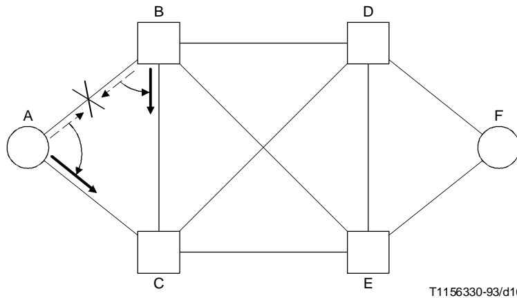
FIGURE A.15/Q.705 Failure of link AB
