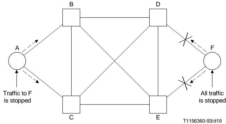
FIGURE A.18/Q.705 Failure of links DF and EF
