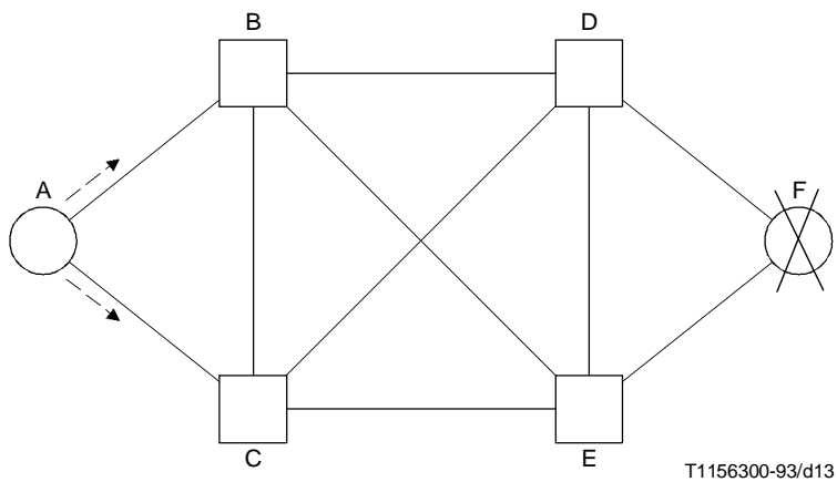
FIGURE A.12/Q.705 Failure of signalling point F
