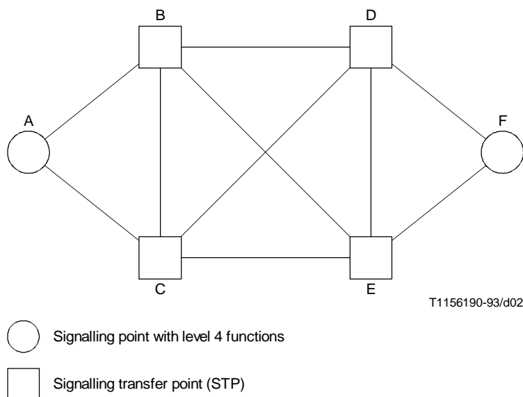
FIGURE A.1/Q.705 Basic mesh network
