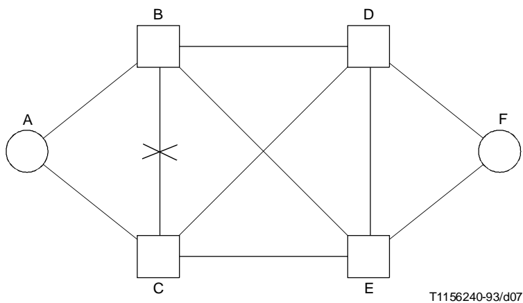
FIGURE A.6/Q.705 Failure of link BC
