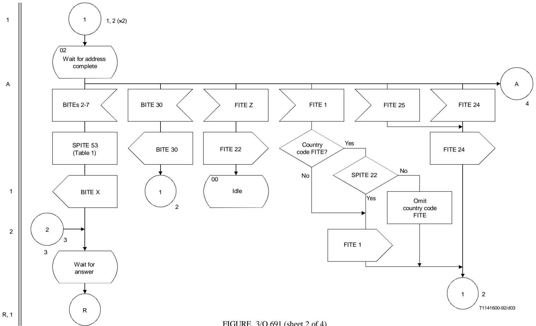
FIGURE 3/Q.691 (sheet 2 of 4) Interworking of Signalling System No. 7 (ISUP) to No. 6
