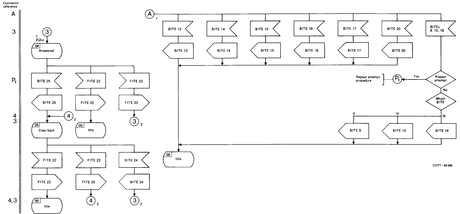
FIGURE 3/Q.663 (Sheet 2 of 2) Interworking of Signalling System No. 7 (TUP) to No. 6
