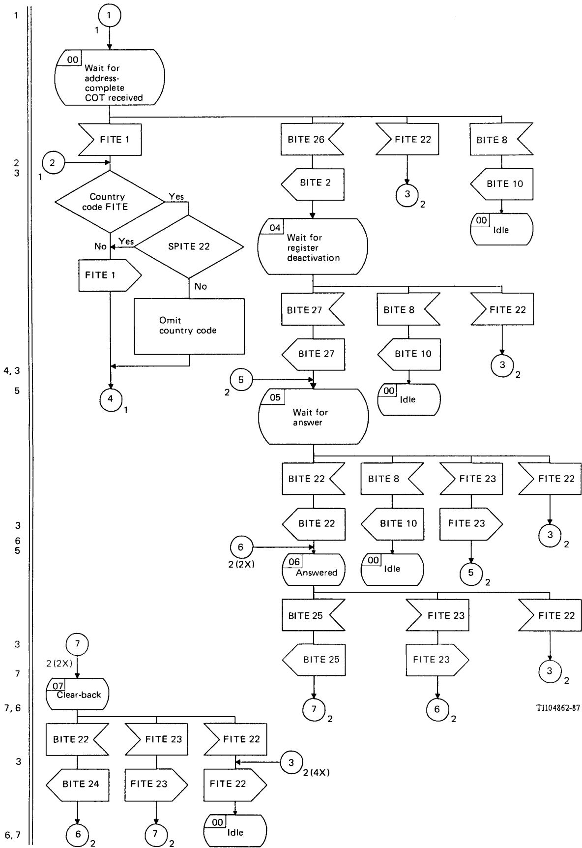
FIGURE 3/Q.662 (Sheet 2 of 2) Interworking of Signalling System No. 7 (TUP) to No. 5
