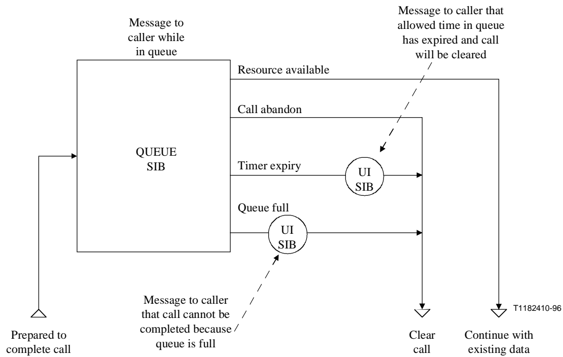
Figure 4-13/Q.86.4 – Queuing of calls/recorded announcements
