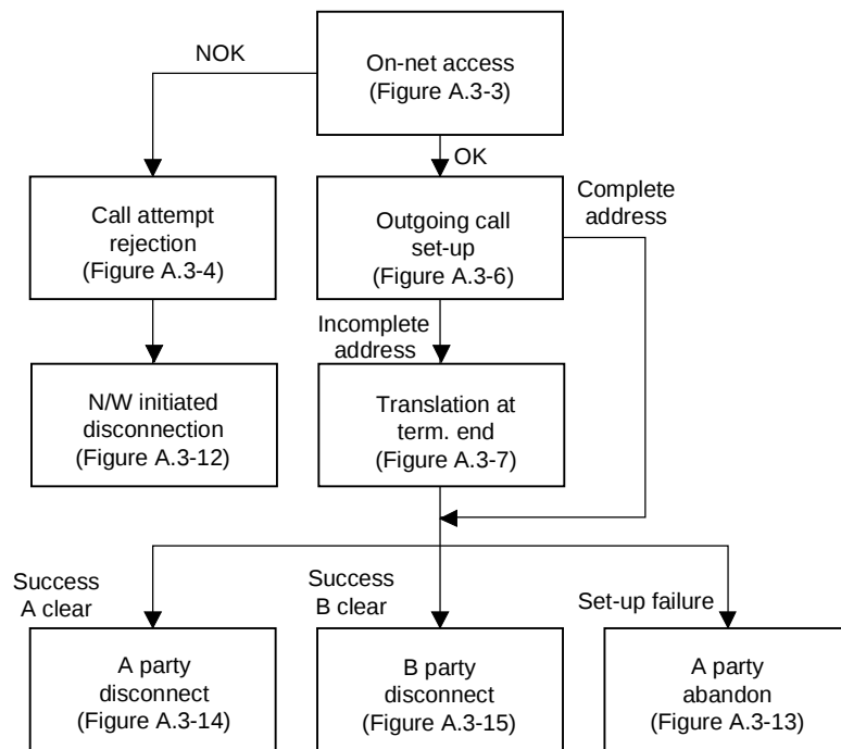
Figure A.3-1/Q.85.6 – Sequencing of diagrams for direct and switched (on-net) access
