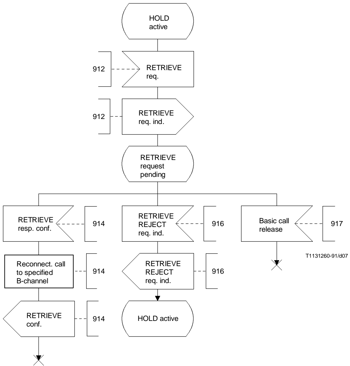
FIGURE 2-5/Q.83 (sheet 3 of 4)
