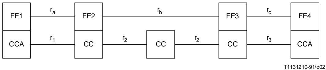
FIGURE 2-2/Q.83 Relationship to basic service
