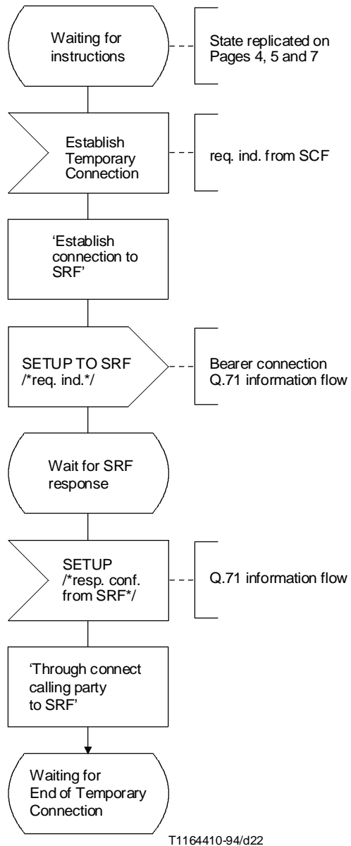
FIGURE 4-1/Q.76 (sheet 2 of 7)
