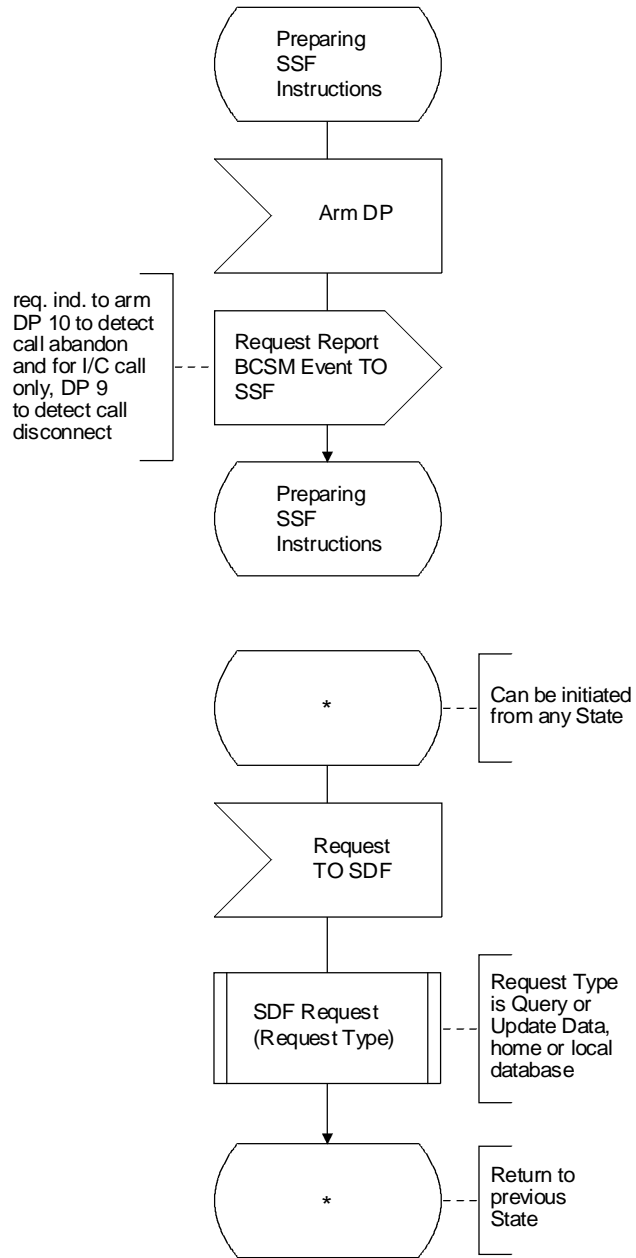
FIGURE 4-2/Q.76 (sheet 2 of 8)
