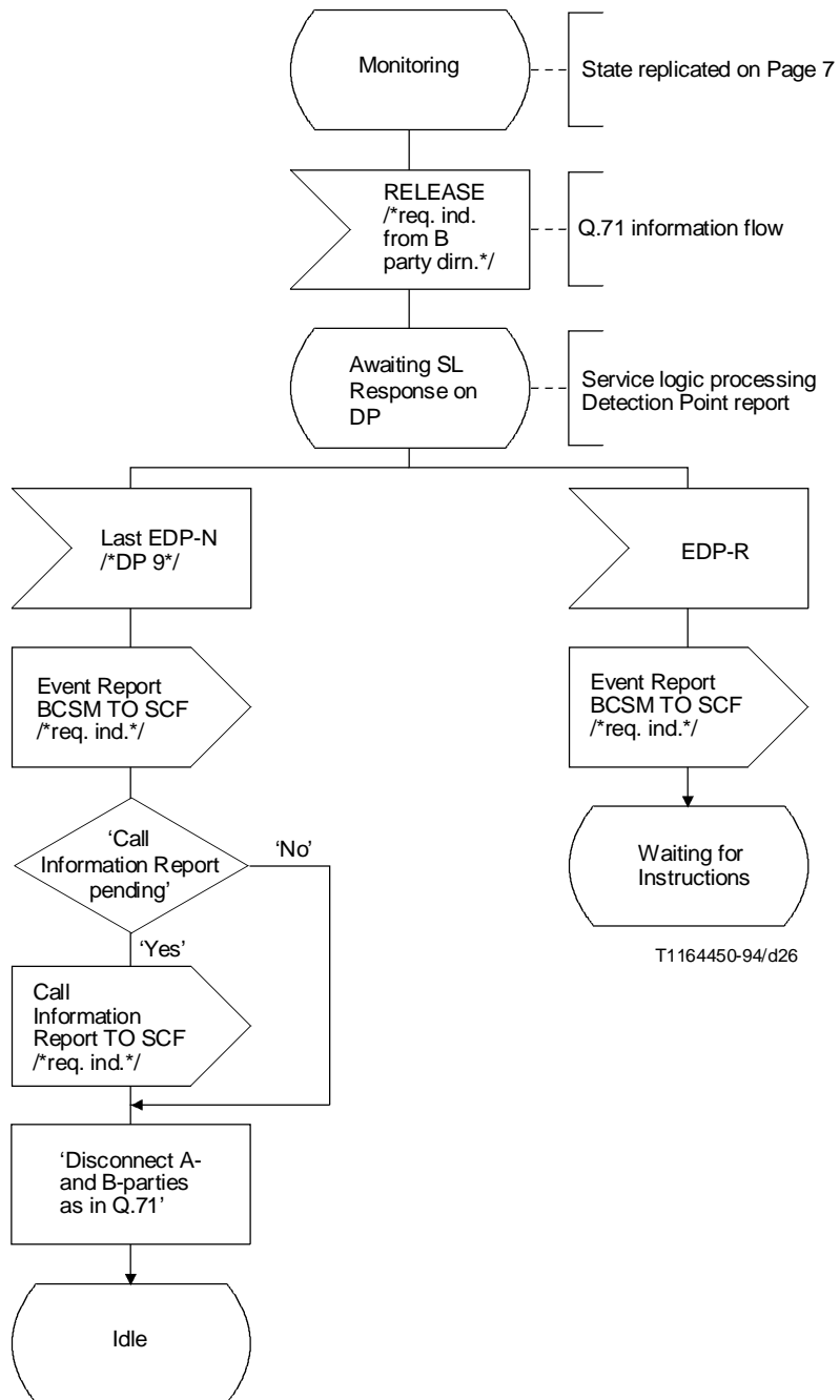
FIGURE 4-1/Q.76 (sheet 6 of 7) SDL diagram for SSF/CCF
