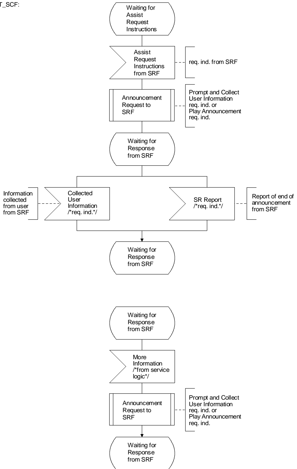
FIGURE 4-2/Q.76 (sheet 4 of 8) SDL diagram for SCF
