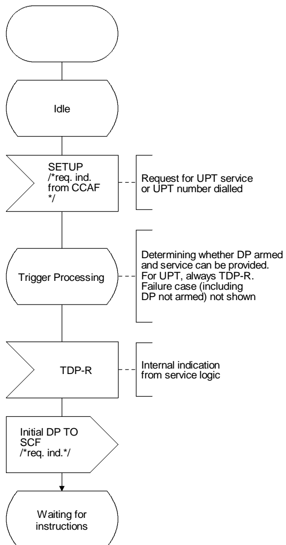
FIGURE 4-1/Q.76 (sheet 1 of 7) SDL diagram for SSF/CCF
