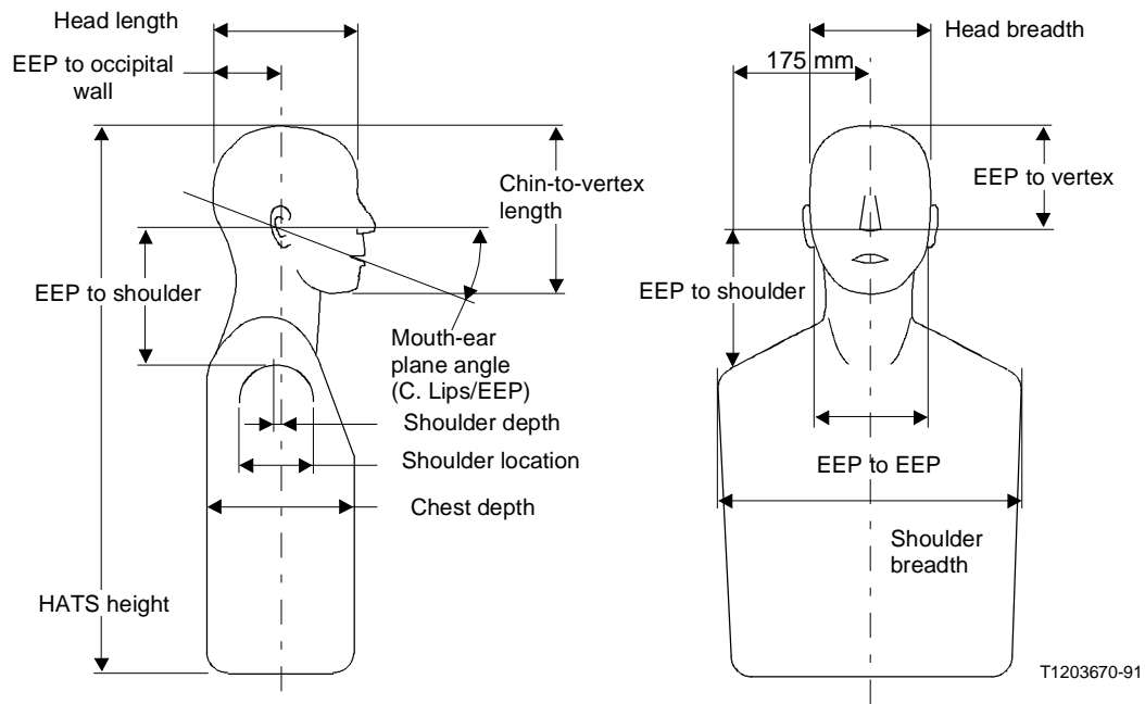
FIGURE 3/P.58 Illustration of HATS dimensions
