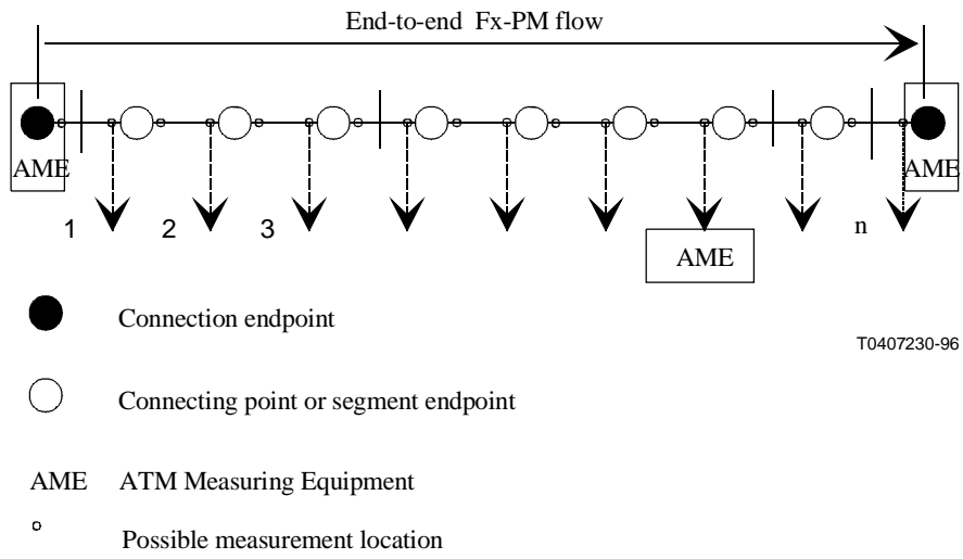
Figure I.6/O.191 – Combination of in-service and out-of-service modes
