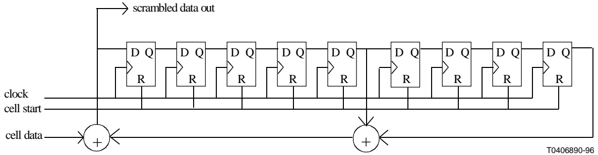
Figure C.1/O.191 – Scrambler circuit using polynomial x^9 + x^5 + 1
