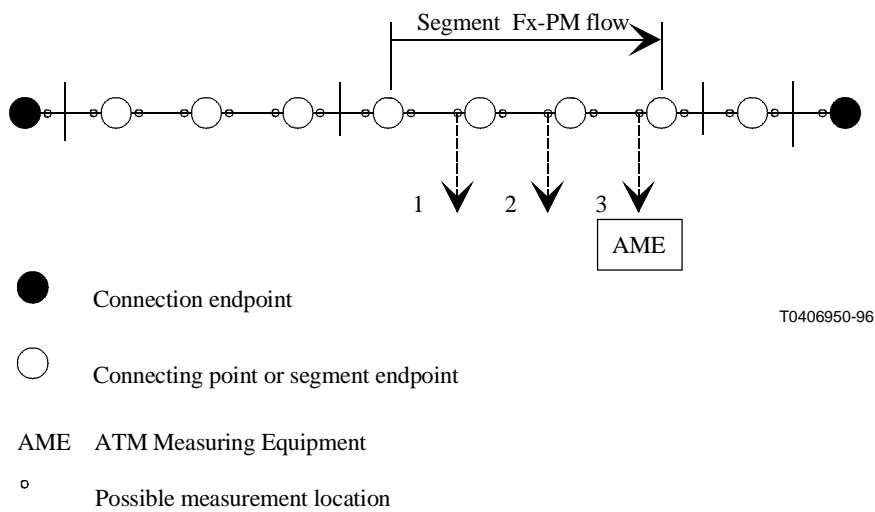
Figure I.5/O.191 – In-service segment test
