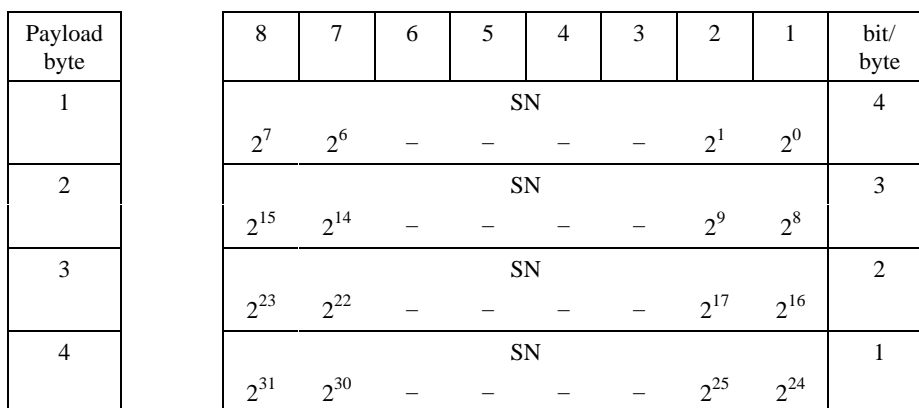
Figure 7-2/O.191 – Details of the SN field
