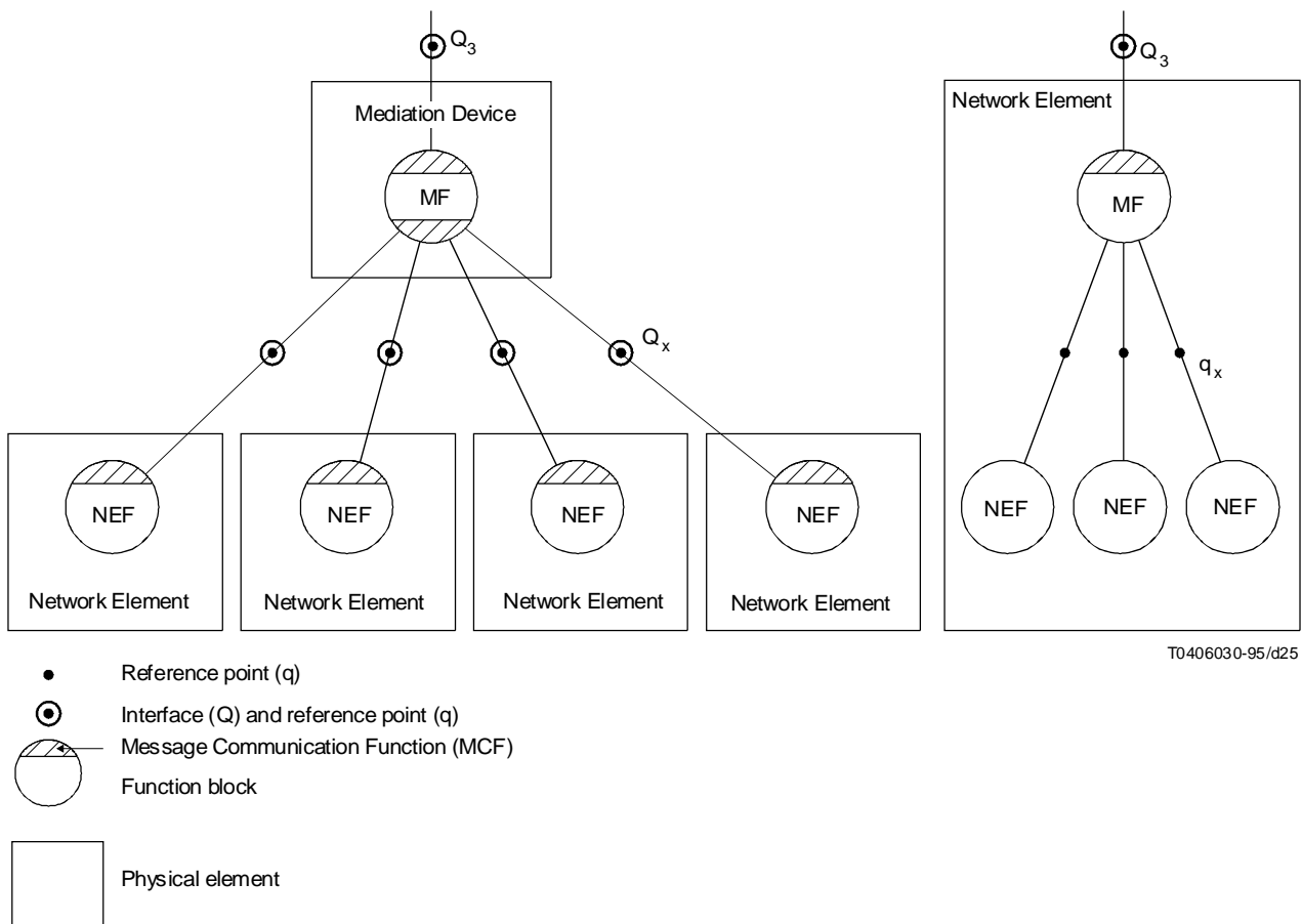
FIGURE 25/M.3010 Example of the use of Mediation
