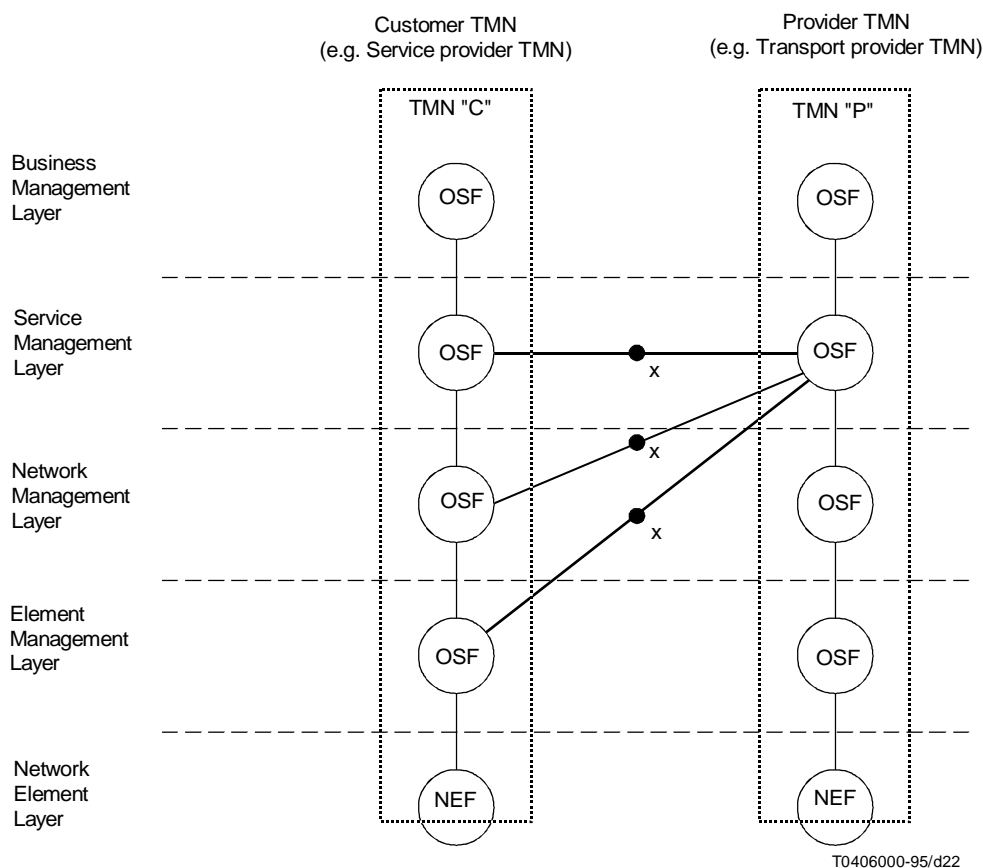
FIGURE 22/M.3010 Examples of inter-TMN functional connectivity
