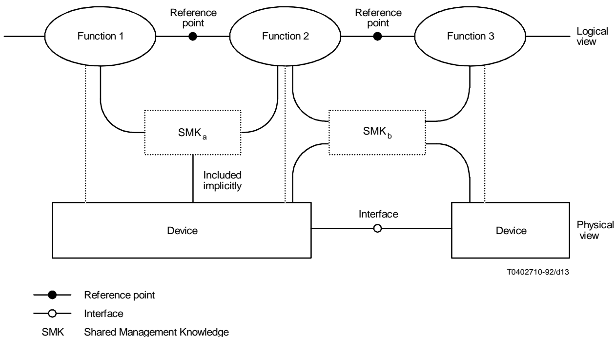
FIGURE 13/M.3010 Independence of SMKs from the physical implementation
