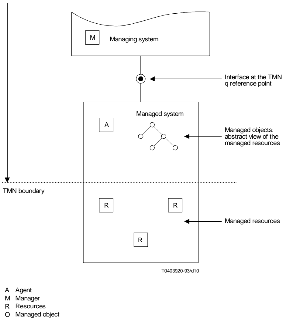
FIGURE 10/M.3010 Relationship between objects and managed resources for the case of an NE
