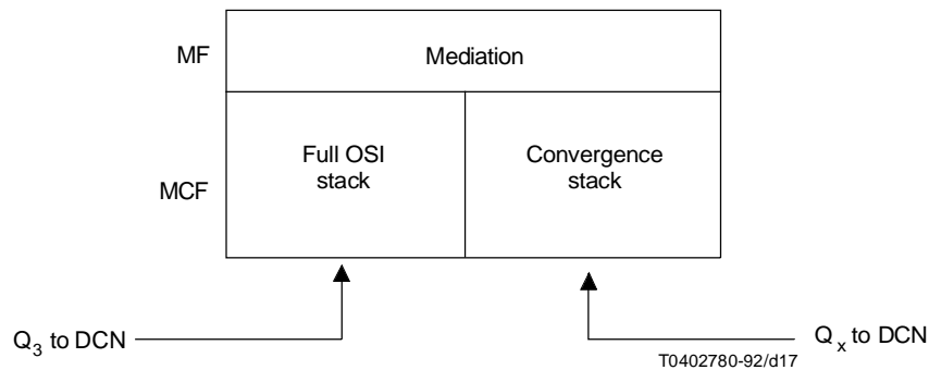
FIGURE 17/M.3010 Example of higher layer interworking
