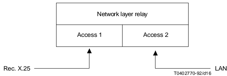
FIGURE 16/M.3010 Communication relay implemented via two DCNs
