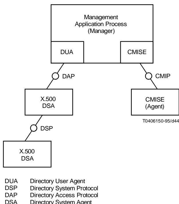
FIGURE V.2/M.3010 Joint use of Directory (DAP) and CMISE (CMIP)
