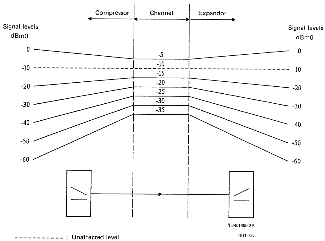
FIGURE A-1/M.590 Compandor characteristic
