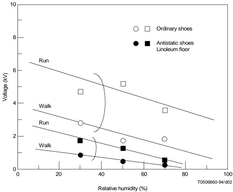
FIGURE I.2/K.32 Maximum values of electrostatic voltage to which operators may be charged in telecommunications central office (Source: COM 5-D.35, 1990, NTT)
