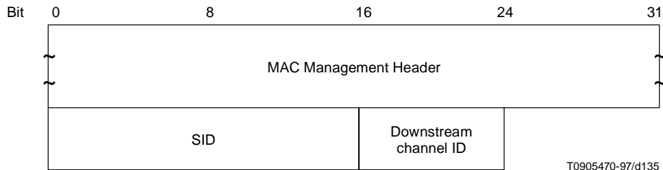
Figure C.6-22/J.112 – RNG-REQ message
