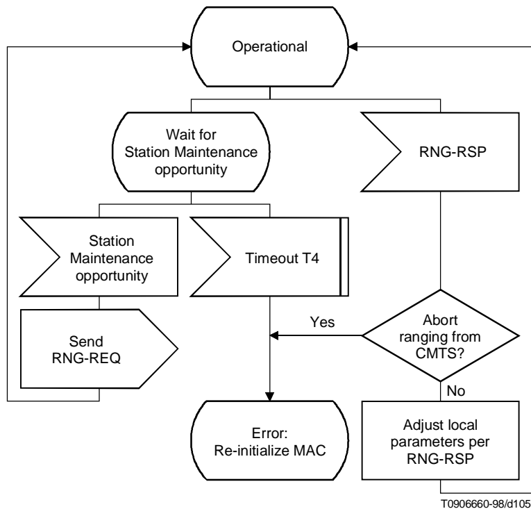
Figure B.7-13/J.112 – Periodic Ranging – CM View
