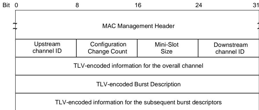
Figure C.6-17/J.112 – UCD message
