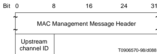
Figure B.6-30/J.112 – Upstream Channel Change Response
