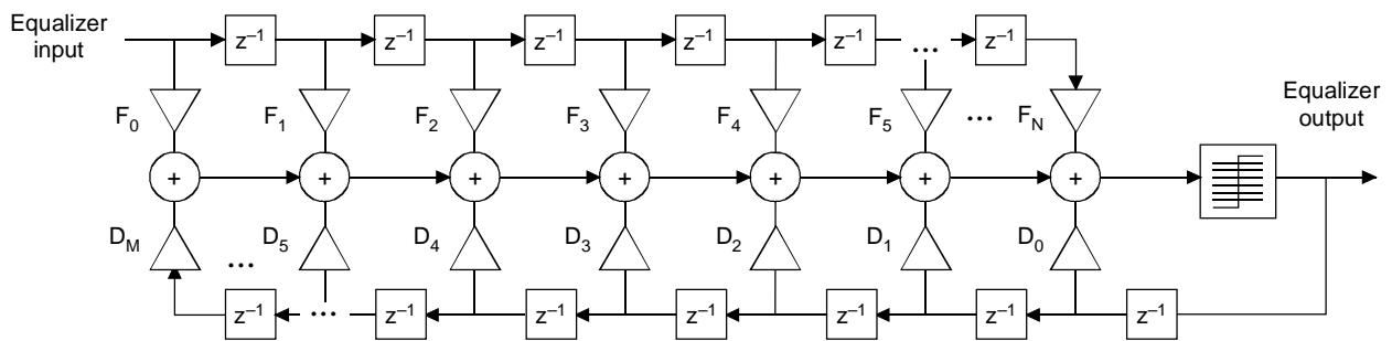
Figure C.6-25/J.112 – Equalizer tap location
