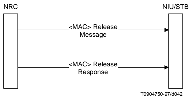
Figure A.33/J.112 – Connection release signalling
