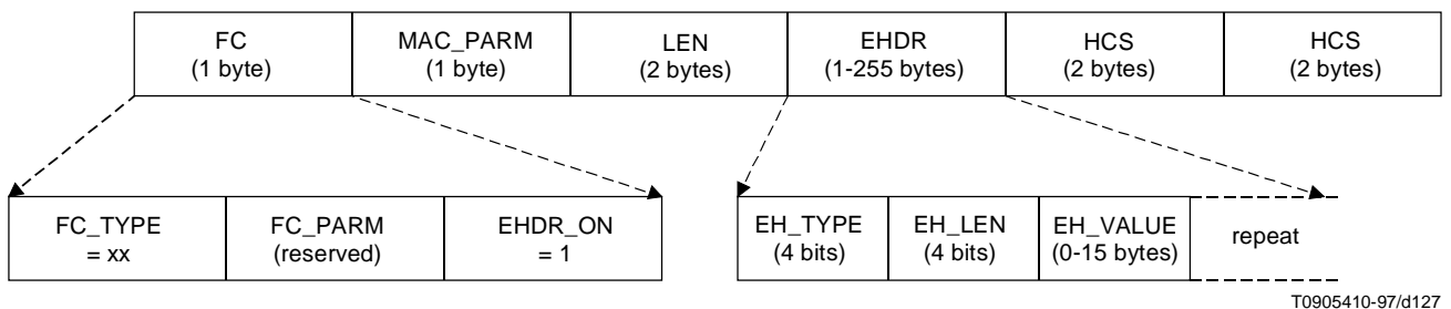
Figure C.6-14/J.112 – Extended MAC Header
