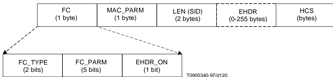
Figure C.6-7/J.112 – MAC Header format
