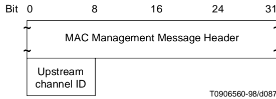
Figure B.6-29/J.112 – Upstream Channel Change Request
