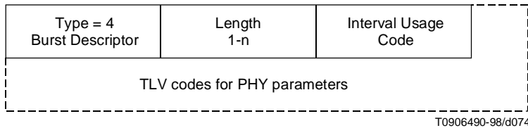
Figure B.6-16/J.112 – Top-level encoding for a Burst Descriptor
