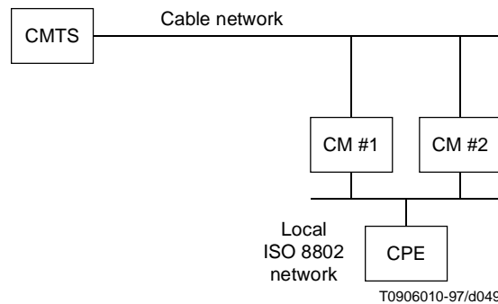
Figure B.3-3/J.112 – Example condition for network loops
