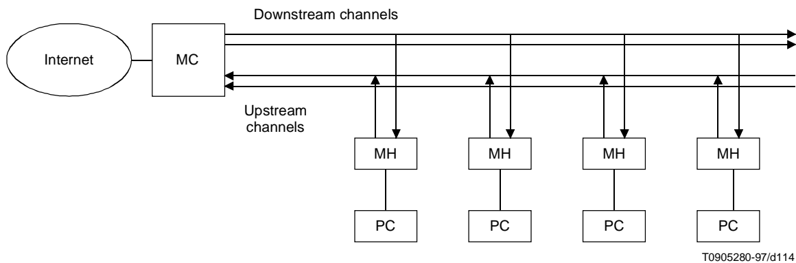
Figure C.6-1/J.112 – Network construction
