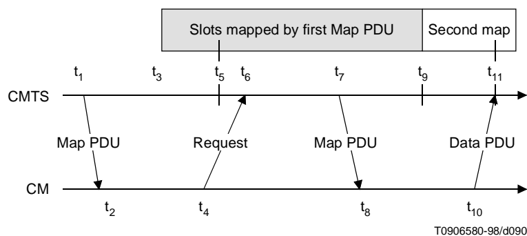
Figure B.6-32/J.112 – Protocol example
