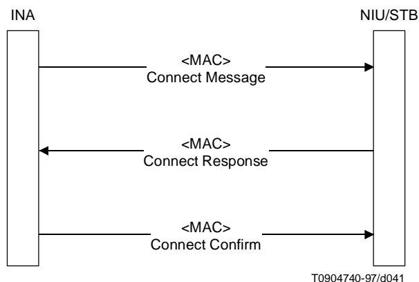
Figure A.32/J.112 – Connection signalling
