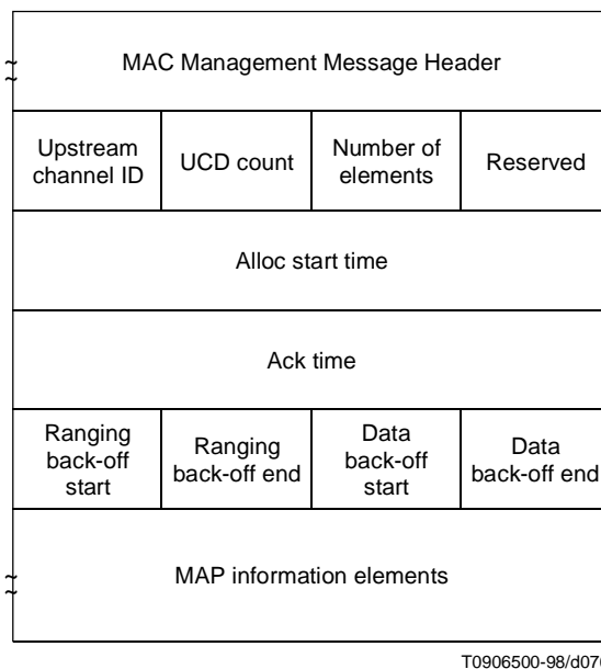
Figure B.6-18/J.112 – MAP format
