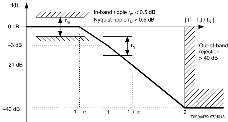
Figure A.14/J.112 – QPSK upstream transmitter Power Spectrum
