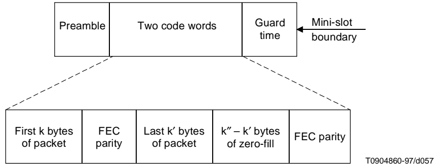
Figure B.4-7/J.112 – Example frame structures with flexible burst length mode
