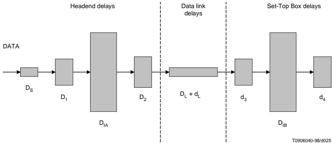
Figure A.24/J.112 – System model for timing analysis
