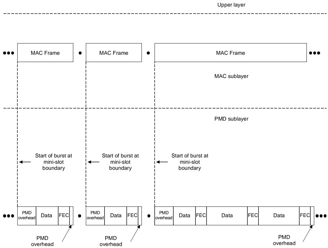
Figure B.6-2/J.112 – Upstream MAC/PMD convergence
