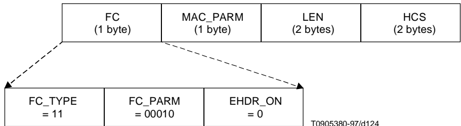
Figure C.6-11/J.112 – MAC request header
