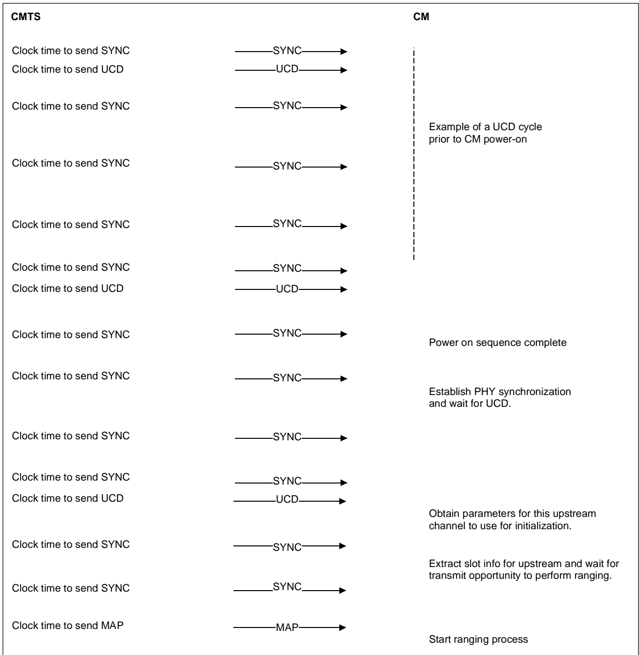
Figure B.7-4/J.112 – Message flows during scanning and Upstream parameter acquisition
