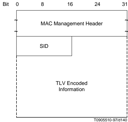
Figure C.6-27/J.112 – REG-REQ message
