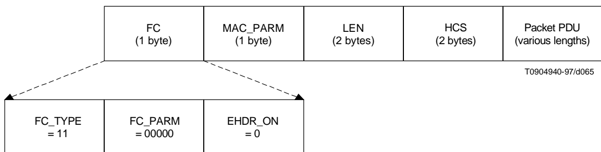
Figure B.6-7/J.112 – Timing MAC Header
