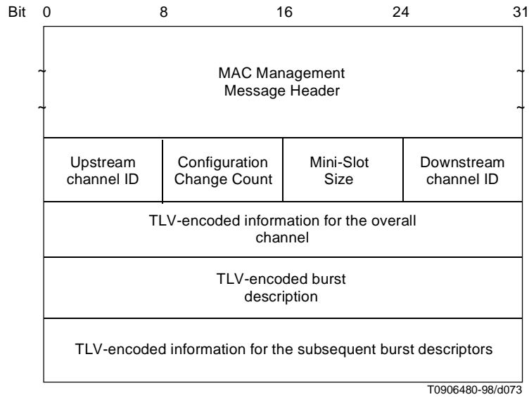
Figure B.6-15/J.112 – Upstream channel descriptor
