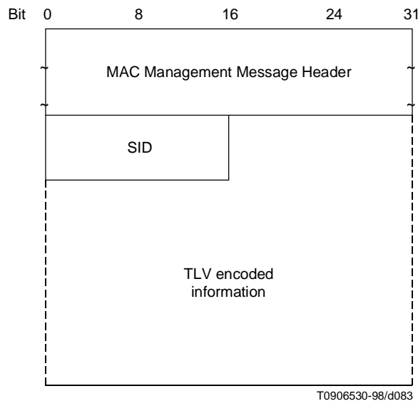
Figure B.6-25/J.112 – Registration Request
