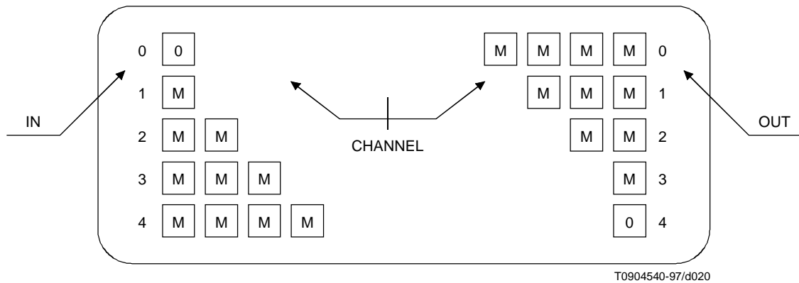
Figure A.19/J.112 – Interleaver and de-interleaver structures
