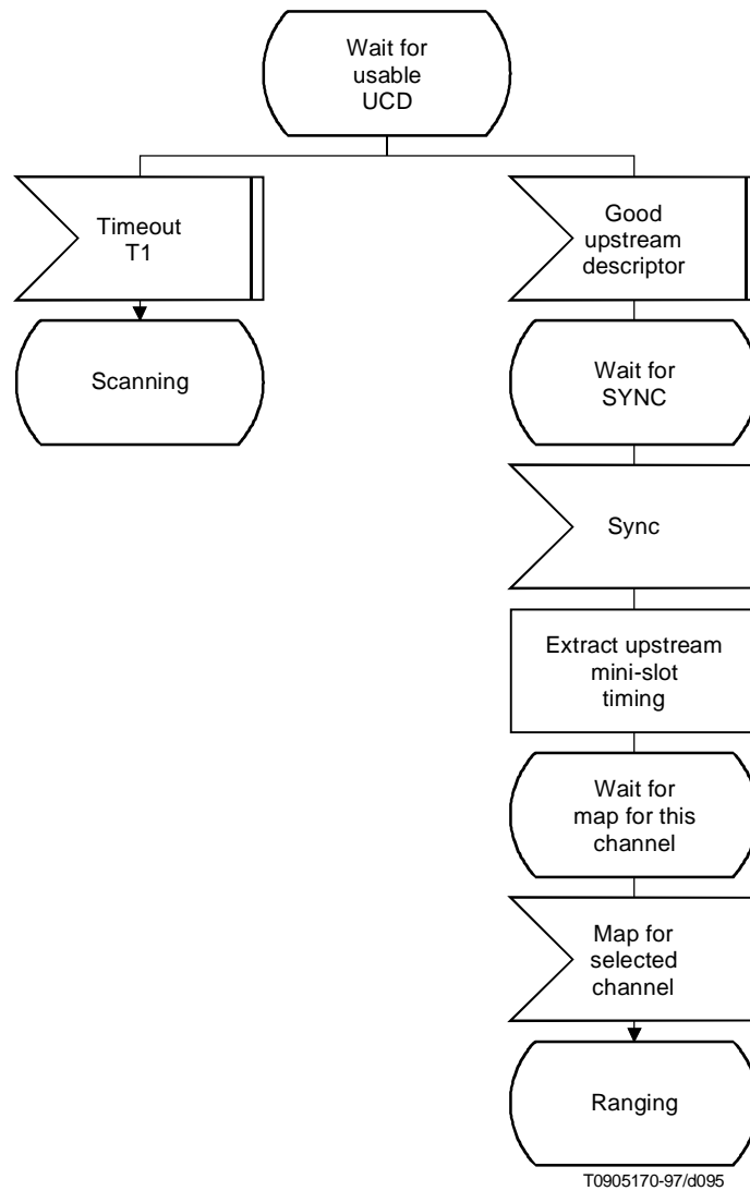
Figure B.7-3/J.112 – Obtaining upstream parameters
