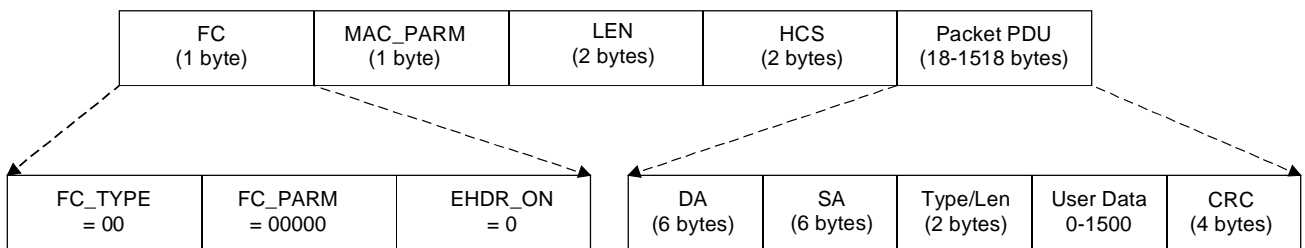
Figure C.6-8/J.112 – Packet-based MAC frame
