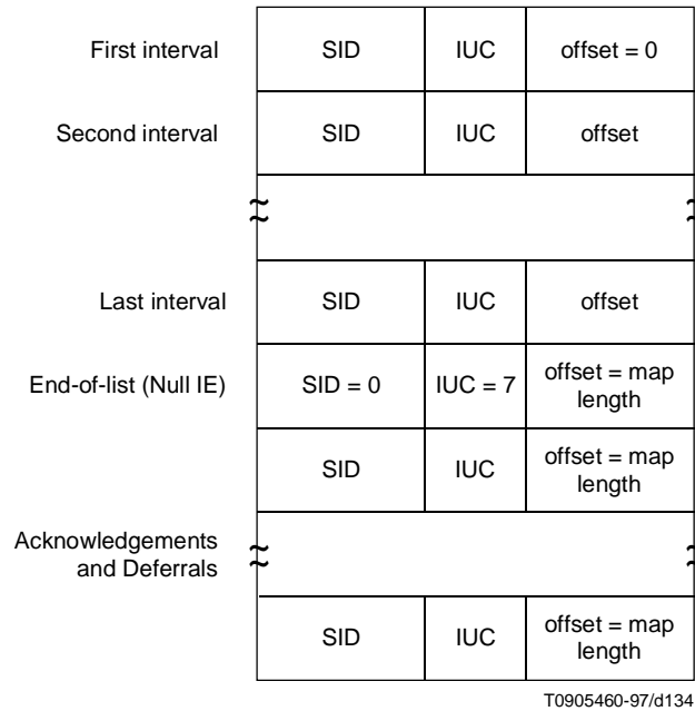
Figure C.6-21/J.112 – MAP information element coding
