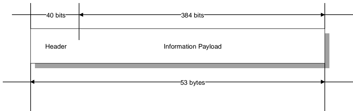
Figure A.18/J.112 – ATM cell format
