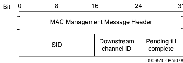
Figure B.6-20/J.112 – Packet PDU following the Timing Header
