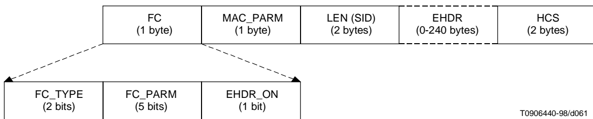
Figure B.6-3/J.112 – MAC Header format
