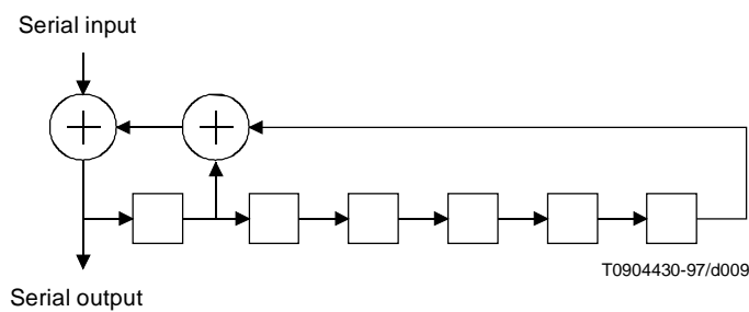
Figure A.10/J.112 – Randomizer
