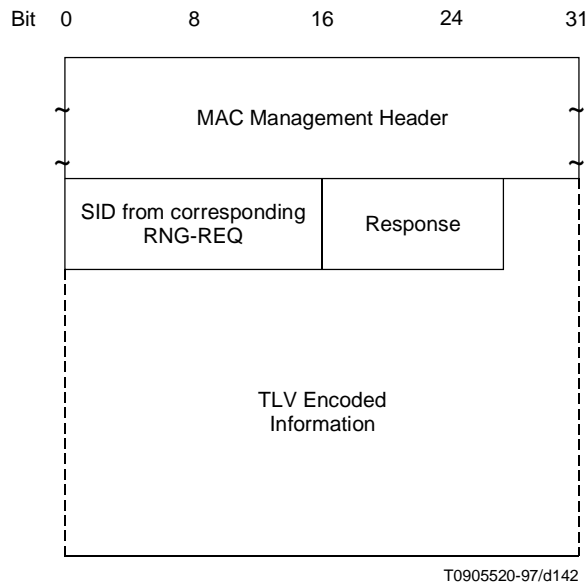
Figure C.6-29/J.112 – REG-RSP message
