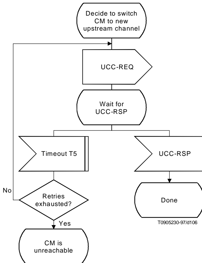
Figure B.7-14/J.112 – Changing upstream channels – CMTS view
