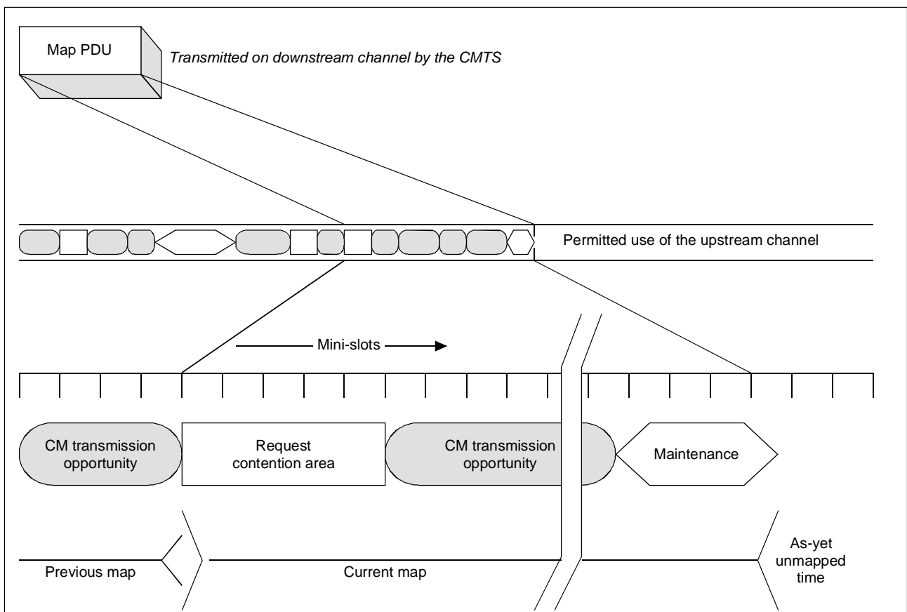
Figure B.6-31/J.112 – Allocation map
