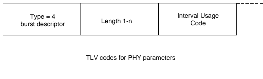
Figure C.6-18/J.112 – Burst Descriptor format
