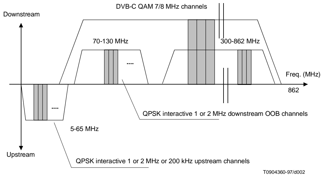
Figure A.3/J.112 – DVB preferred frequency ranges for CATV interactive systems
