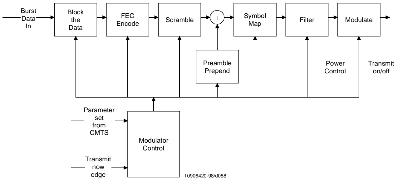
Figure B.4-8/J.112 – Signal-processing sequence
