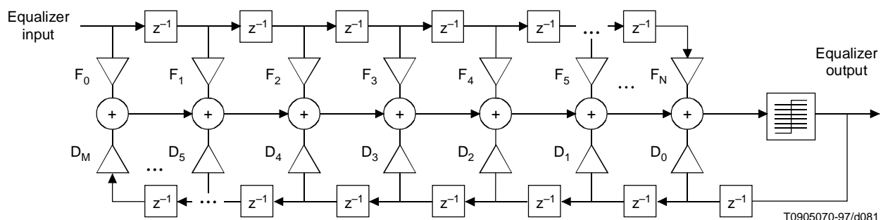
Figure B.6-23/J.112 – CMTS demodulator equalizer tap location definition
