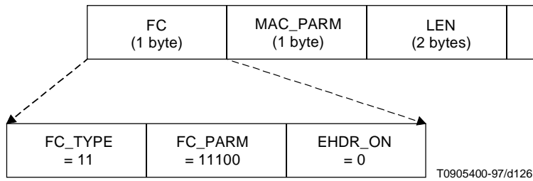
Figure C.6-13/J.112 – MAC Concatenation Header
