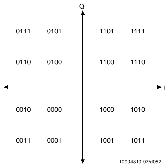
Figure B.4-2/J.112 – 16 QAM Gray-coded symbol mapping
