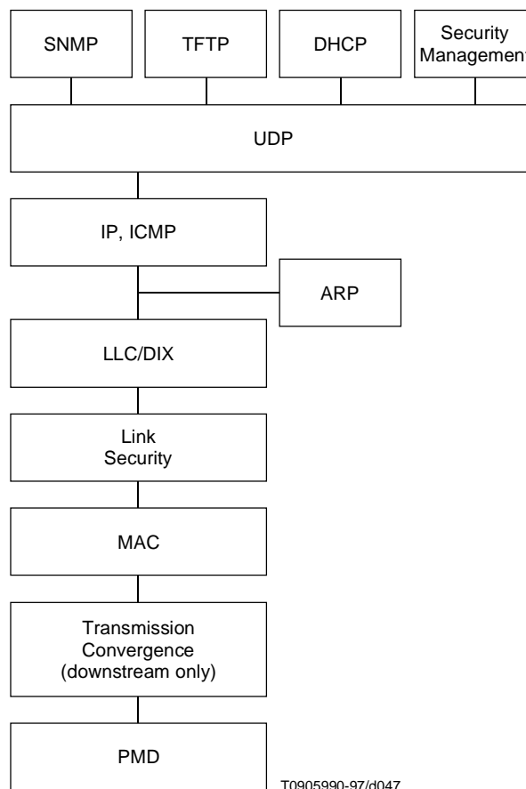
Figure B.3-1/J.112 – Protocol stack on the RF interface
