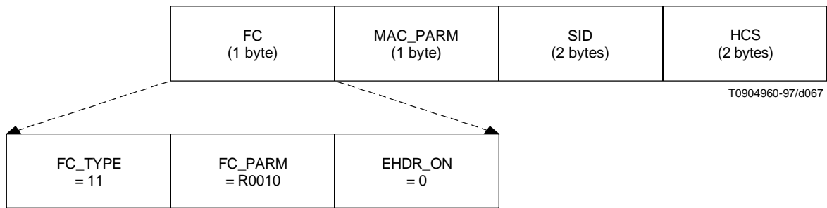
Figure B.6-9/J.112 – Request MAC Header format
