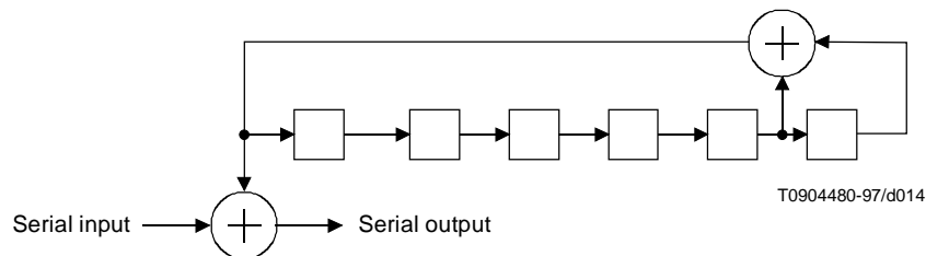
Figure A.15/J.112 – Randomizer
