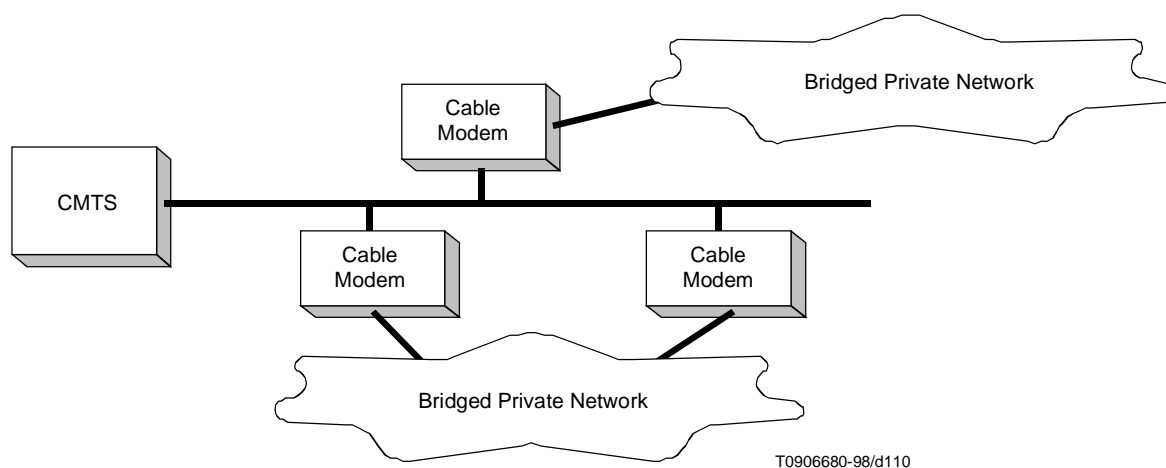
Figure B.VIII-1/J.112 – Spanning tree topology
