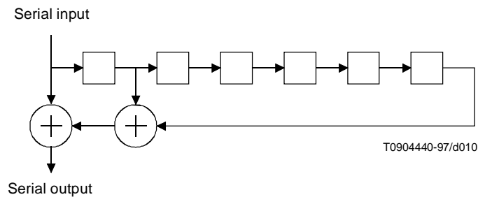
Figure A.11/J.112 – De-randomizer
