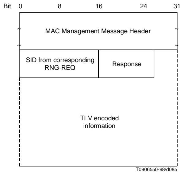
Figure B.6-27/J.112 – Registration Response format
