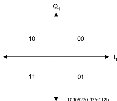
Figure C.4-1/J.112 – QPSK Signal Constellation Diagram
