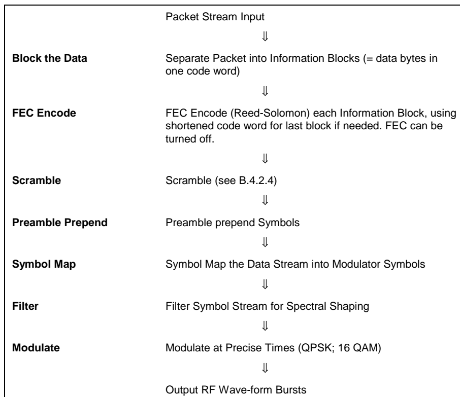
Figure B.4-9/J.112 – TDMA upstream transmission processing
