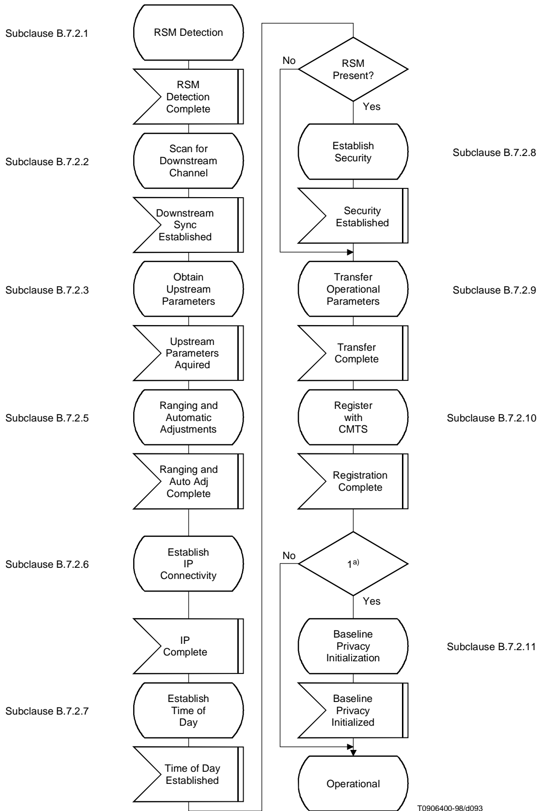
Figure B.7-1/J.112 – CM initialization overview
