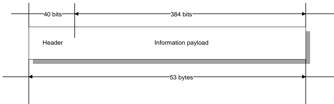
Figure A.22/J.112 – ATM cell format
