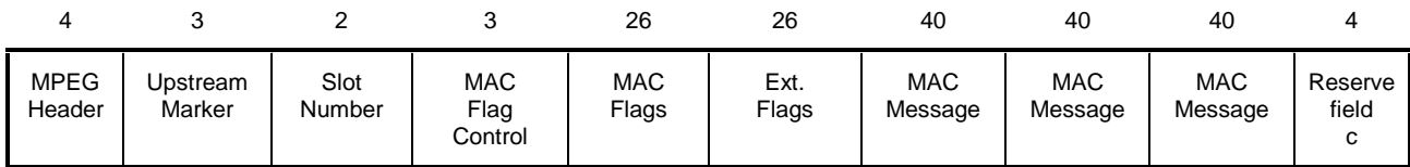
Figure A.20/J.112 – Frame structure (MPEG-2 TS format)
