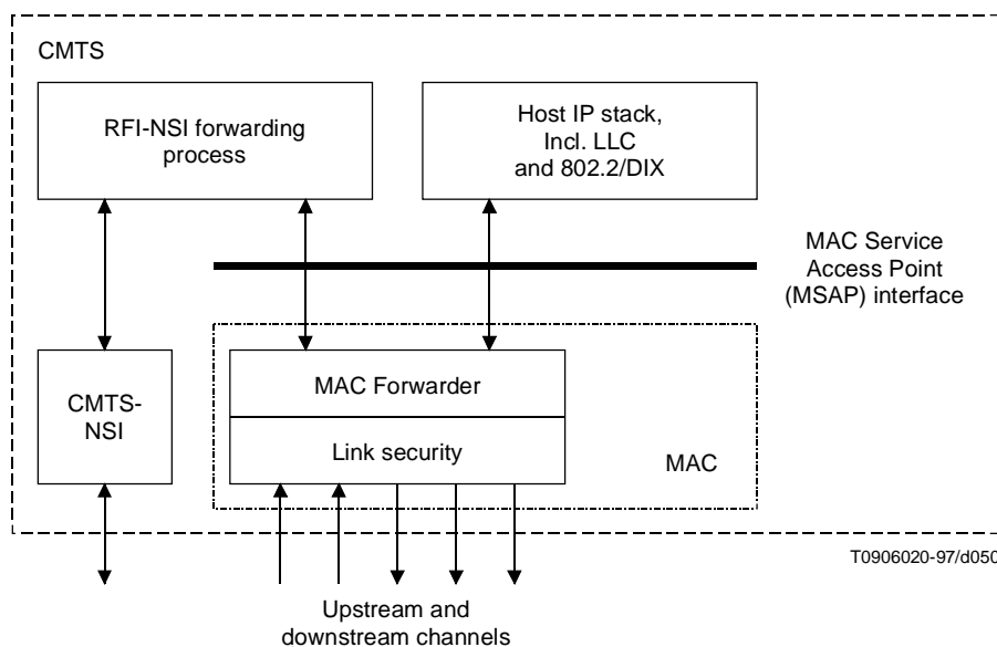
Figure B.3-4/J.112 – MAC Forwarder
