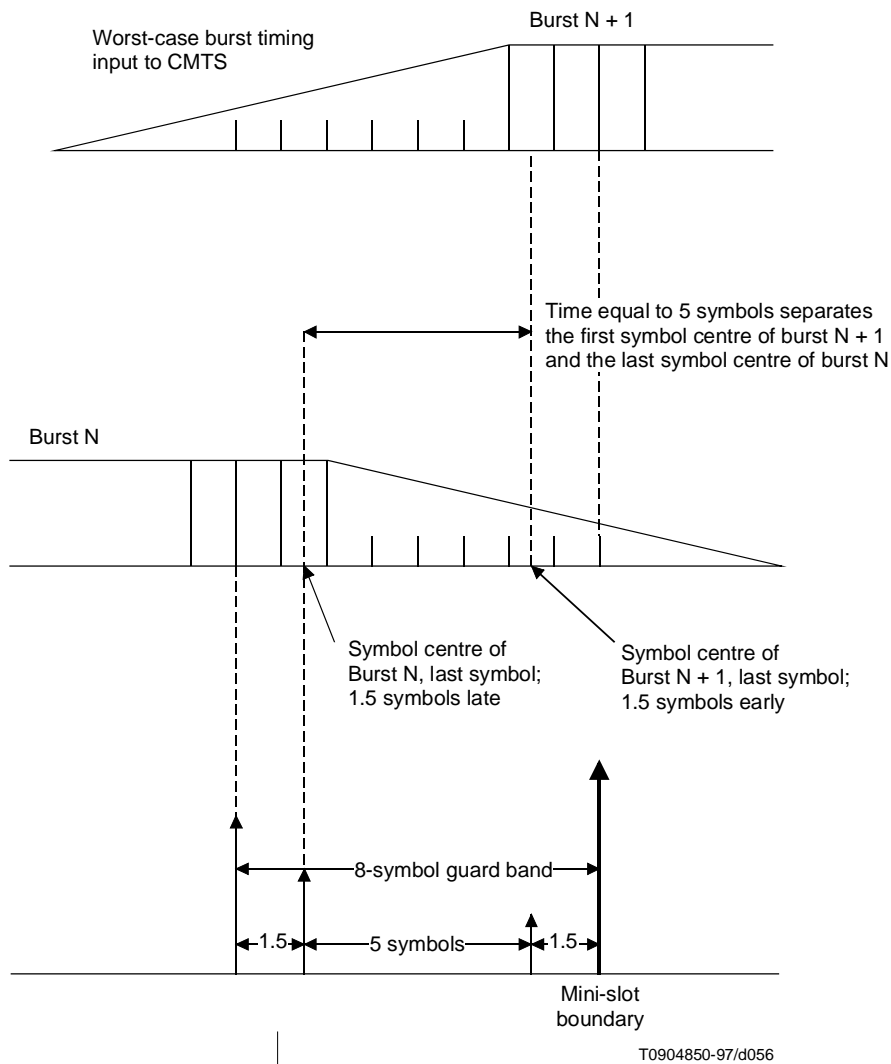
Figure B.4-6/J.112 – Worst-case burst timing
