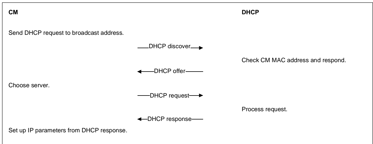
Figure B.7-9/J.112 – Establishing IP connectivity
