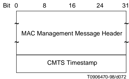
Figure B.6-14/J.112 – Format of Packet PDU following the timing Header
