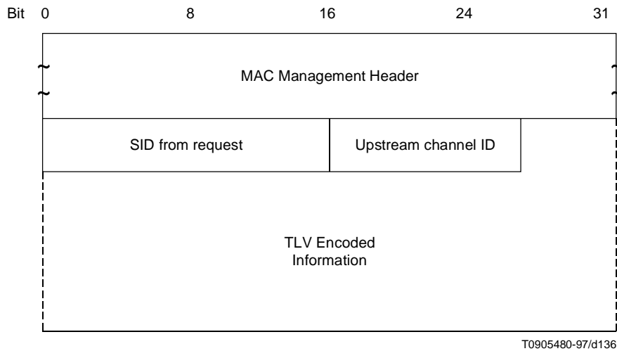
Figure C.6-23/J.112 – RNG-RSP message
