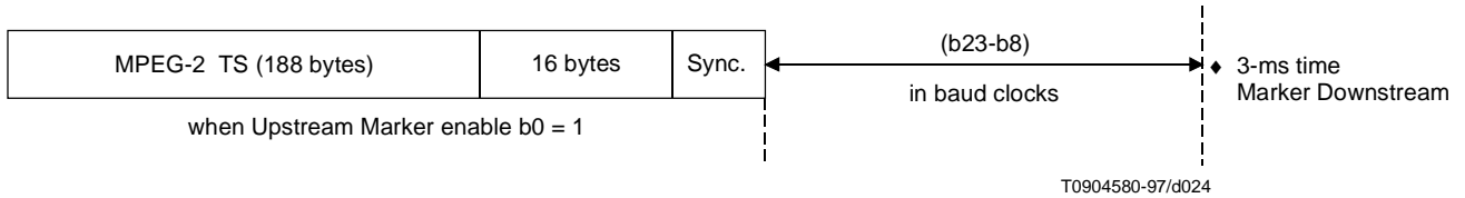
Figure A.23/J.112 – Position of the 3-ms time marker for IB signalling
