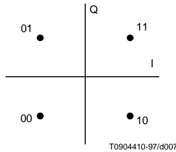
Figure A.8/J.112 – Mapping for the QPSK constellation (downstream OOB)
