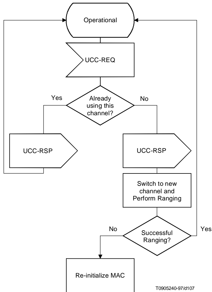
Figure B.7-15/J.112 – Changing Upstream Channels – CM view
