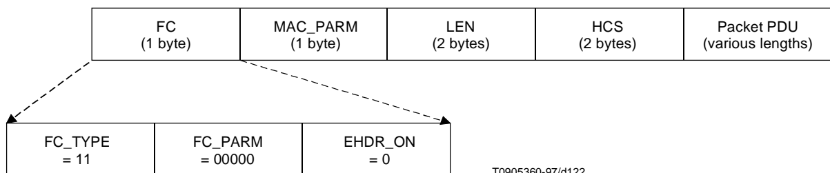
Figure C.6-9/J.112 – MAC timing header
