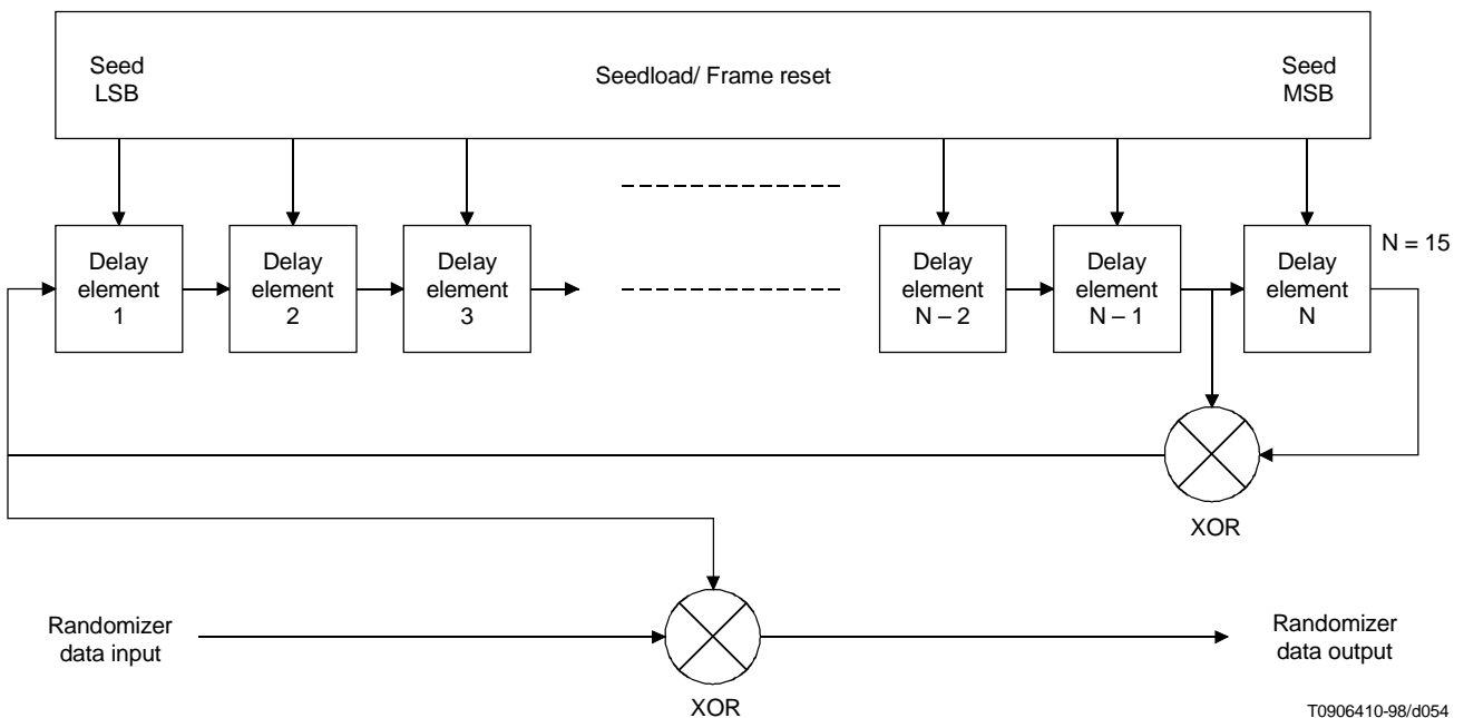
Figure B.4-4/J.112 – Scrambler structure
