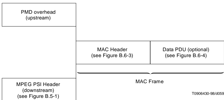
Figure B.6-1/J.112 – Generic MAC Frame format
