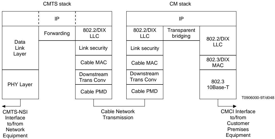
Figure B.3-2/J.112 – Data forwarding through the CM and CMTS
