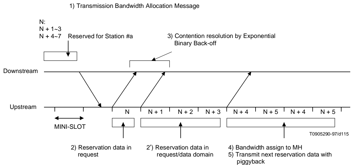
Figure C.6-2/J.112 – Bandwidth assignment by mini-slot and message
