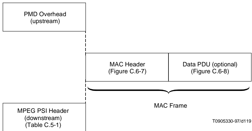
Figure C.6-6/J.112 – MAC Frame
