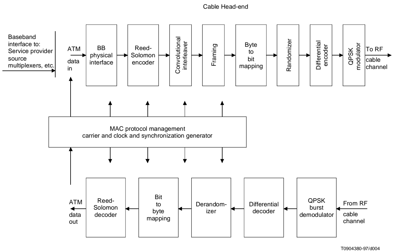
Figure A.5/J.112 – Conceptual block diagram for the OOB head-end transceiver
