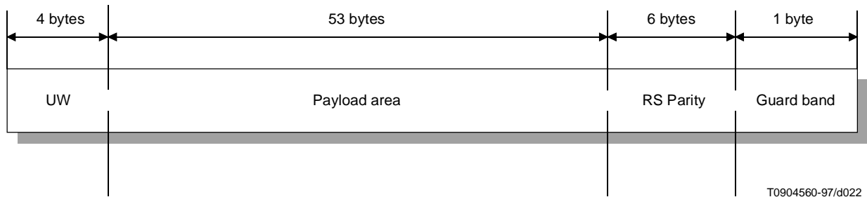
Figure A.21/J.112 – Slot format
