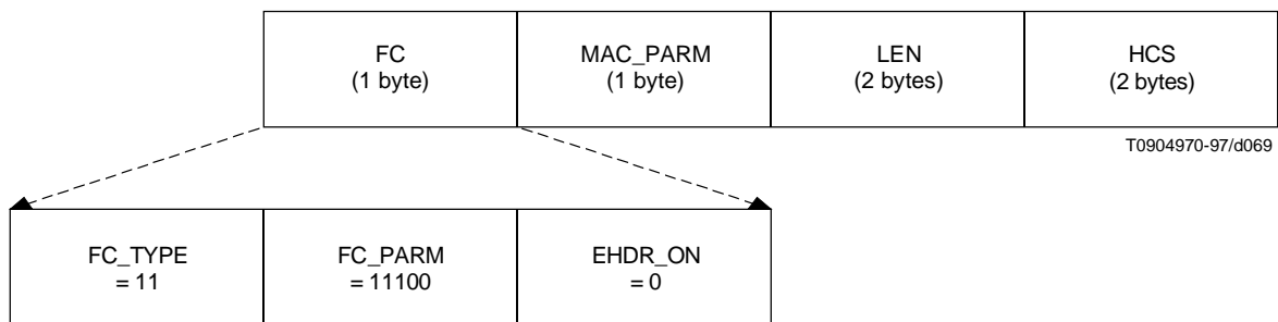
Figure B.6-11/J.112 – Concatenation MAC Header format
