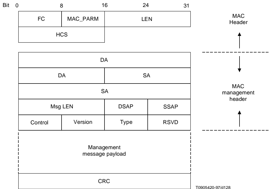
Figure C.6-15/J.112 – MAC management message
