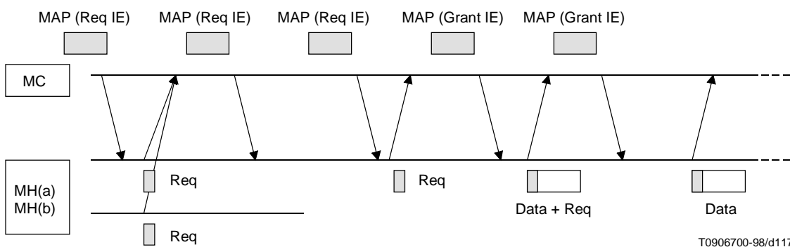
Figure C.6-4/J.112 – Random reservation sequence
