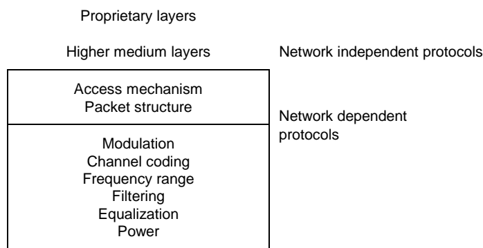
Figure A.1/J.112 – Layer structure for generic system reference model
