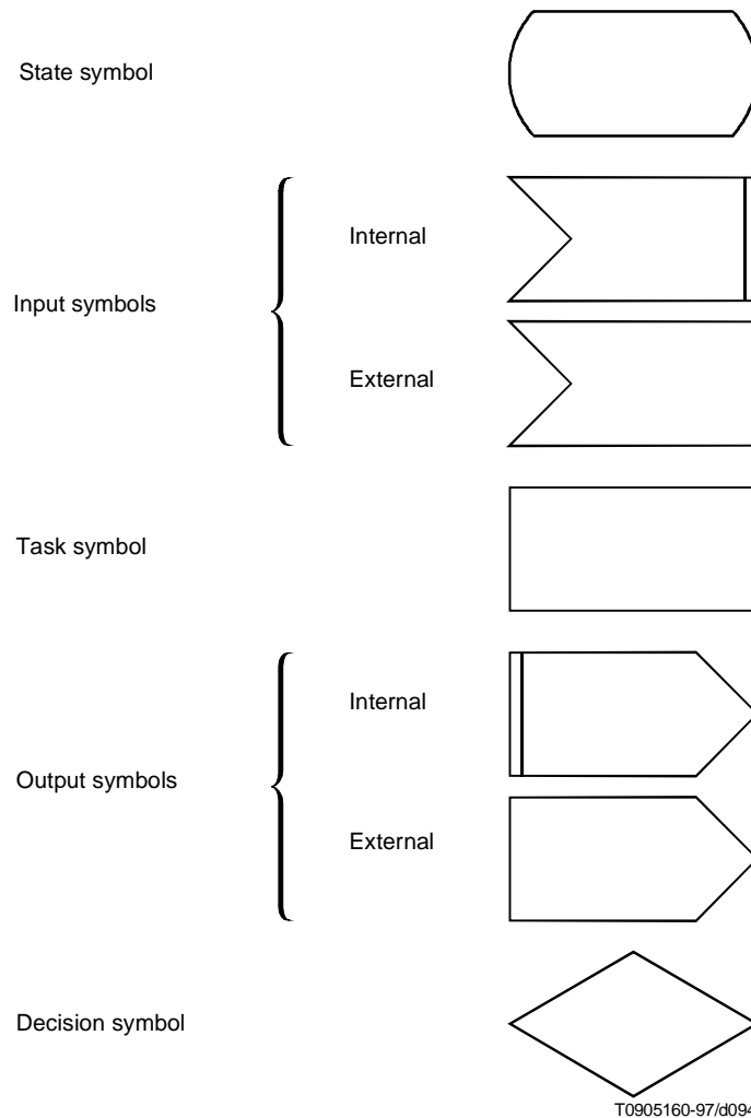
Figure B.7-2/J.112 – SDL notation
