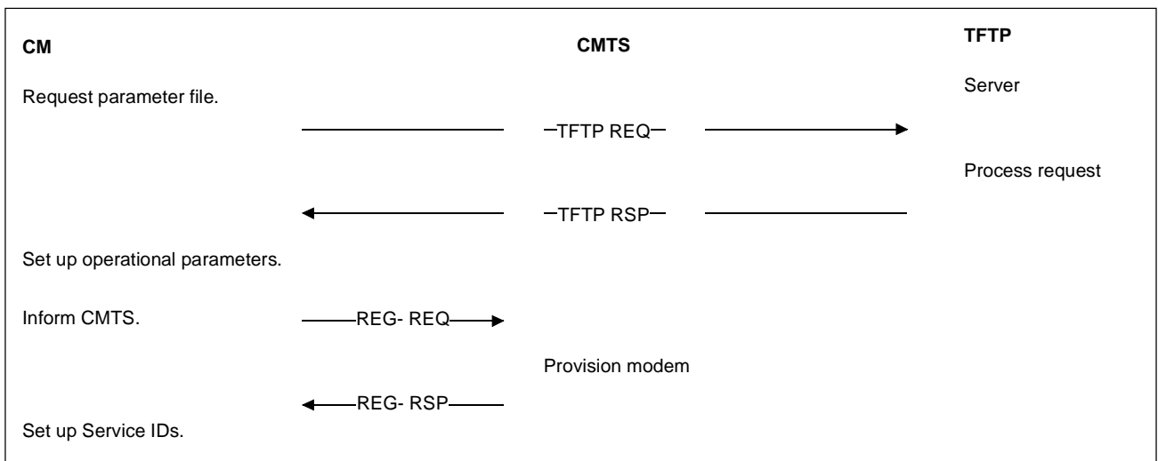
Figure B.7-11/J.112 – Transferring operational parameters and registration
