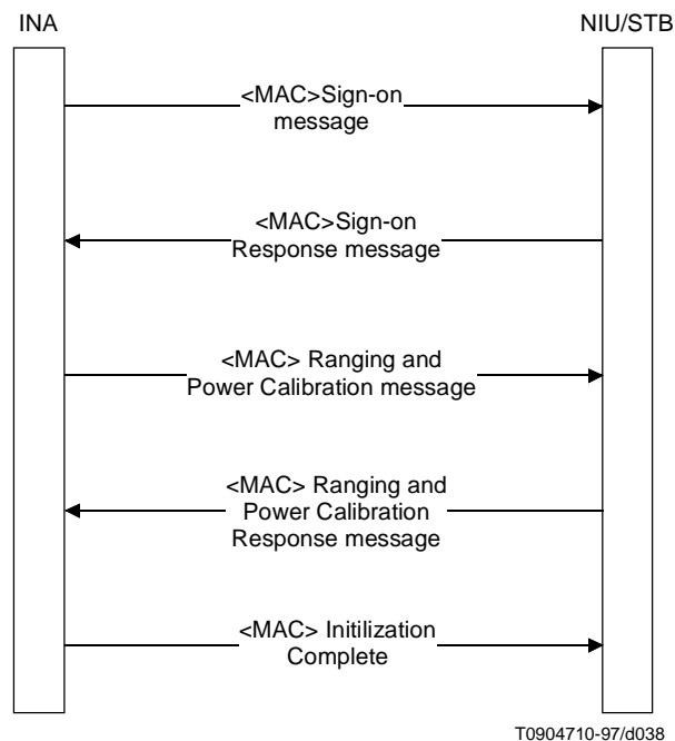
Figure A.29/J.112 – Ranging and calibration signalling
