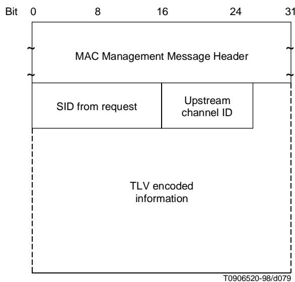
Figure B.6-21/J.112 – Ranging Response
