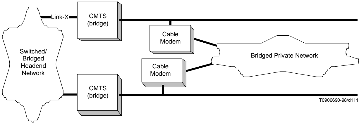
Figure B.VIII-2/J.112 – Spanning tree across CMTSs
