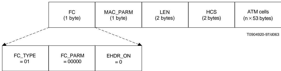
Figure B.6-5/J.112 – ATM cell MAC Frame format
