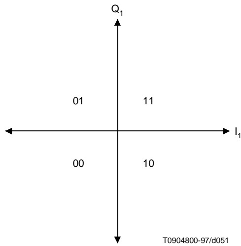
Figure B.4-1/J.112 – QPSK symbol mapping
