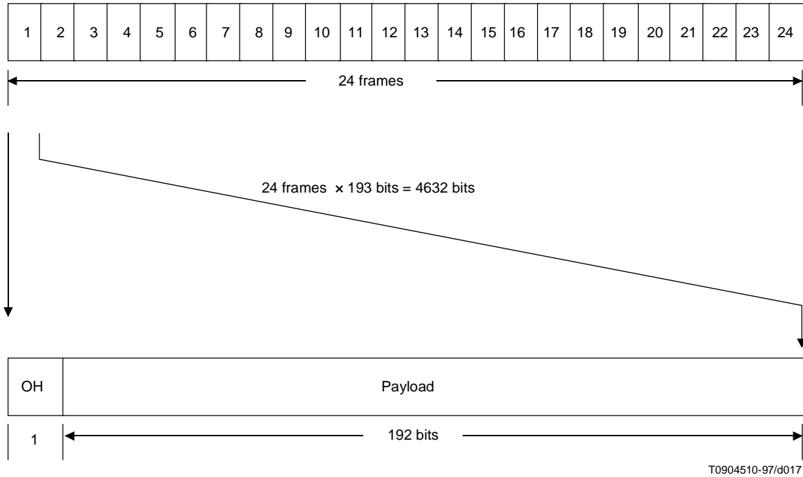
Figure A.17/J.112 – SL-ESF frame structure
