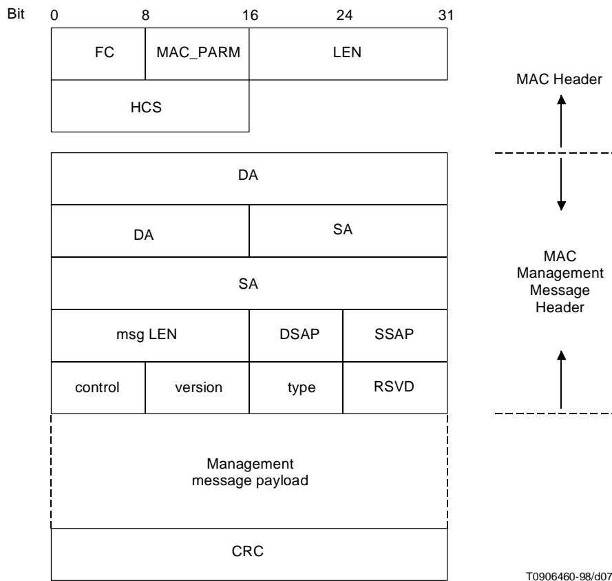
Figure B.6-13/J.112 – MAC Header and MAC Management Message Header fields
