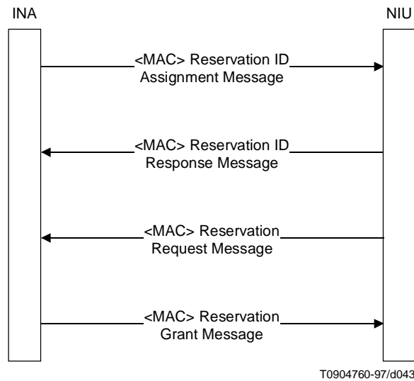
Figure A.34/J.112 – Reservation access signalling
