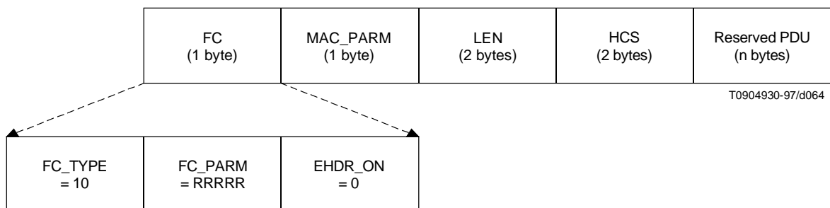
Figure B.6-6/J.112 – Reserved PDU format
