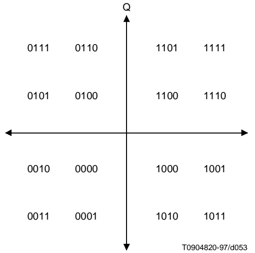
Figure B.4-3/J.112 – 16 QAM differential-coded symbol mapping
