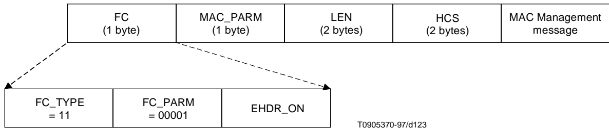
Figure C.6-10/J.112 – MAC management header
