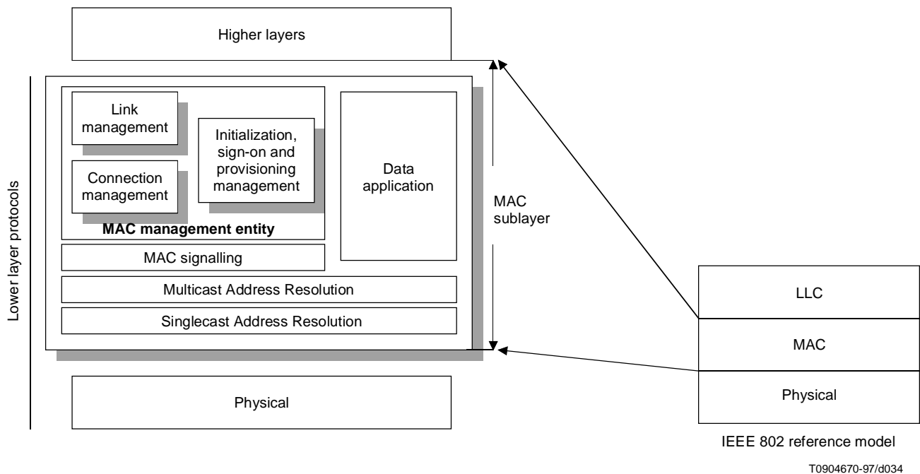
Figure A.25/J.112 – MAC reference model
