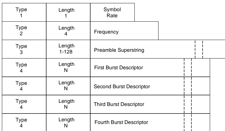
Figure C.6-19/J.112 – A Sample of Burst Descriptor coding
