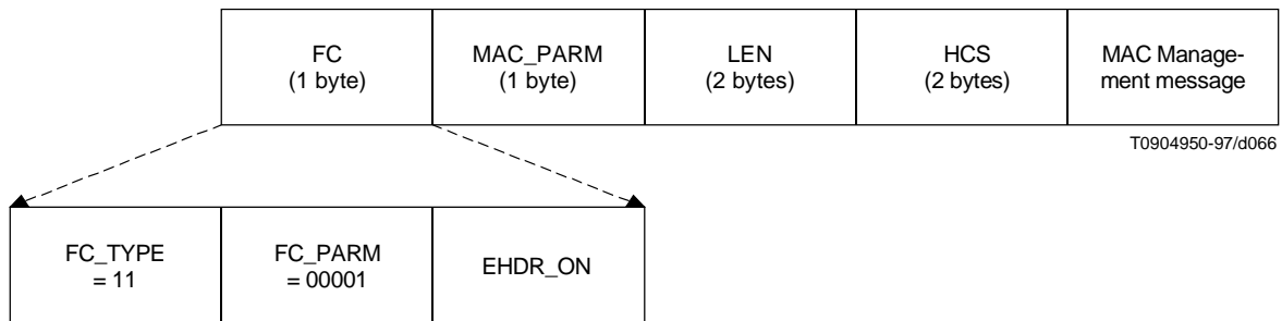
Figure B.6-8/J.112 – Management MAC Header
