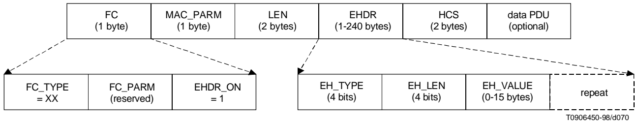
Figure B.6-12/J.112 – Extended MAC format
