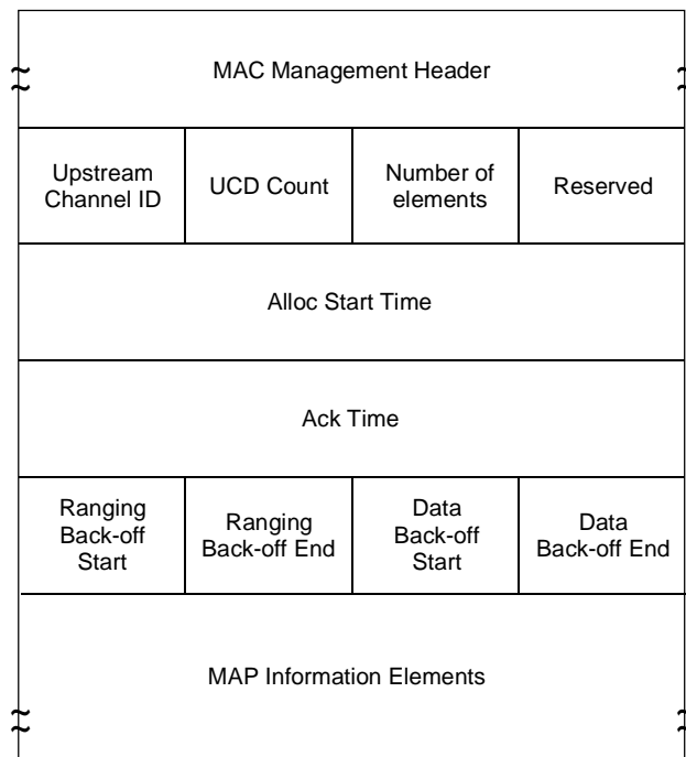
Figure C.6-20/J.112 – MAP message
