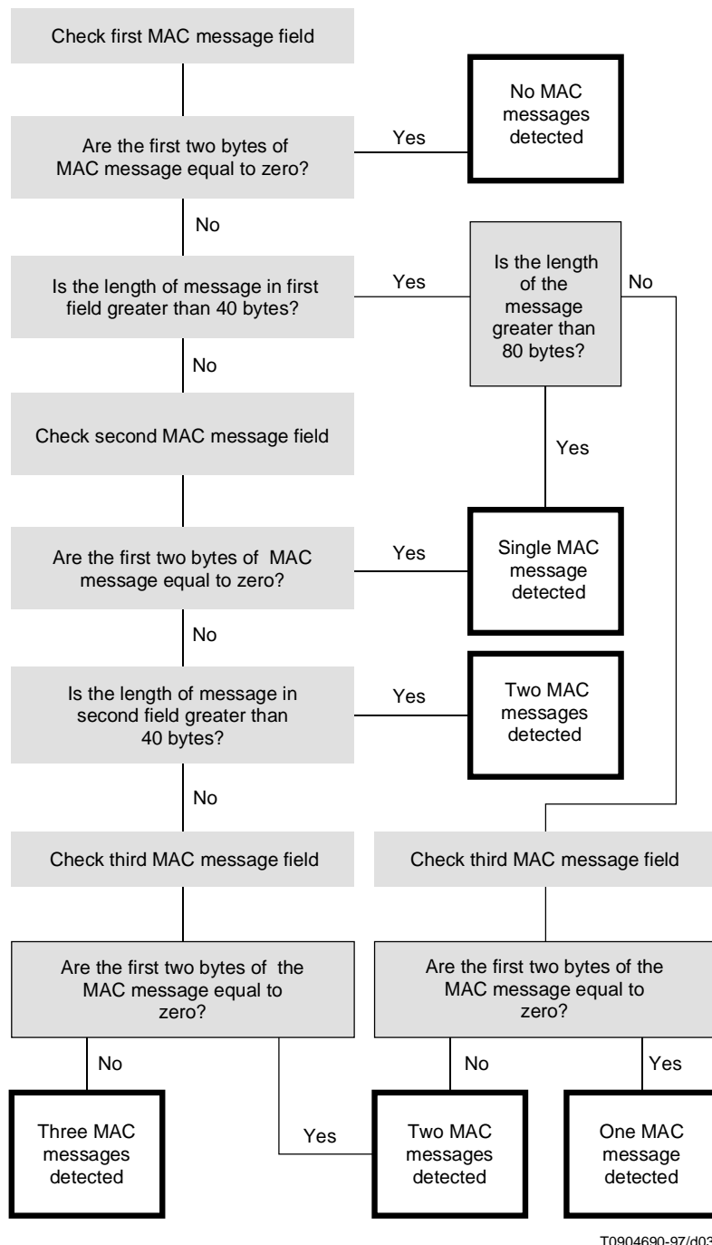
Figure A.27/J.112 – Algorithm when MAC messages are sent IB downstream
