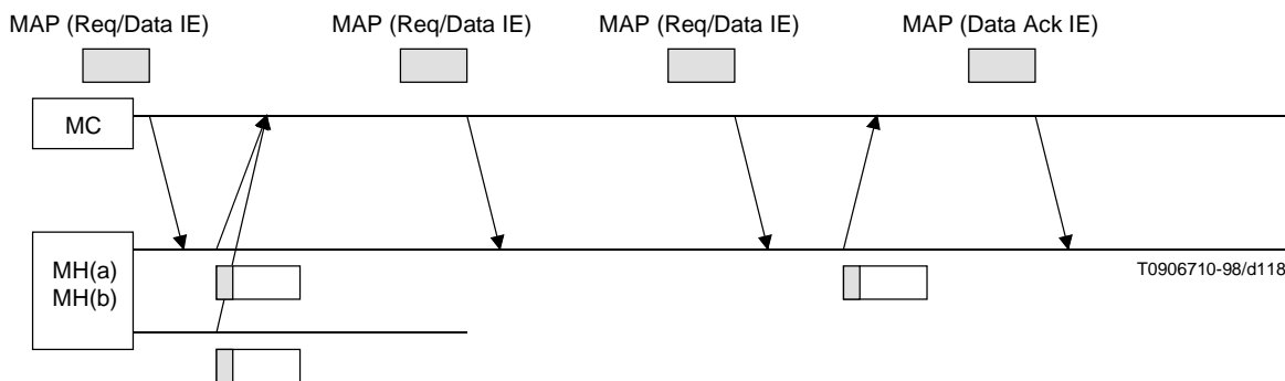
Figure C.6-5/J.112 – Random access sequence
