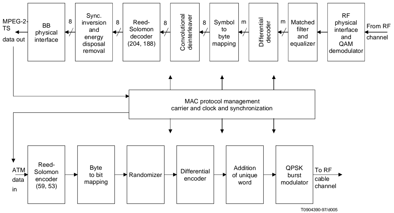
Figure A.6/J.112 – Conceptual block diagram for the IB NIU transceiver
