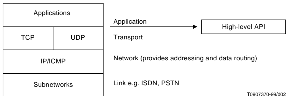
Figure 2 – TCP/IP model
