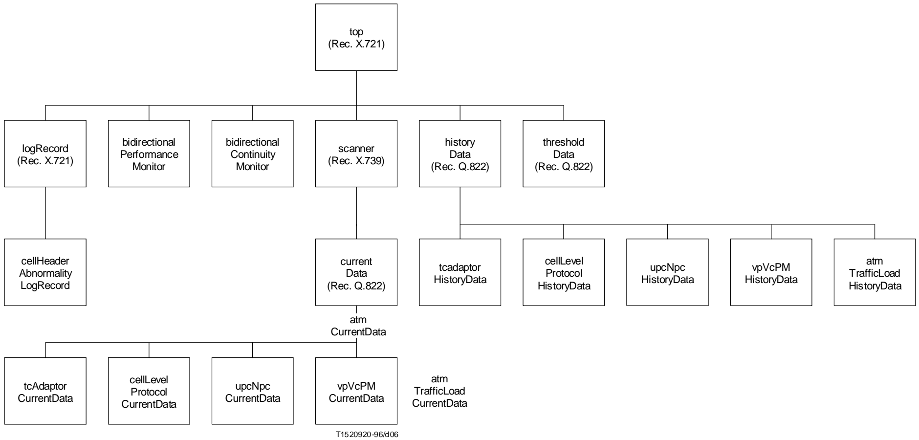
FIGURE 7-1/I.751 (part 2) Inheritance tree for ATM objects
