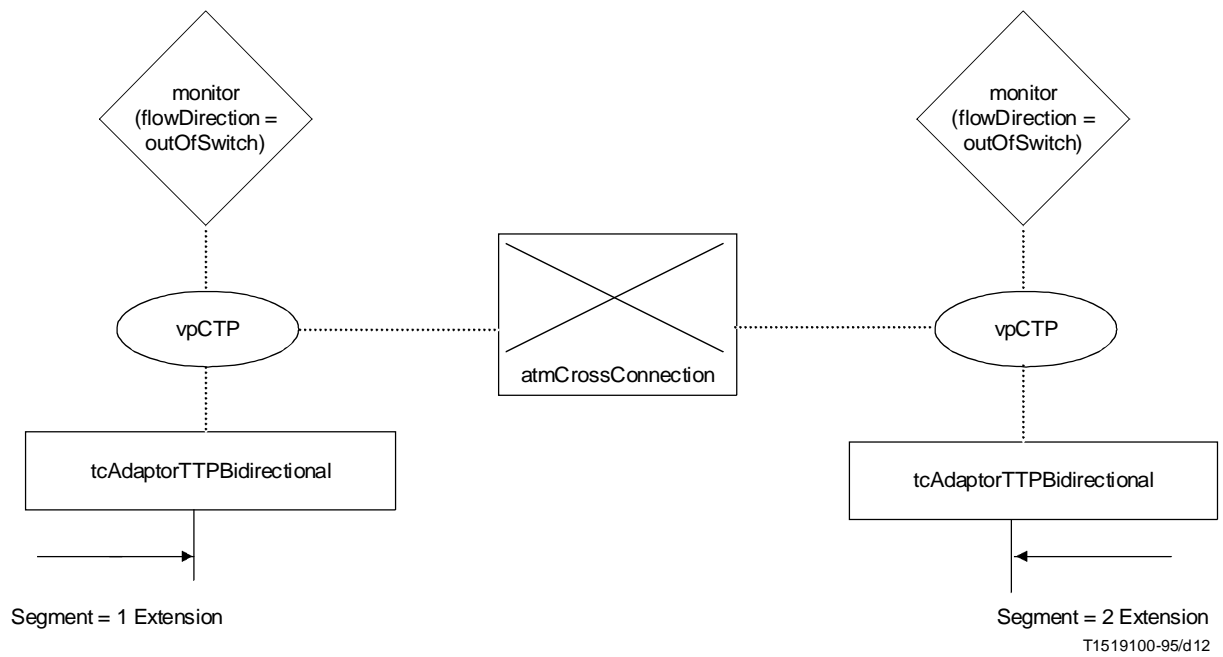
FIGURE I.4/I.751 Case D, the monitor objects and the segment extension definition
