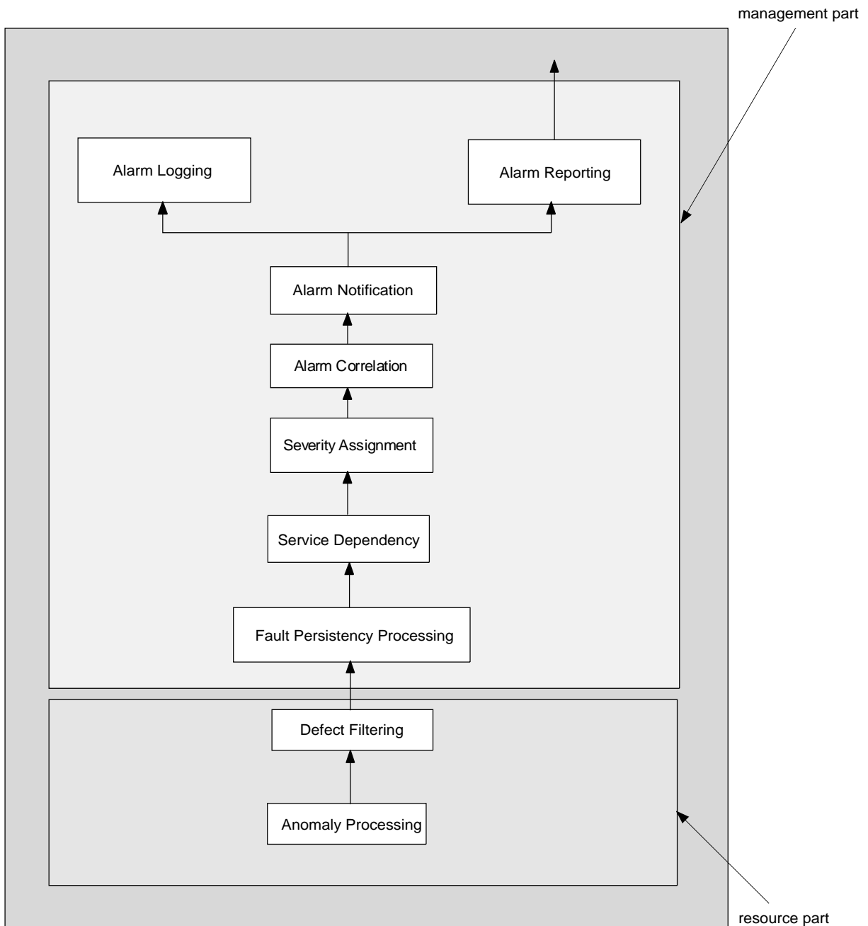
FIGURE 6-1/I.751 Functional architecture of the alarm process 3)
