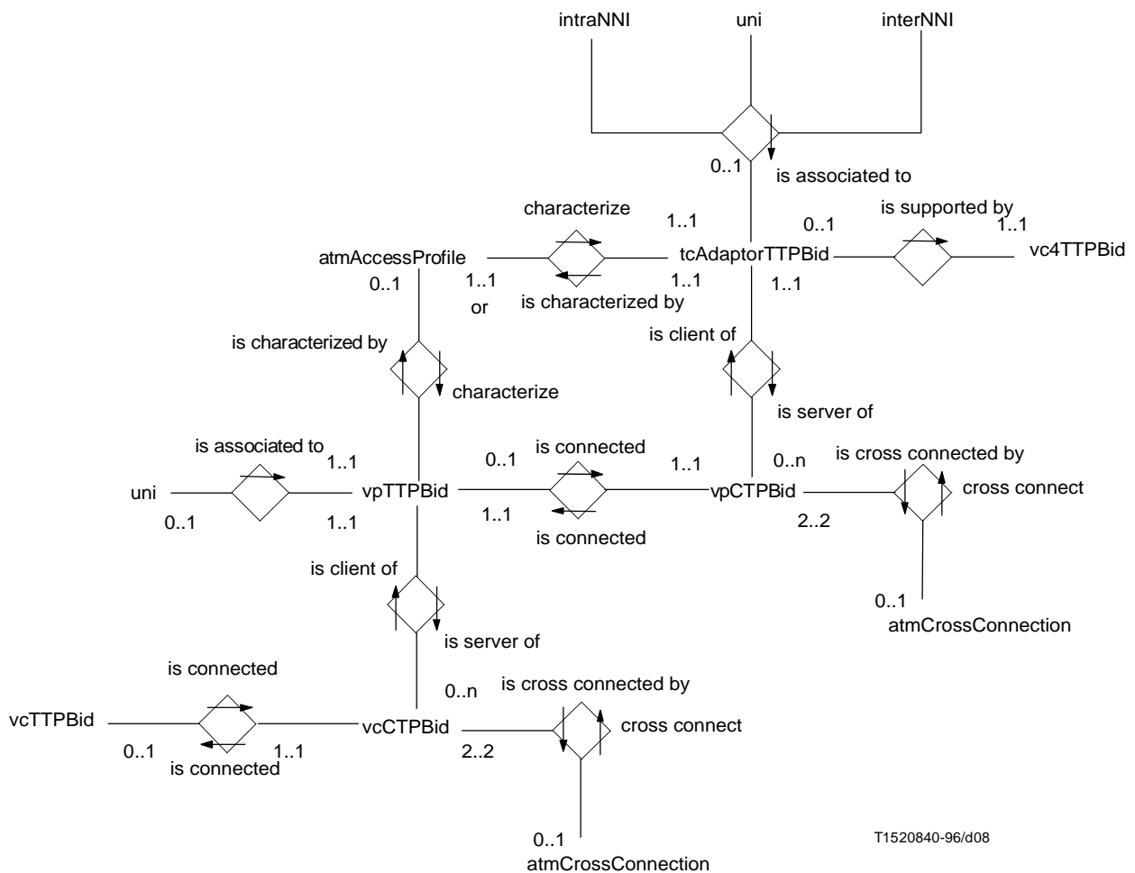
FIGURE 7-3/I.751 ATM Entity-Relationship diagram
