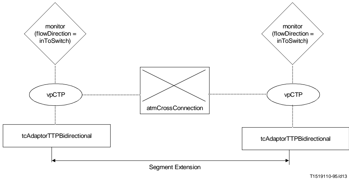
FIGURE I.5/I.751 Case E, the monitor objects and the segment extension definition
