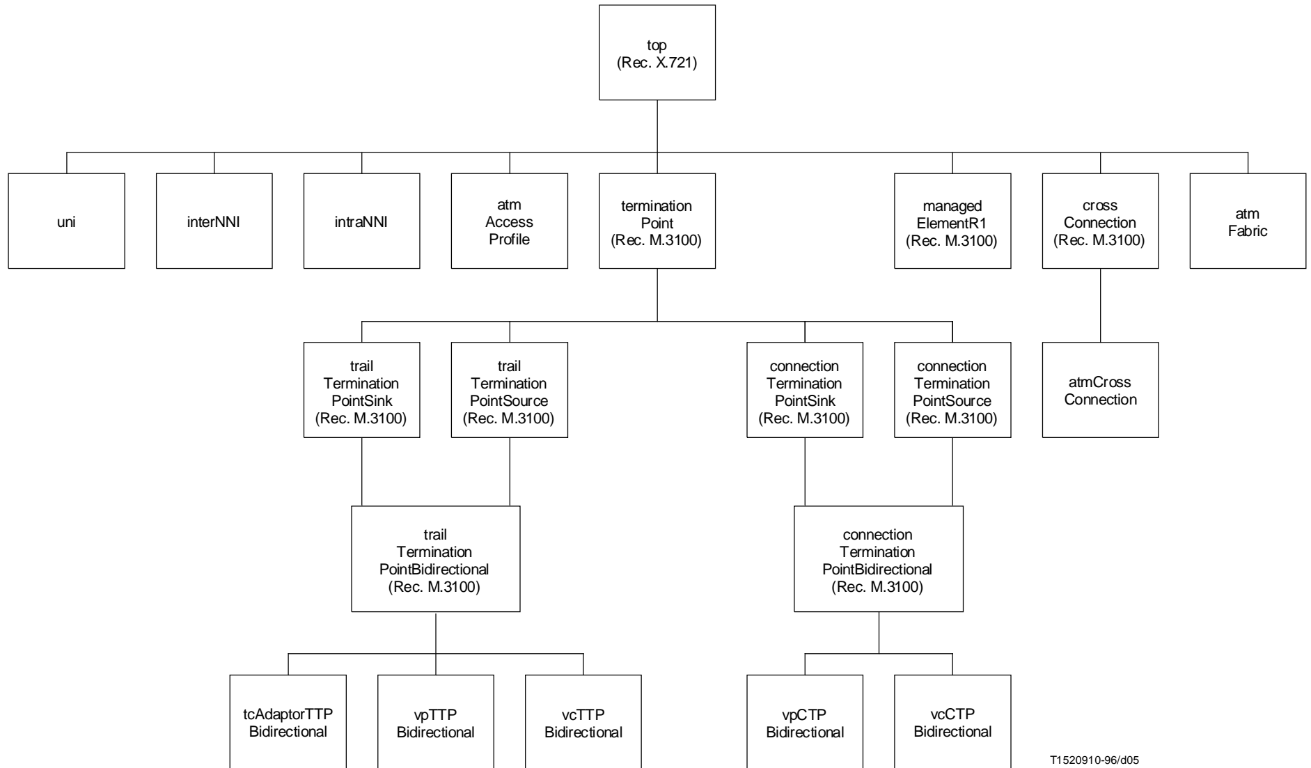
FIGURE 7-1/I.751 (part 1) Inheritance tree for ATM objects
