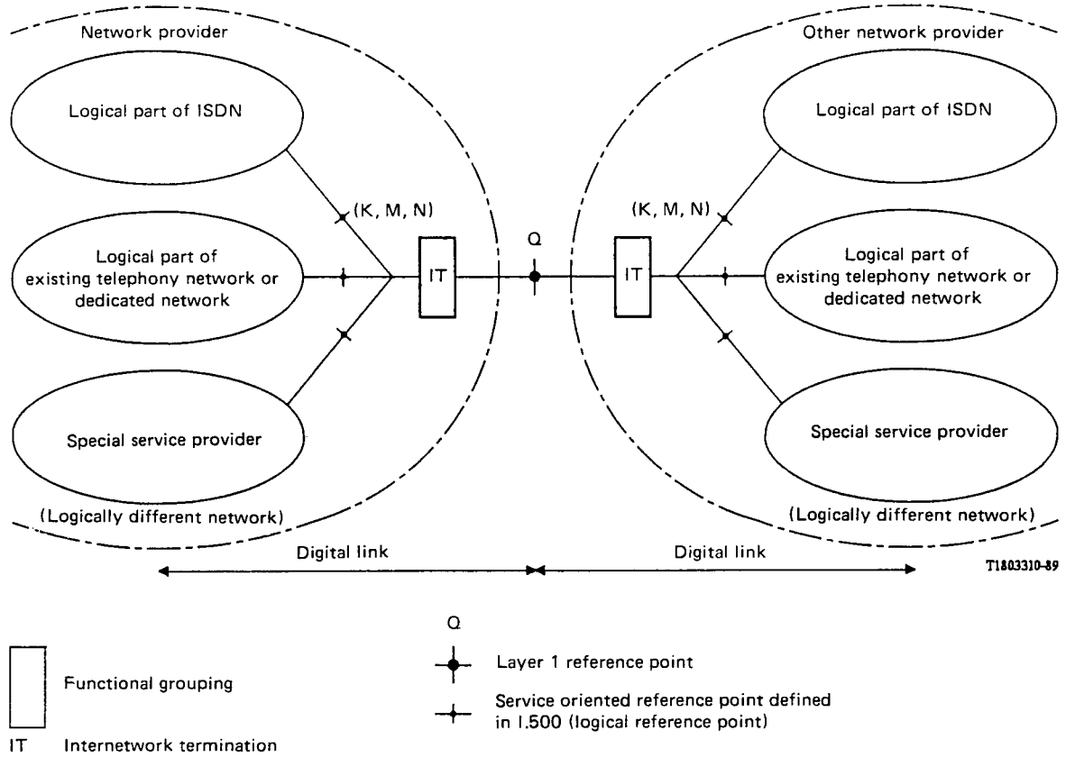
FIGURE 1/I.511 Reference configuration for the ISDN-related internetwork interface at layer 1
