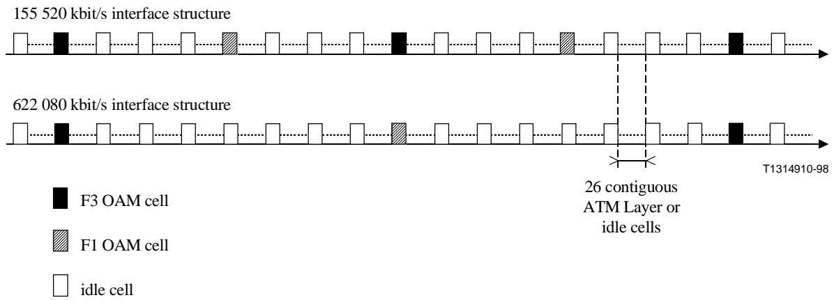
Figure 7/I.432.2 – Interface structure
