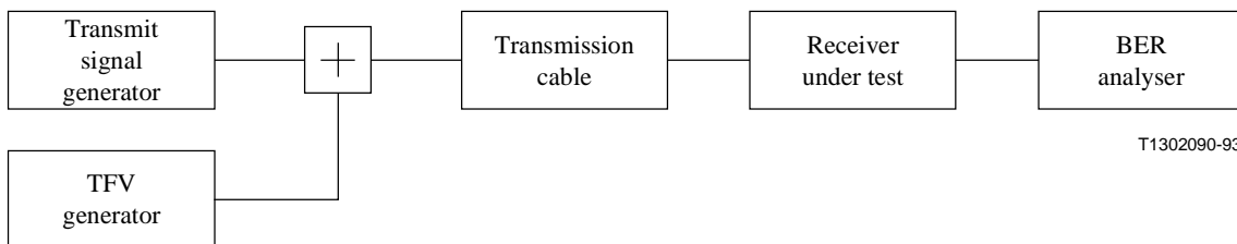
Figure 3/I.432.2 – Measurement configuration
