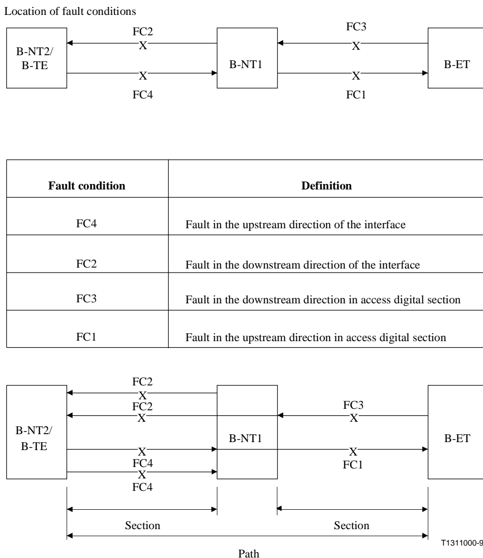
Figure 9/I.432.2 – Fault conditions and operational span of section path maintenance signals
