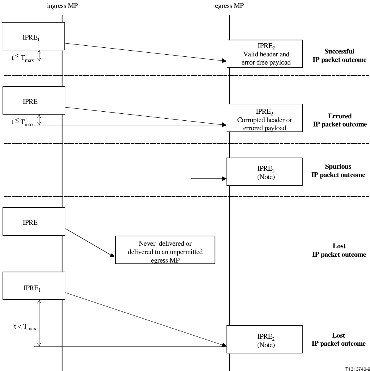
Figure 6/I.380 – IP packet transfer outcomes
