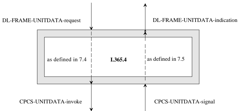
Figure 2/I.365.4 – Relationship of DL-FRAME primitives and AAL type 5 CPCS signals
