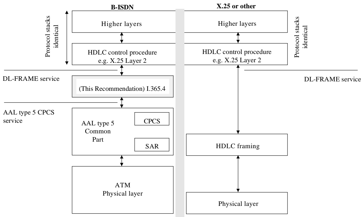
Figure 1/I.365.4 – Environment for the DL-FRAME SSCS for HDLC applications
