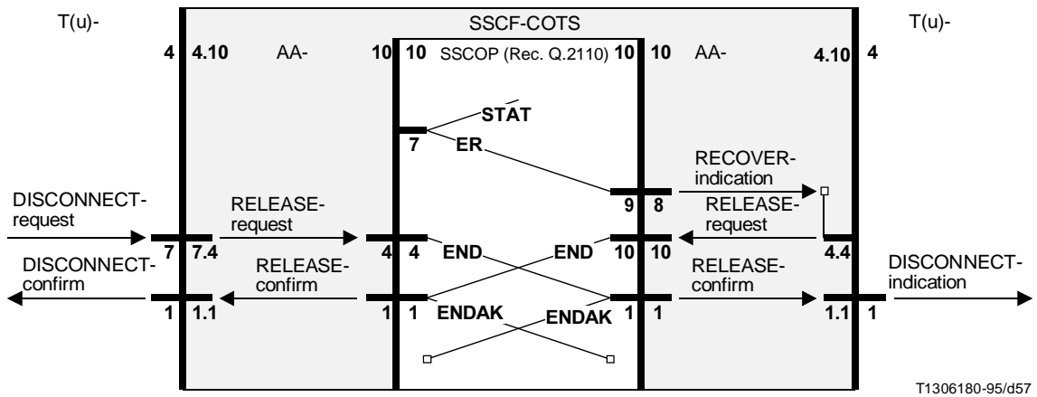
FIGURE I.20/I.365.3 Sequences for a provider initiated release of a T(u)-connection followed immediately by a user release
