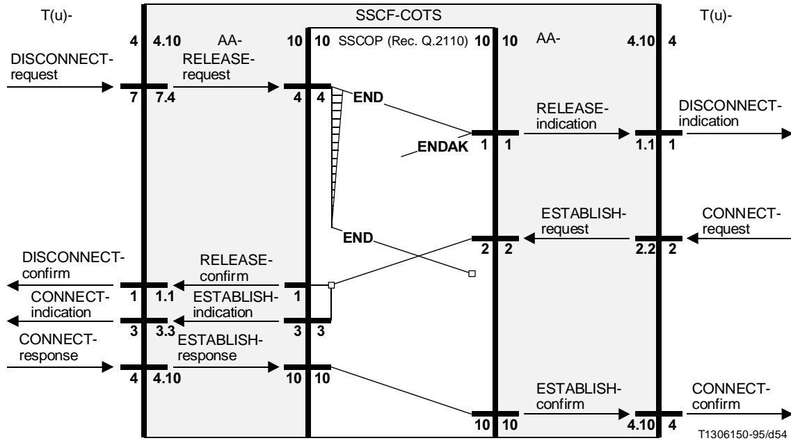
FIGURE I.17/I.365.3 Sequences for release of a T(u)-connection PDU corruption followed by a T(u)-connection establishment
