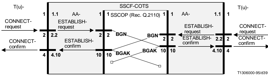
FIGURE I.2/I.365.3 Sequences for establishing a T(u)-connection with collision
