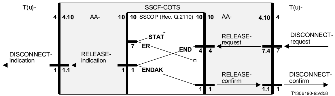
FIGURE I.21/I.365.3 Sequences for release of a T(u)-connection concurrently with a provider initiated release
