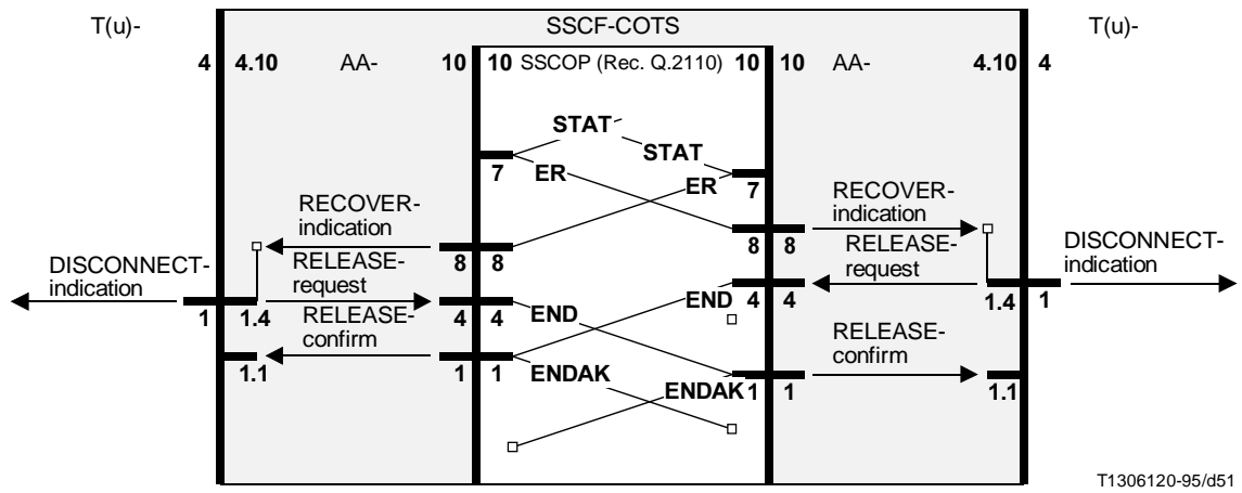
FIGURE I.14/I.365.3 Sequences for provider initiated release of a T(u)-connection with collision
