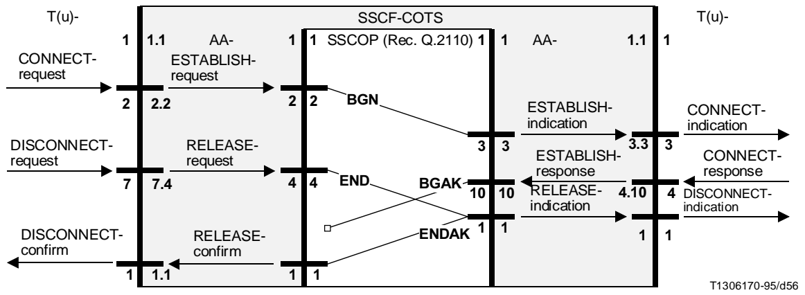
FIGURE I.19/I.365.3 Sequences for establishing a T(u)-connection followed immediately by a release
