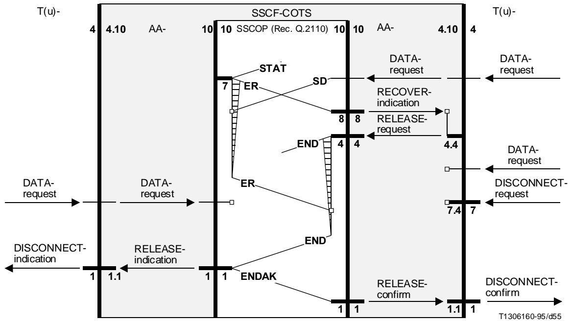
FIGURE I.18/I.365.3 Sequences for provider initiated release of a T(u)-connection with PDU followed by a connection release
