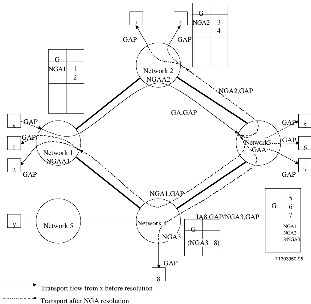
Figure 24/I.364 – Centralized database approach with one level of NGAs – An example of the addition of a new member
