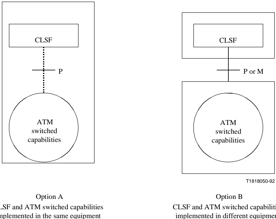
Figure 2/I.364 – Implementation of CLSF and ATM switched capabilities
