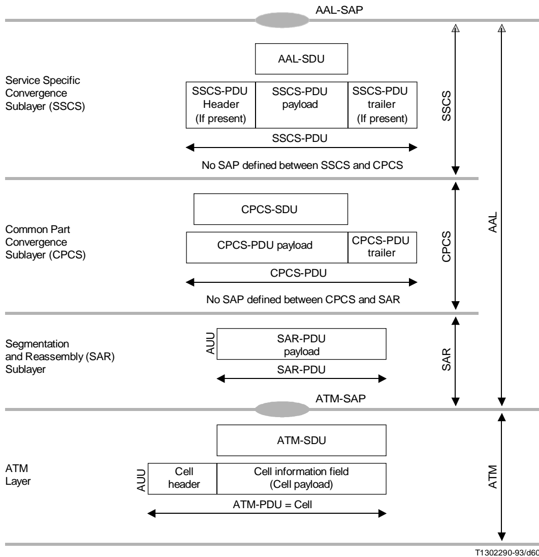
FIGURE A.4/I.363 Data unit naming conventions for the AAL type 5
