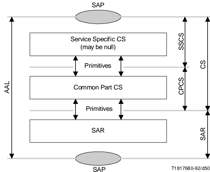
FIGURE 6-1/I.363 Structure of the AAL type 5
