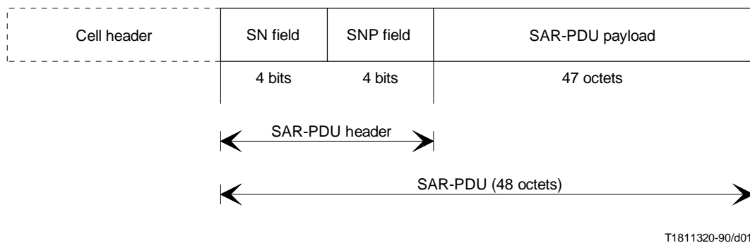
FIGURE 1/I.363 SAR-PDU format of AAL type 1
