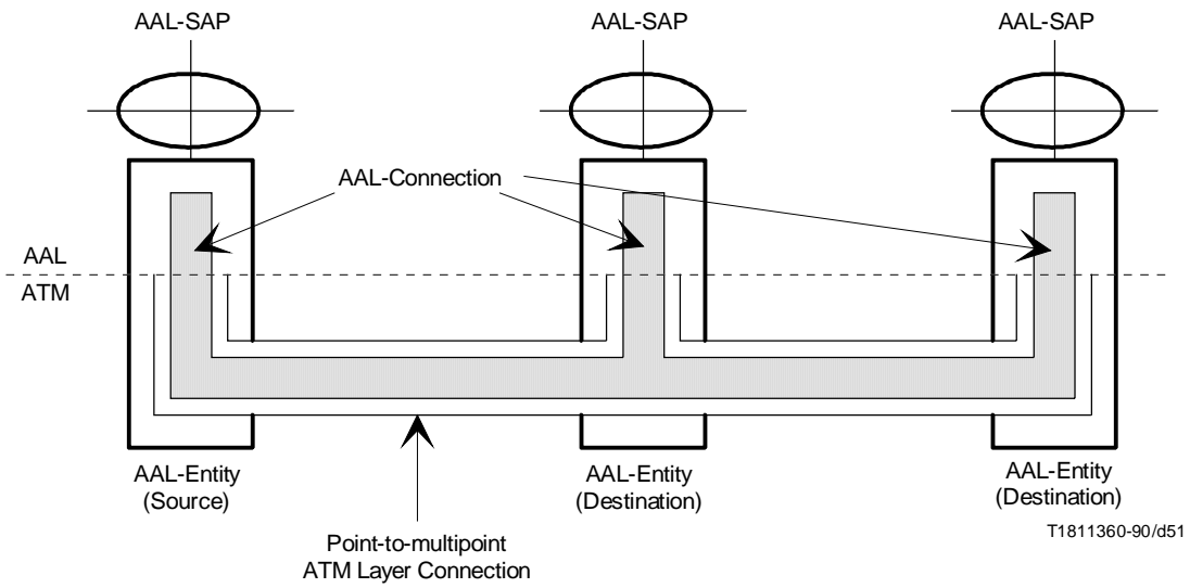
b) Point-to-multipoint AAL connection
