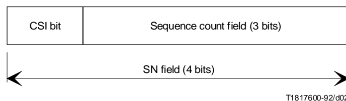
FIGURE 2/I.363 Sequence number (SN) field format
