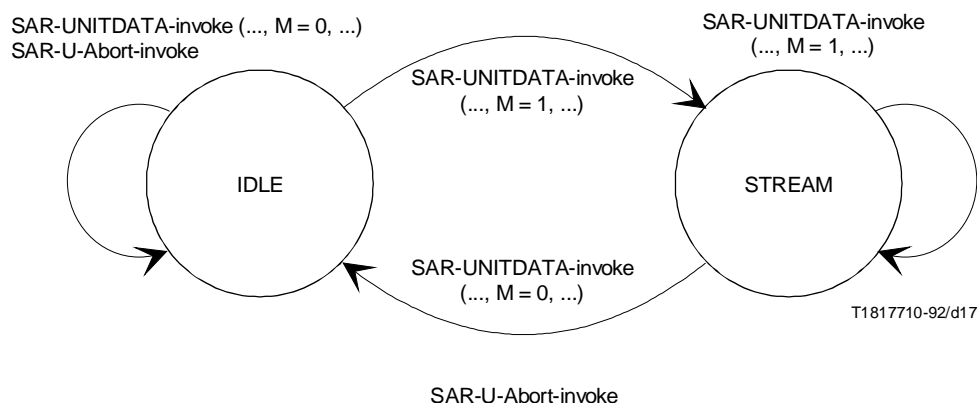
FIGURE 17/I.363 State transition diagram for the SAR sender
