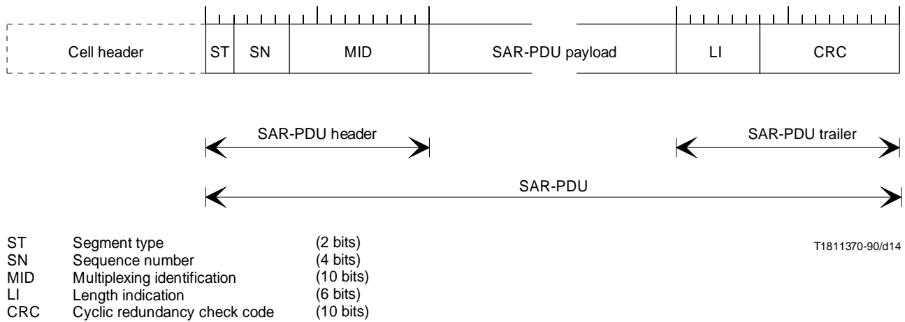
FIGURE 14/I.363 SAR-PDU format for AAL type 3/4
