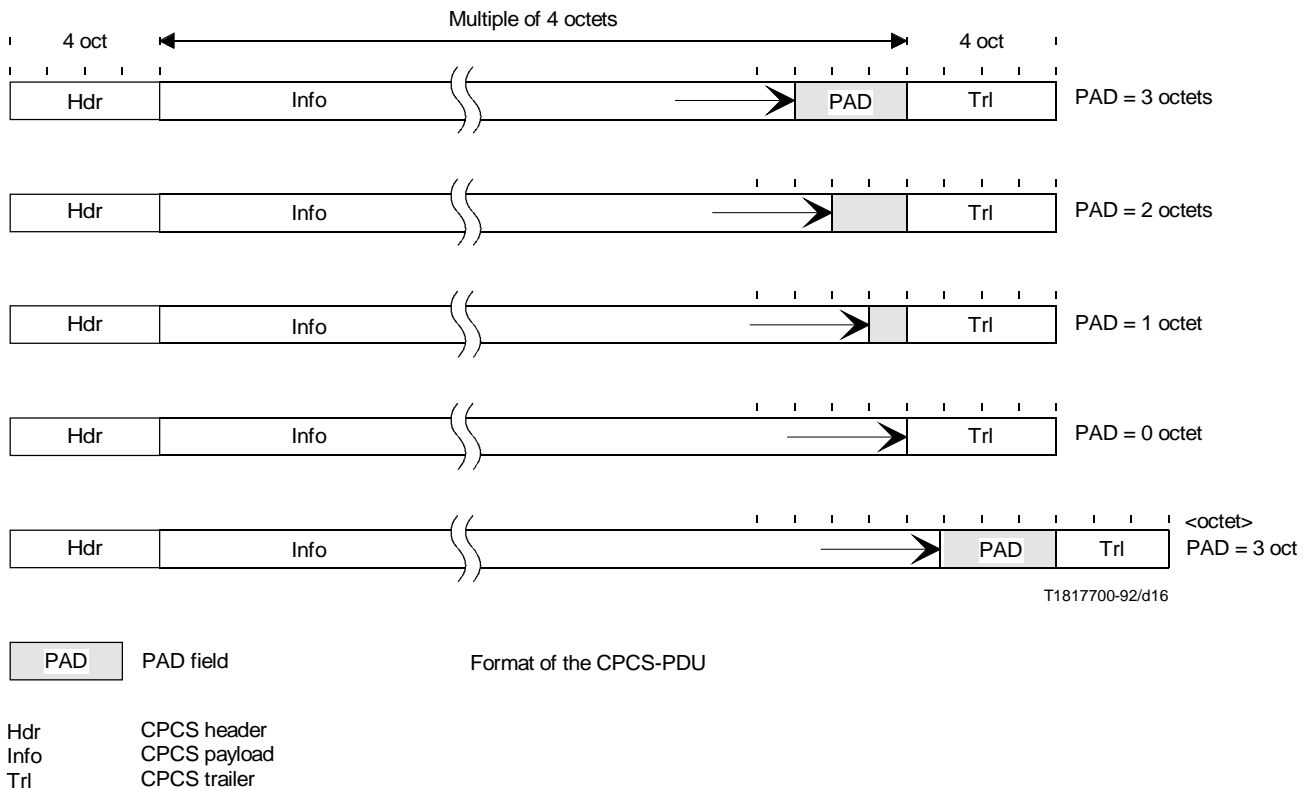
FIGURE 16/I.363 Function of the PAD field
