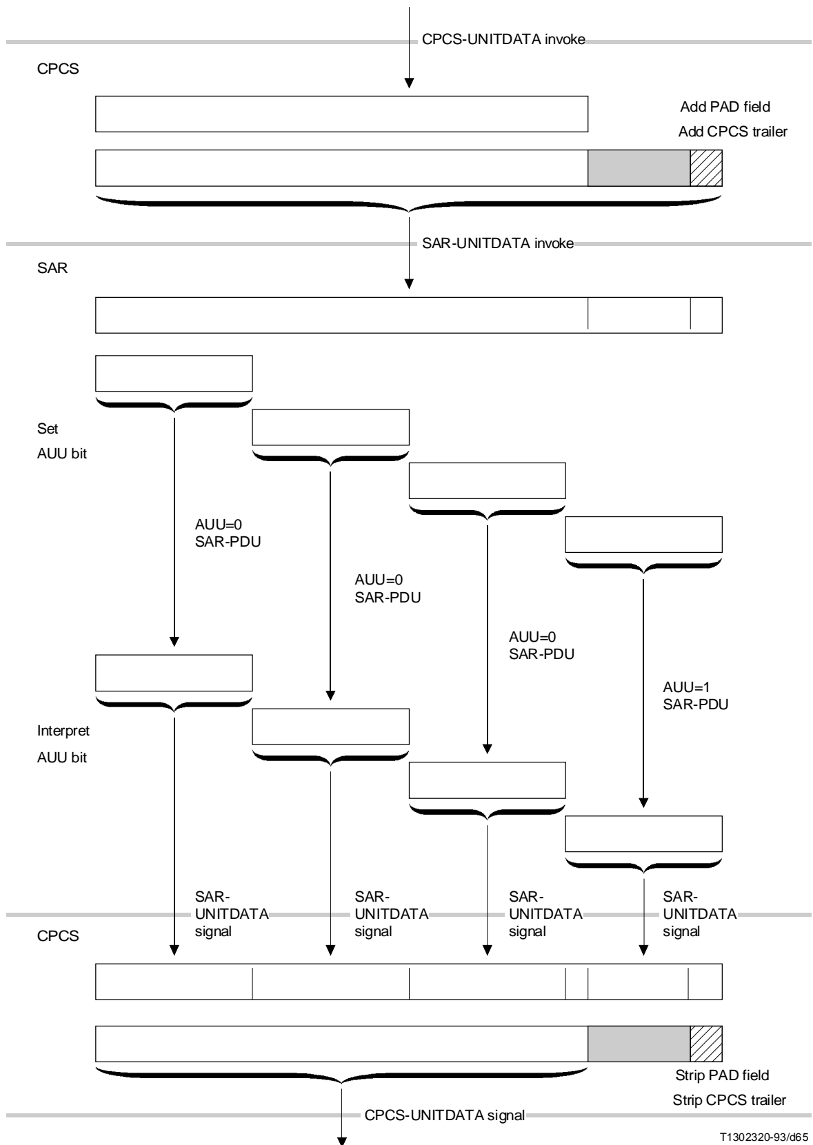
FIGURE F.3/I.363 Successful segmentation and reassembly of a CPCS user PDU
