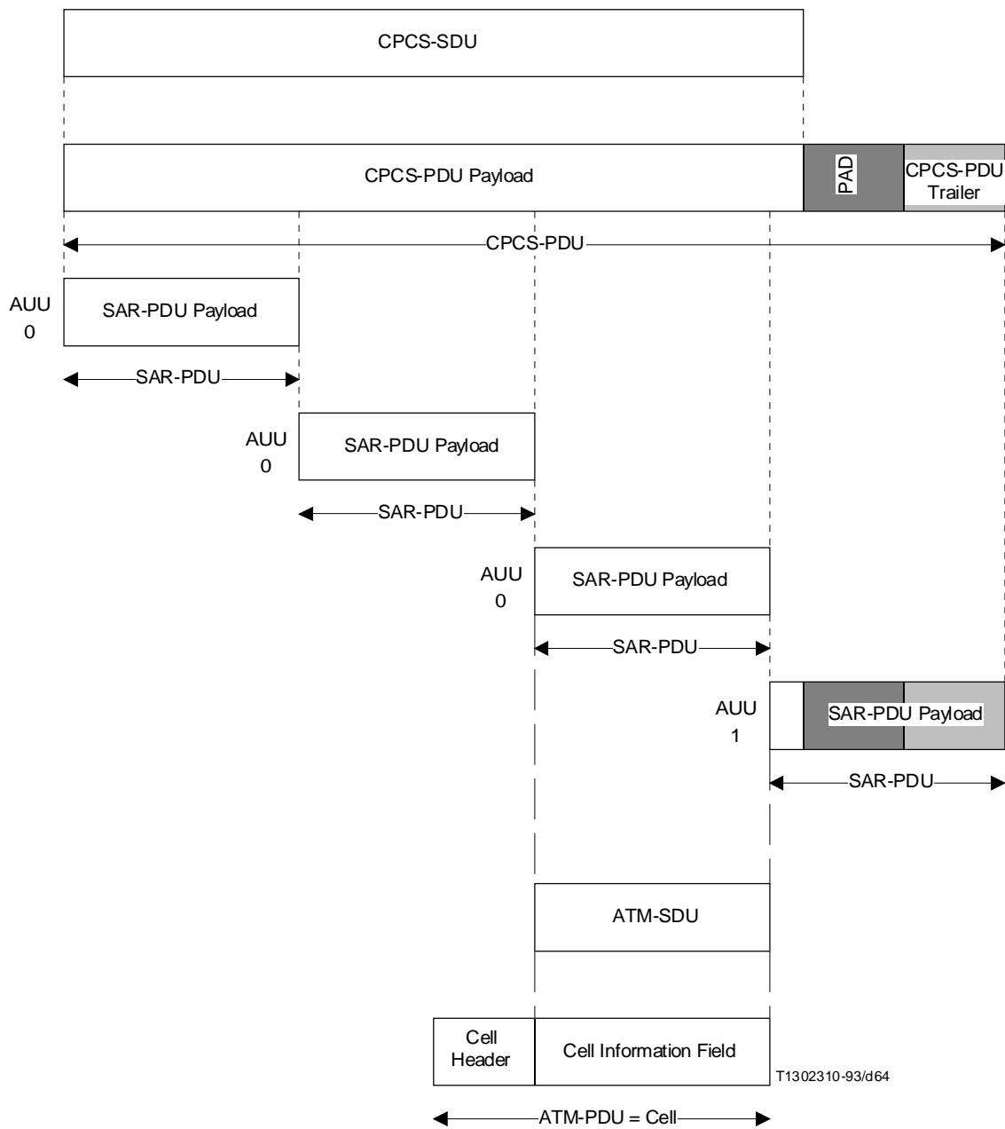
FIGURE F.2/I.363 PDU Headers, trailers and terminology
