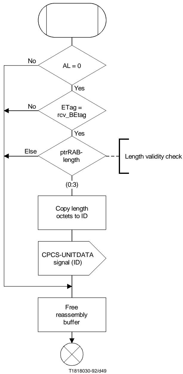
FIGURE I.5/L.363 (sheet 5 of 5)
