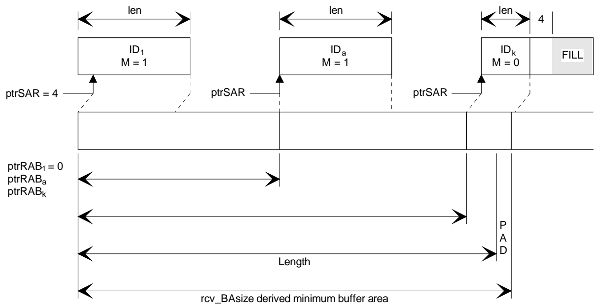
FIGURE I.3/I.363 The mechanism of the reassembly buffer
