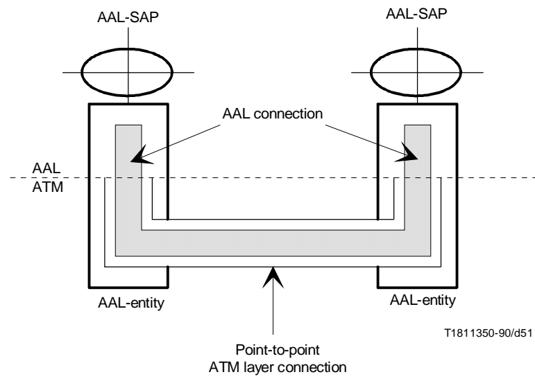
a) Point-to-point AAL connection
