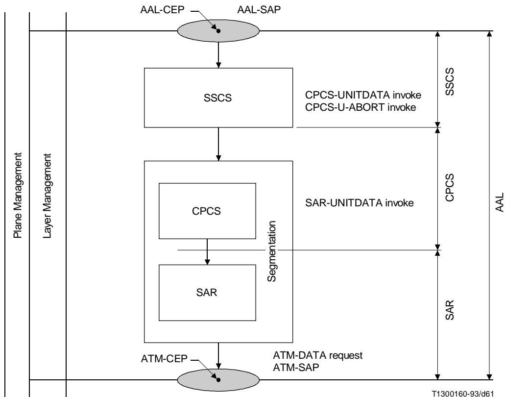
FIGURE E-1/I.363 Functional model for the AAL type 5 (sender side)
