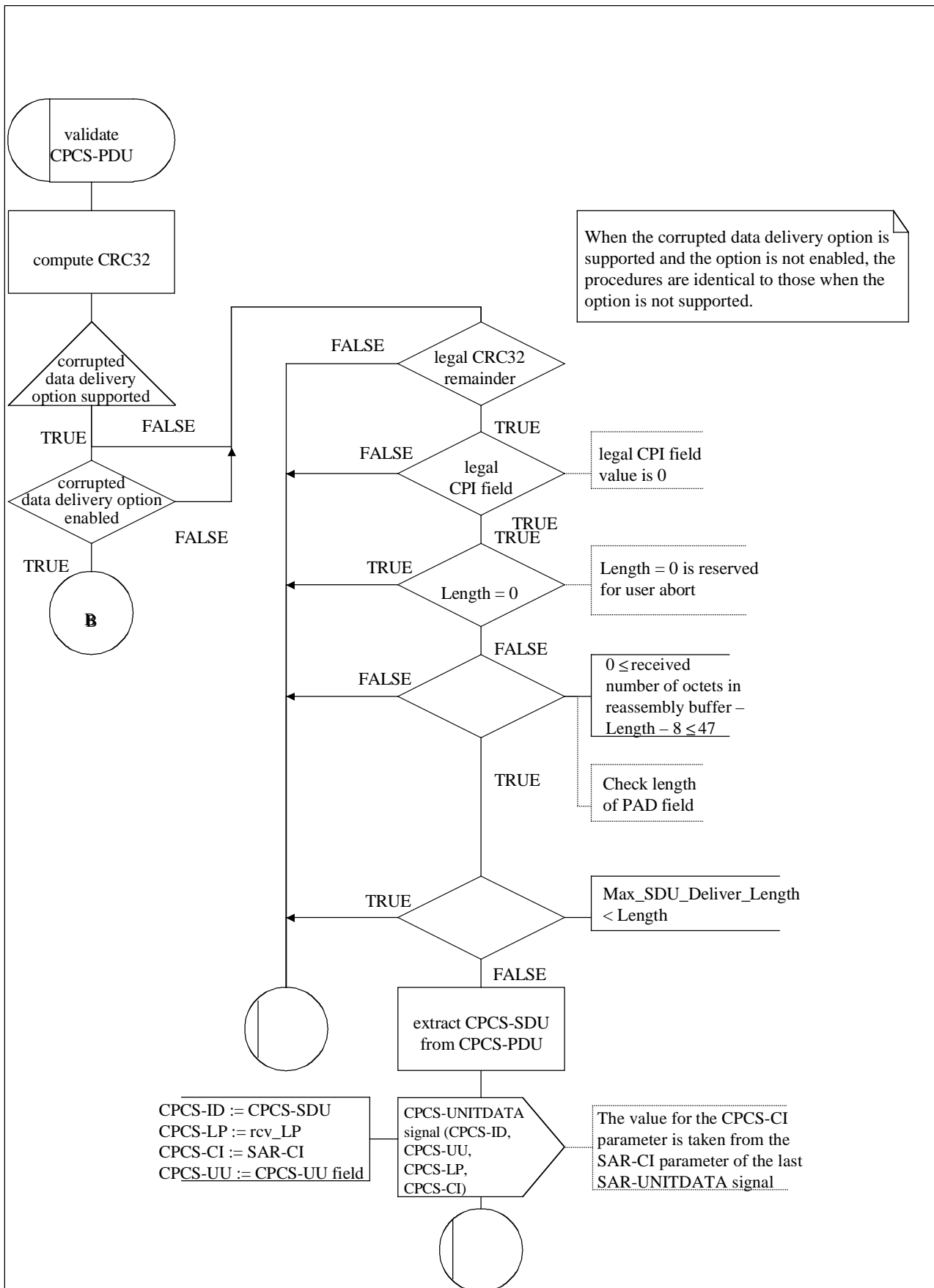
Figure E.2/I.363.5 (sheet 3 of 6) – CPCS receiver for the corrupted data delivery option
