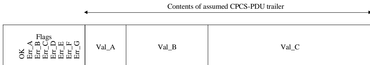
Figure E.1/I.363.5 – Model of the Reception Status parameter
