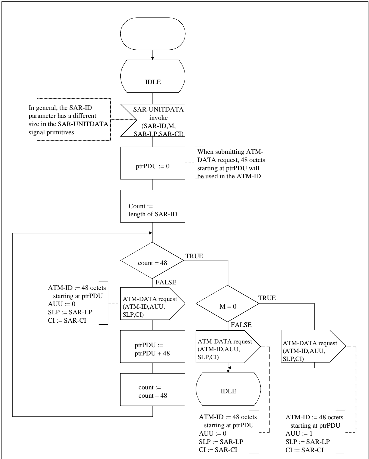
Figure D.1/I.363.5 – SDL diagrams for the SAR sender
