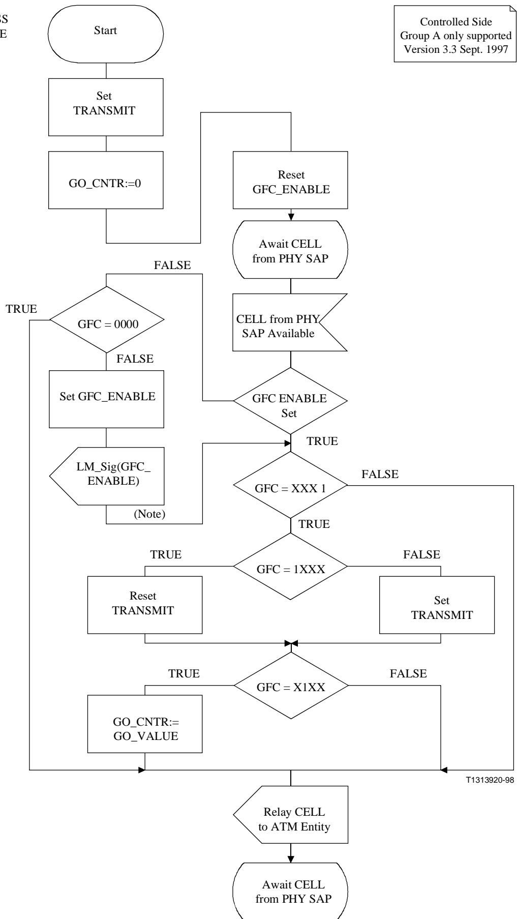
Figure B.11/I.361 – SDL diagrams for GFC mechanism at the multiaccess UNI (Part 1 of 2)
