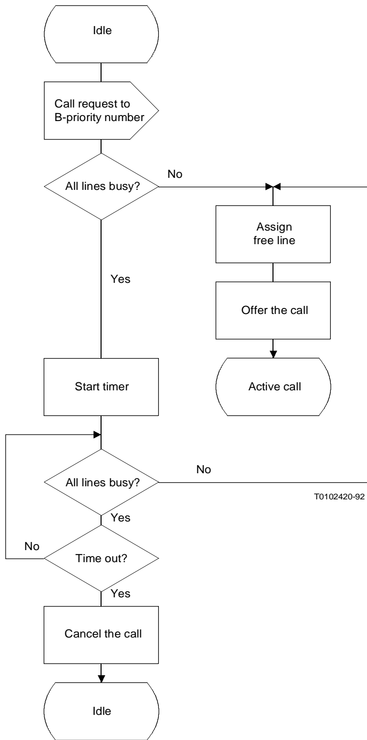
FIGURE 2/I.255.4 Overall SDL diagram for the case of B-priority
