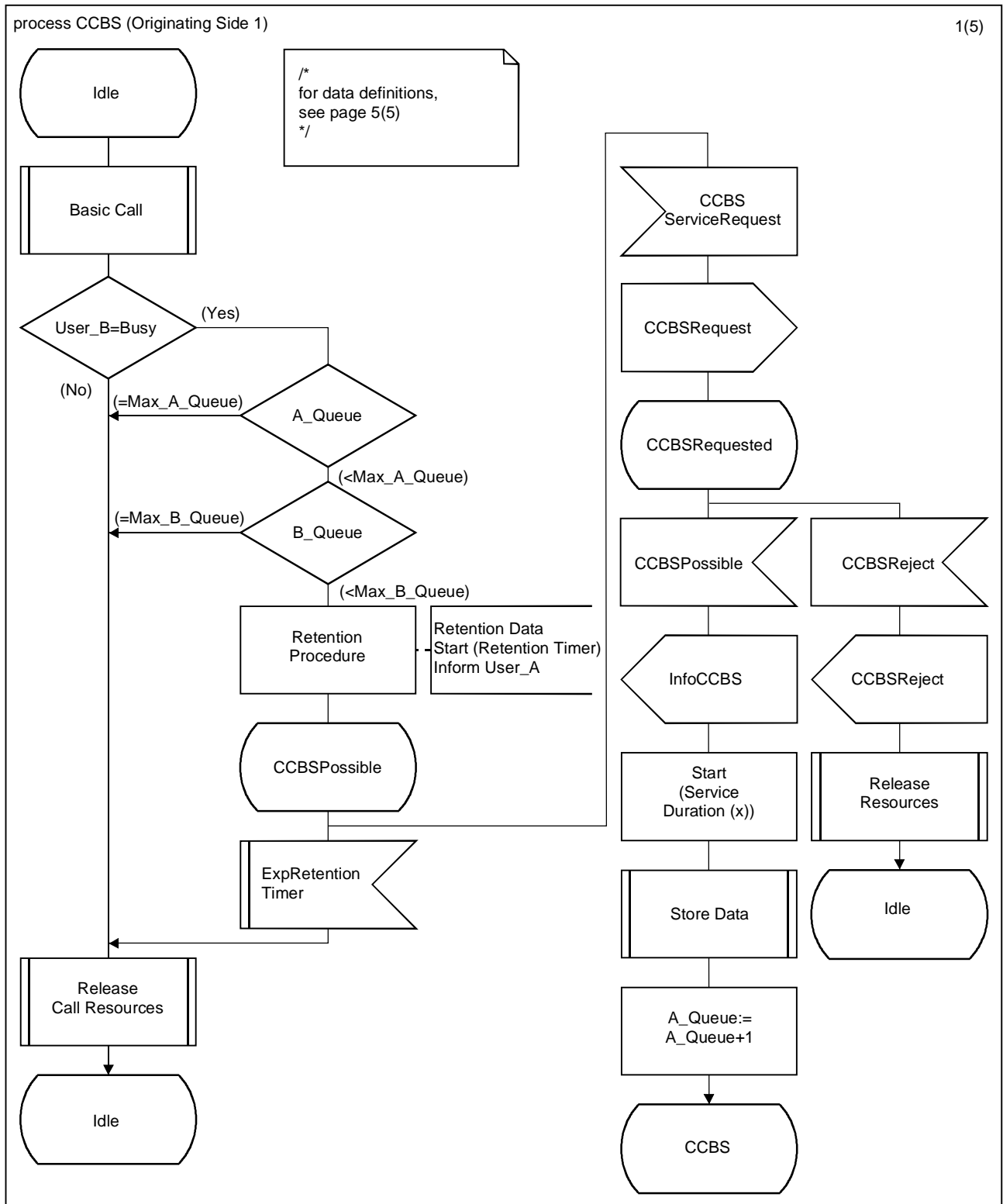
FIGURE 1/I.253.3 (sheet 1 of 5)
