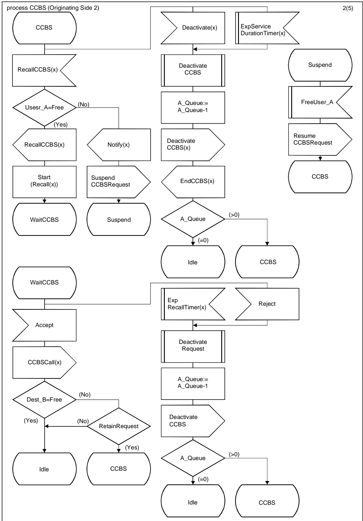
FIGURE 1/I.253.3 (sheet 2 of 5) CCBS SDL description
