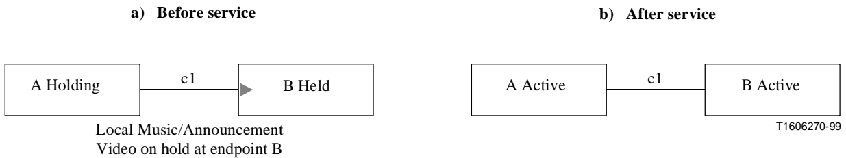
Figure 10/H.450.4 – Operational model for retrieve from remote-end call hold
