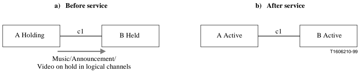
Figure 4/H.450.4 – Operational model for retrieve from near-end call hold
