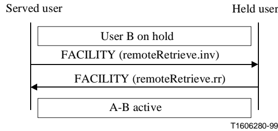
Figure 11/H.450.4 – Signalling flow for retrieve from remote-end call hold
