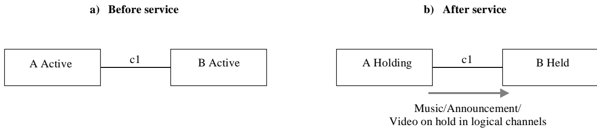
Figure 1/H.450.4 – Operational model for near-end call hold
