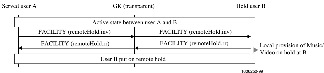
Figure 8/H.450.4 – Signalling flow for remote-end call hold – GK routed model – GK transparent
