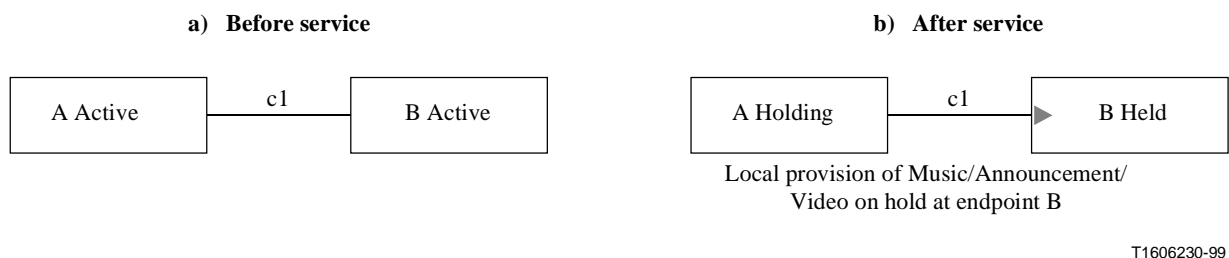
Figure 6/H.450.4 – Operational model for remote-end call hold
