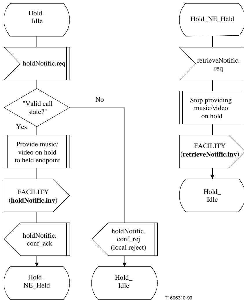
Figure 14/H.450.4 – Near-end call hold – Holding SDL
