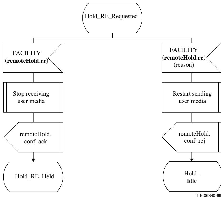
Figure 17/H.450.4 – Remote-end call hold – Holding SDL (sheet 2 of 3)
