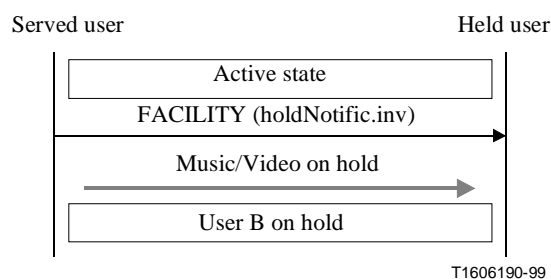
Figure 2/H.450.4 – Signalling flow for near-end call hold
