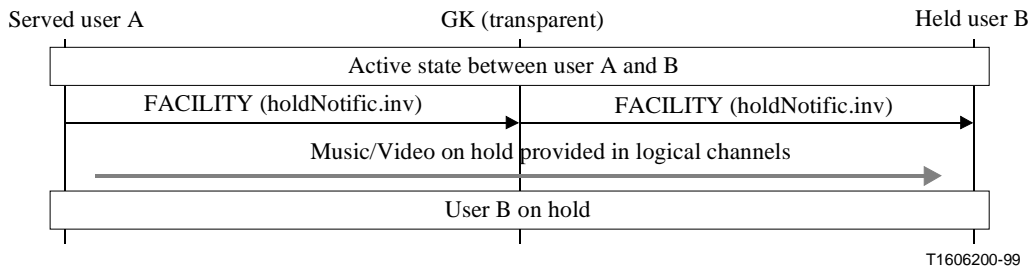
Figure 3/H.450.4 – Signalling flow for near-end call hold for a GK routed model
