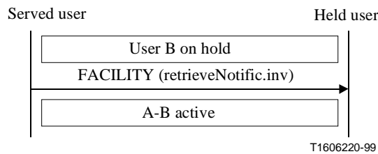
Figure 5/H.450.4 – Signalling flow for retrieve from near-end call hold
