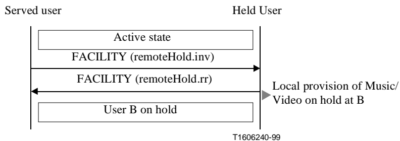
Figure 7/H.450.4 – Signalling flow for remote-end call hold
