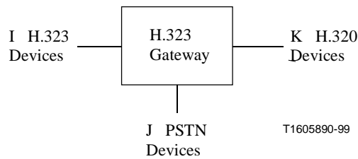
Figure 1/H.341 – Model of an H.323 Gateway
