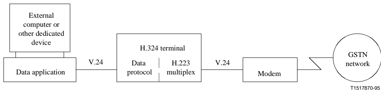
Figure 2/H.324 – Data application – Data protocol interface
