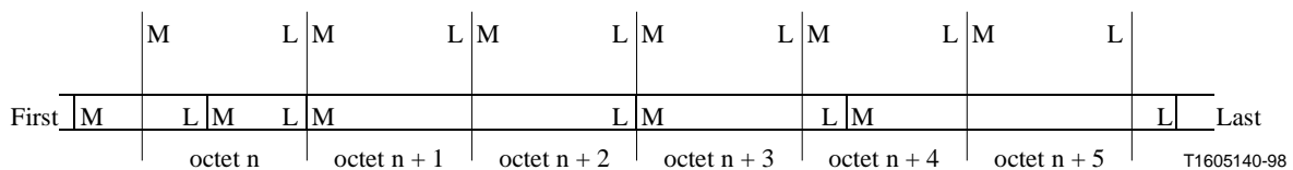
Figure I.2/H.324 – Output split into octets
