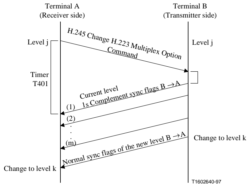
Figure C.1/H.324 – Level or option change procedure
