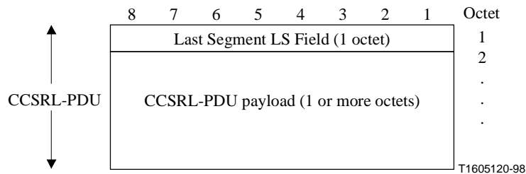
Figure C.3/H.324 – CCSRL-PDU Format
