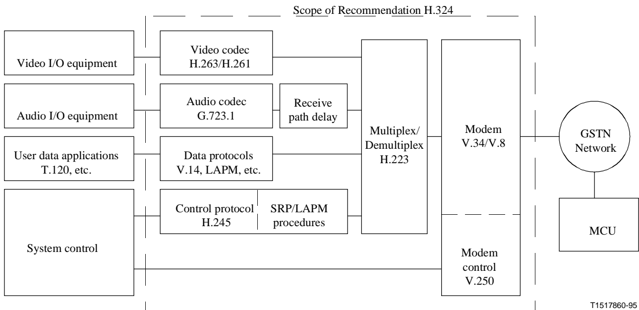
Figure 1/H.324 – Block diagram for H.324 multimedia system
