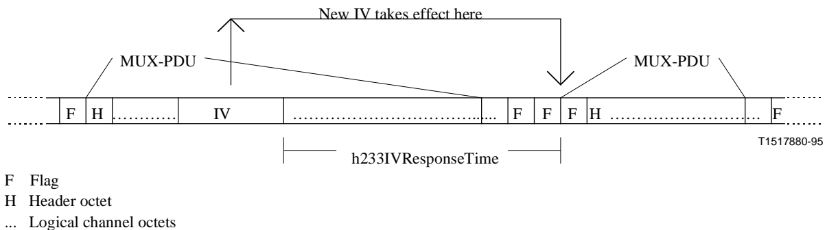
Figure 3/H.324 – Encryption IV synchronization
