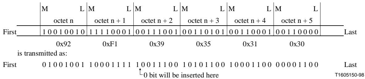
Figure I.3/H.324 – Example sequence
