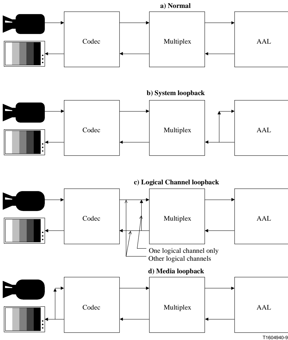
Figure 7/H.310 – Maintenance loops
