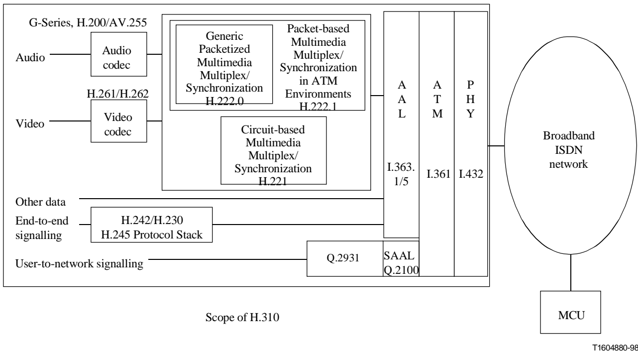
Figure 1/H.310 – Broadband audiovisual communication system and terminal configuration
