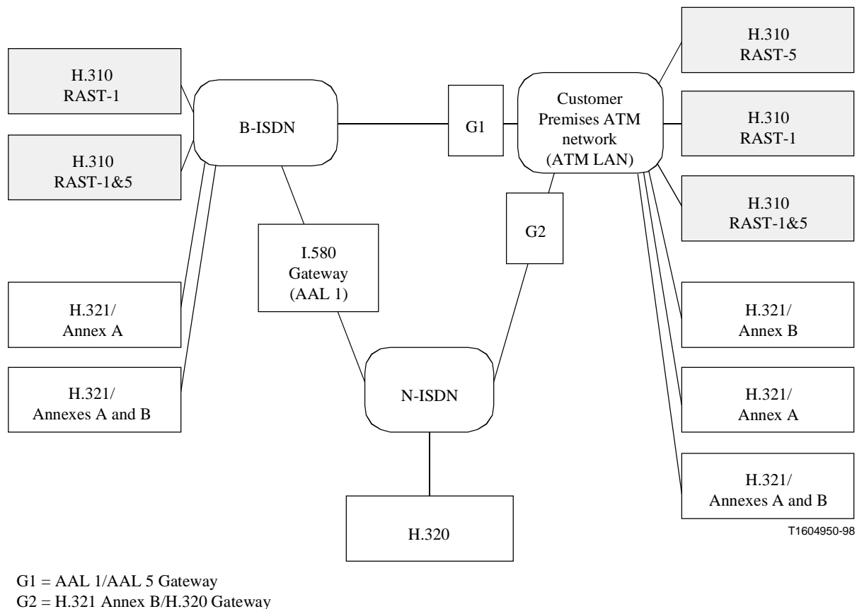
Figure 8/H.310 – Interworking of H.310 terminals
