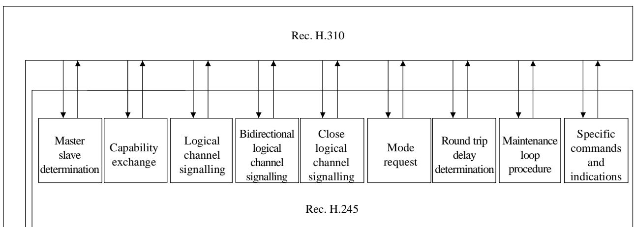
Figure 4/H.310 – Configuration of H.245 entities in H.310 terminal
