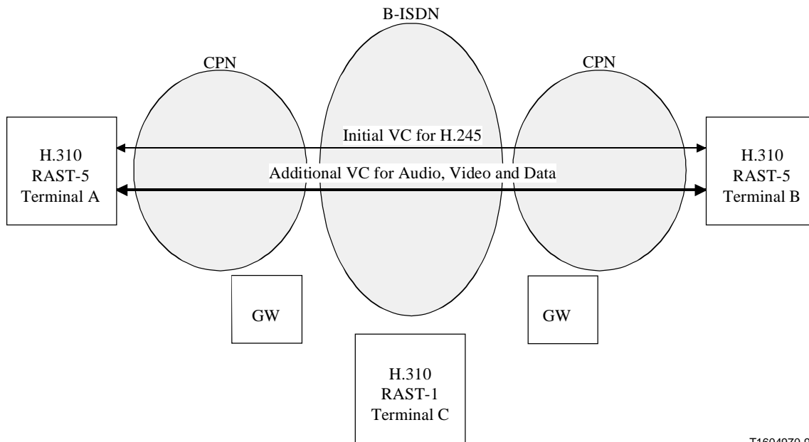
Figure C.1/H.310 – Communication between two RAST-5 terminals
