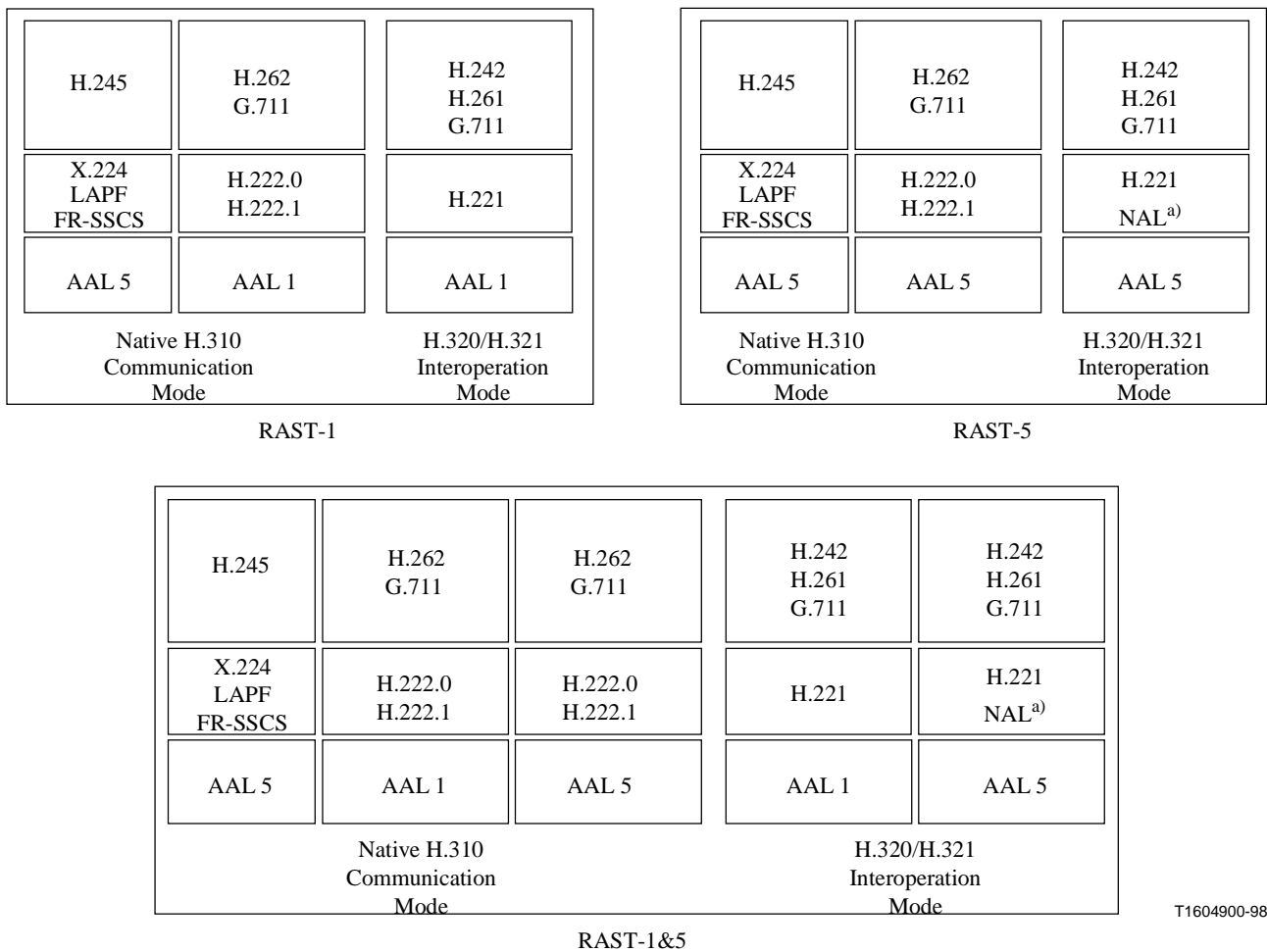
Figure 3/H.310 – Protocol stacks for native H.310 and H.320/H.321 interoperation communication modes
