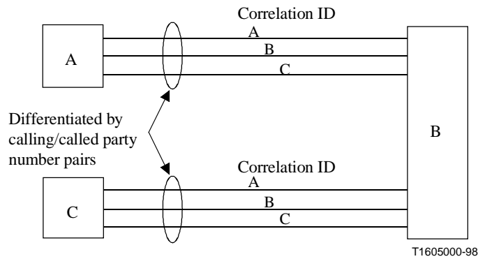
Figure II.1/H.310 – Identification of VCs in single session case
