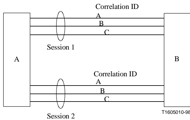
Figure II.2/H.310 – Identification of VCs in multi-session case
