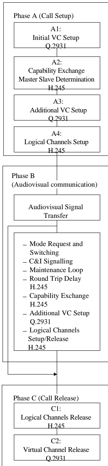
Figure 6/H.310 – H.310 call phases for native H.310 communication
