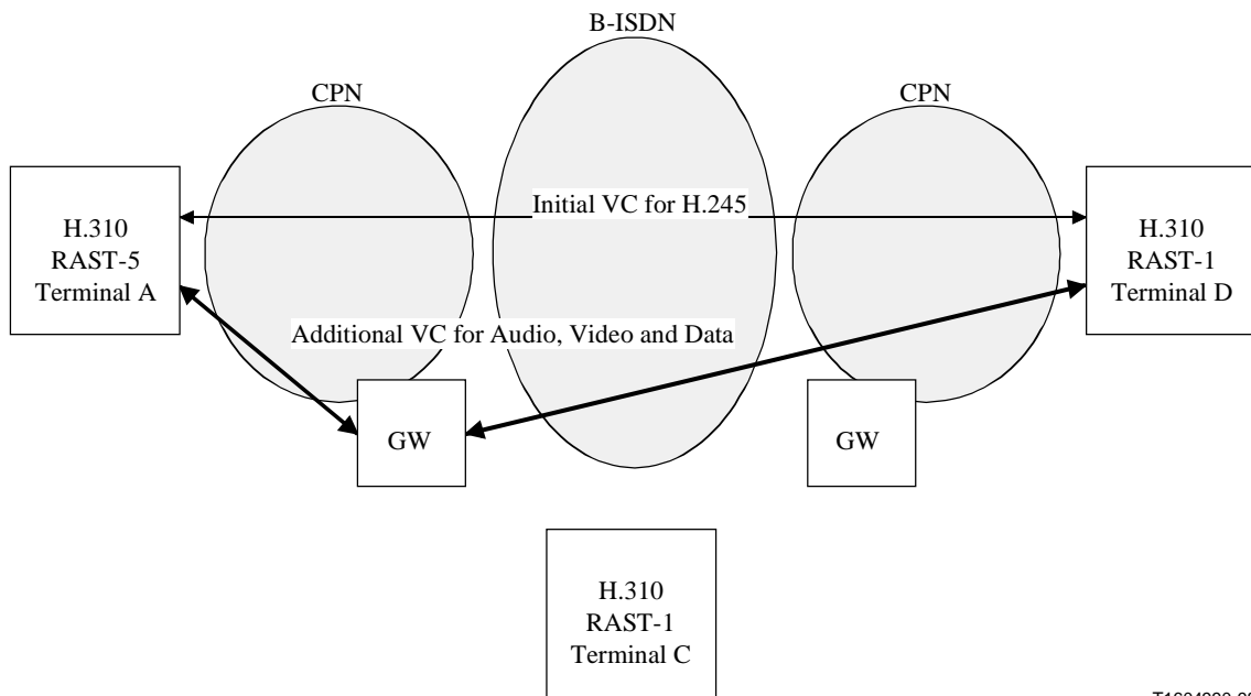
Figure C.3/H.310 – Communication between RAST-5 on CPN and RAST-1 on CPN
