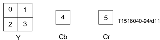
Figure 6-10 – 4:2:0 Macroblock structure
