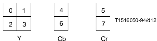
Figure 6-11 – 4:2:2 Macroblock structure
