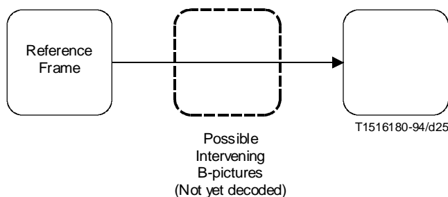
Figure 7-10 – Frame-prediction for I-pictures and P-pictures
