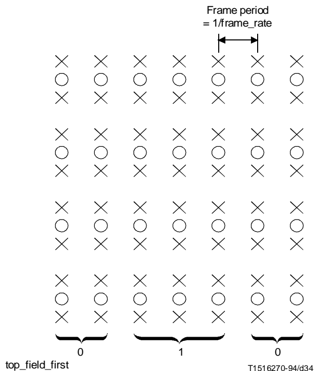
Figure 7-19 – progressive_sequence == 1, repeat_first_field = 1
