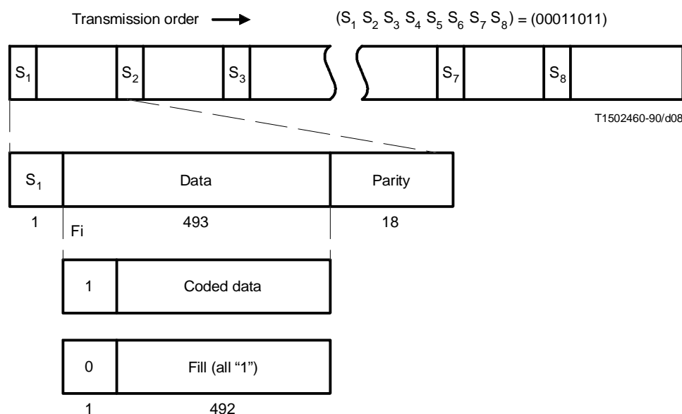
FIGURE 13/H.261 Error correcting frame
