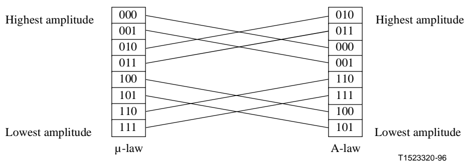
Figure X.1/H.242 – Order of segments according to amplitude, \mu -law and A-law PCM
