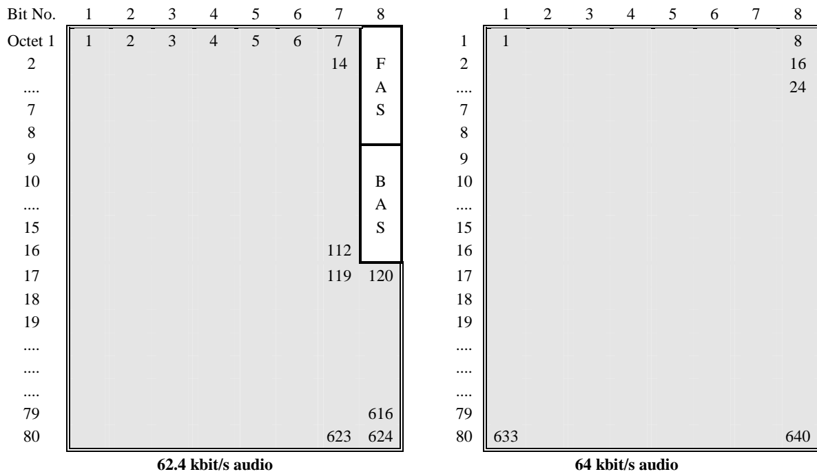
Figure 6c/H.221 – Bit positions for ISO/IEC 11172-3 audio in one or two 64 kbit/s channels: 62.4 and 64 kbit/s audio streams
