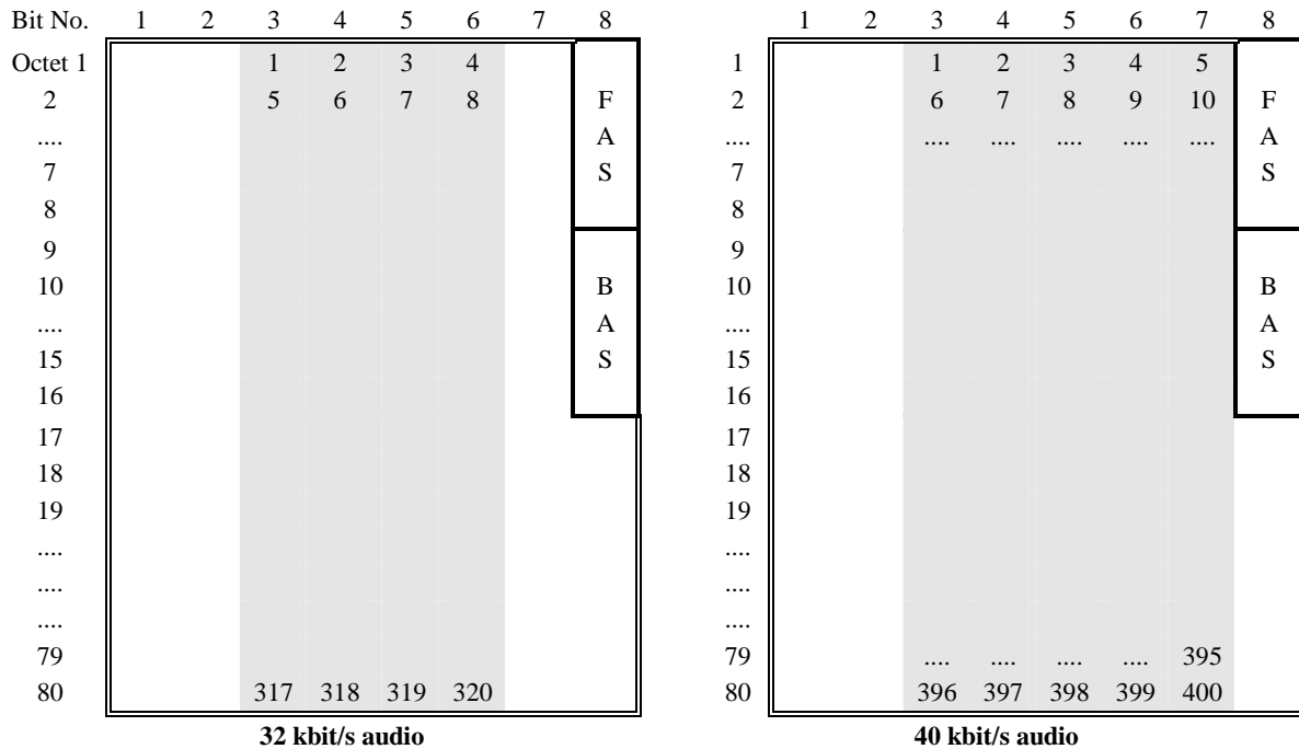
Figure 6a/H.221 – Bit positions for ISO/IEC 11172-3 audio in one or two 64 kbit/s channels: 32 and 40 kbit/s audio streams
