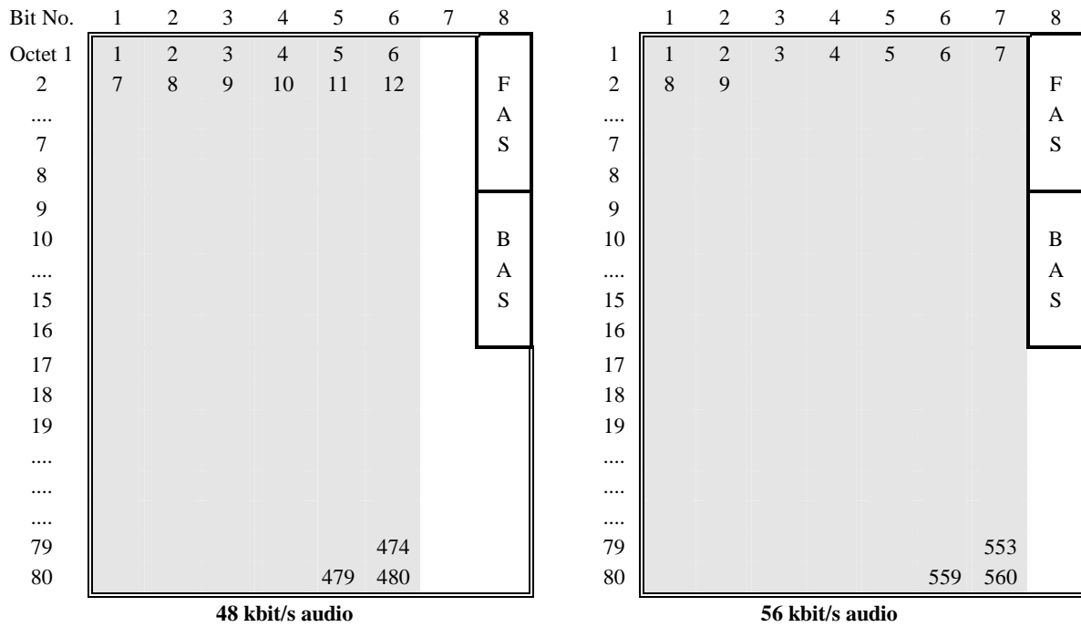
Figure 6b/H.221 – Bit positions for ISO/IEC 11172-3 audio in one or two 64 kbit/s channels: 48 and 56 kbit/s audio streams
