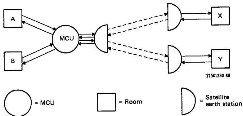
FIGURE 2/H.140 Use of a single MCU in a satellite configuration
