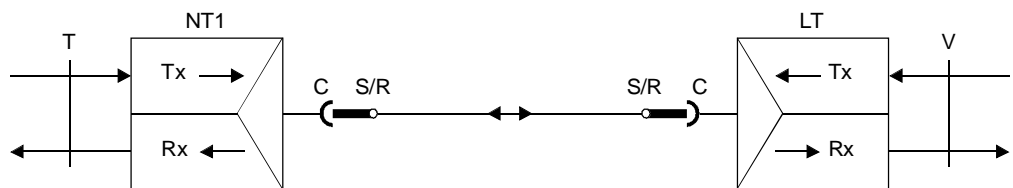
b) One-fibre system
