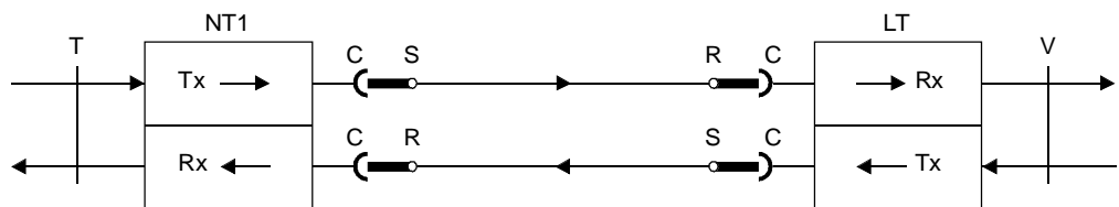
a) Two-fibre system
