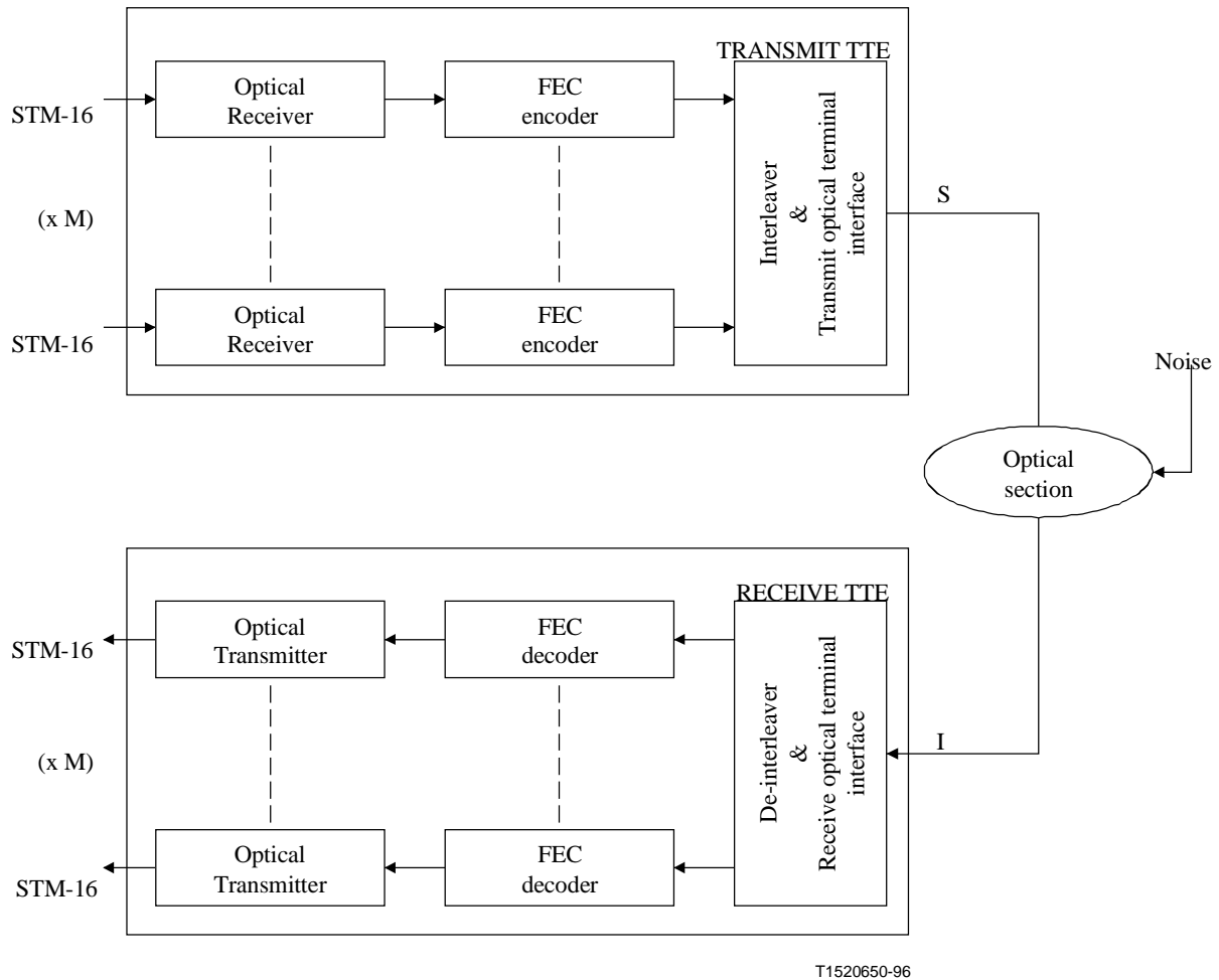
Figure 1/G.975 – Block diagram of a submarine system which uses a FEC function
