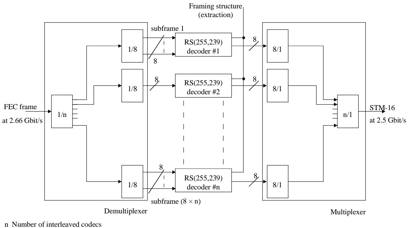
Figure 3/G.975 – FEC decoder architecture
