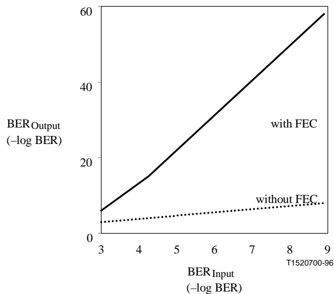
Figure 6/G.975 – Theoretical output versus input BER
