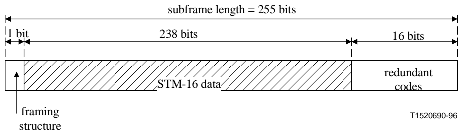
Figure 5/G.975 – Content of the subframes of the FEC frame
