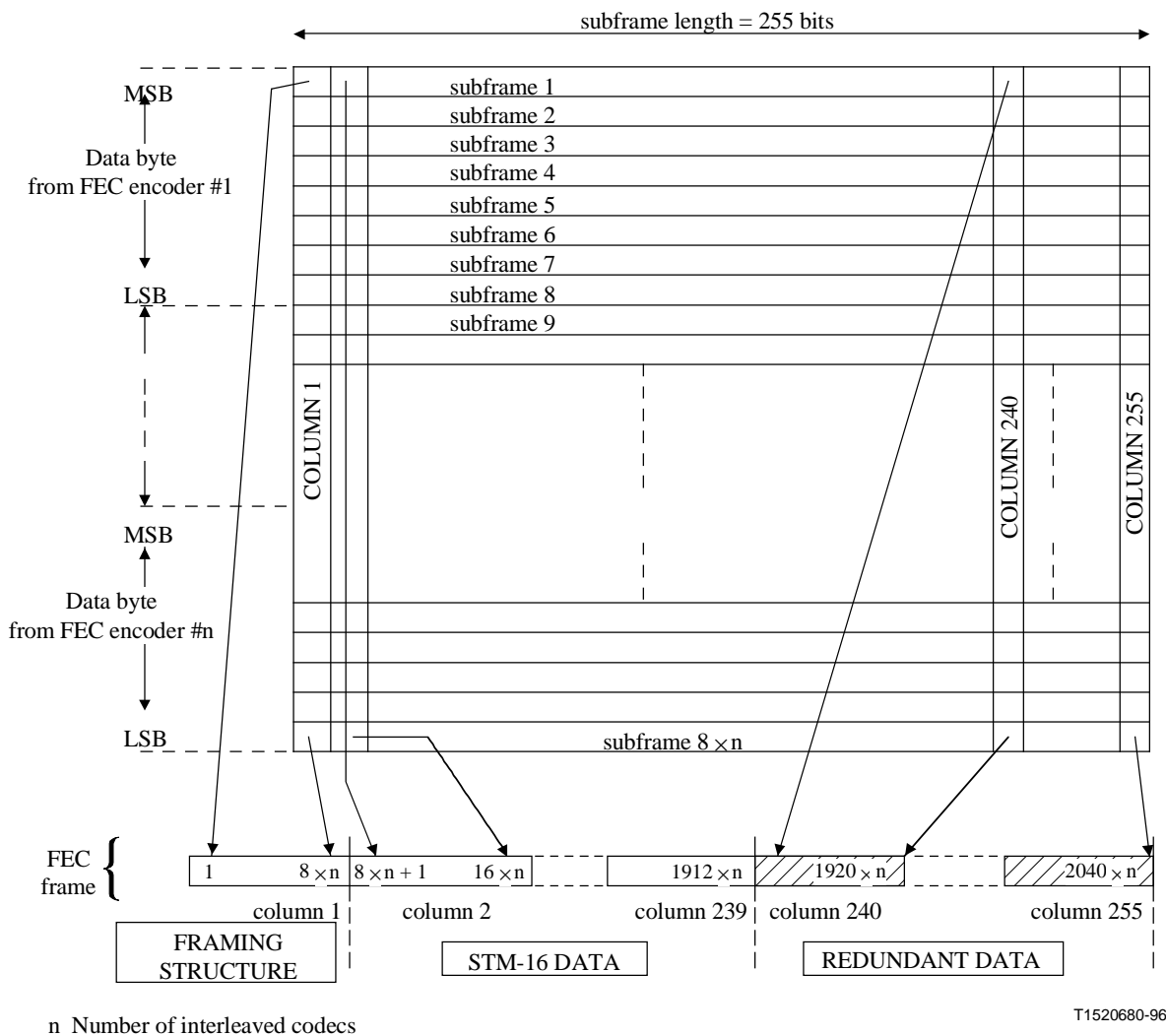
Figure 4/G.975 – FEC frame construction
