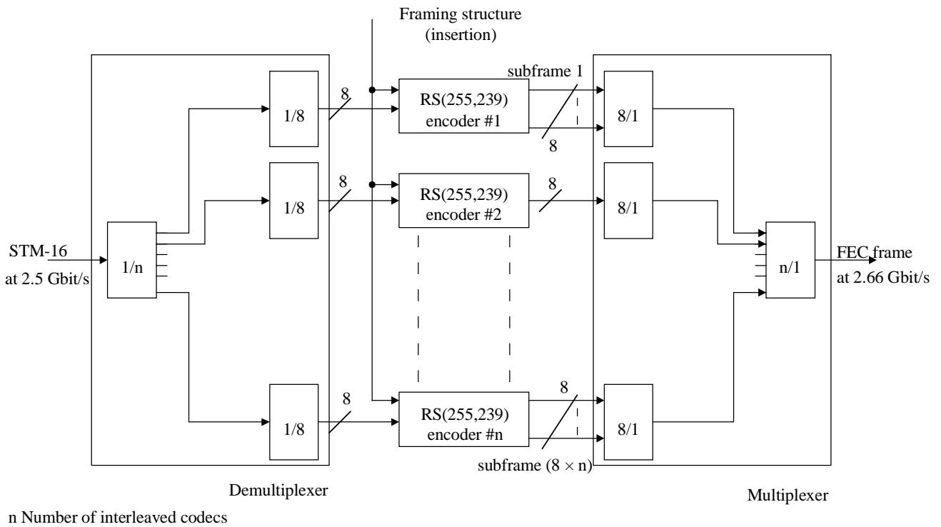
Figure 2/G.975 – FEC encoder architecture
