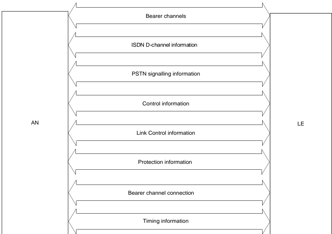
FIGURE 5/G.965 Functional description of the V5.2 interface
