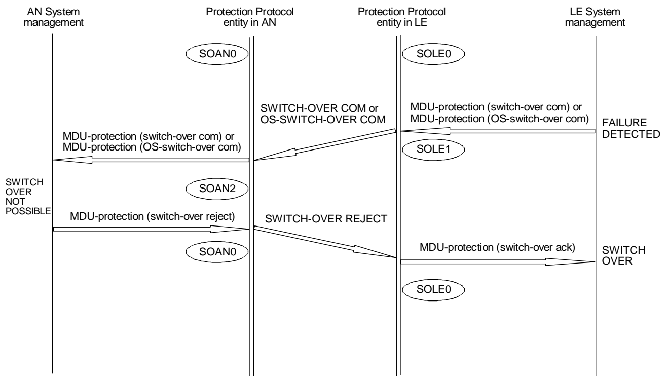
FIGURE J.3/G.965 Rejection of LE-initiated switch-over by AN
