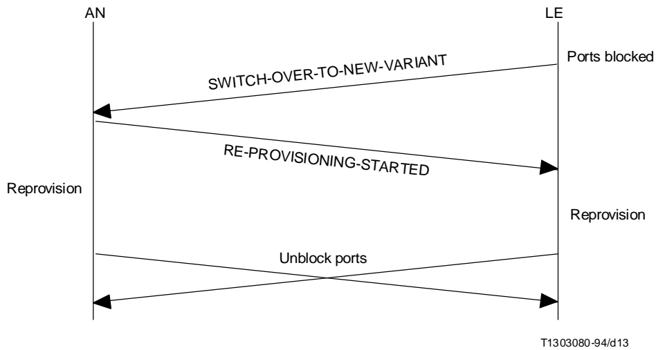
FIGURE C.1/G.965 Procedure for re-provisioning initiated from LE
