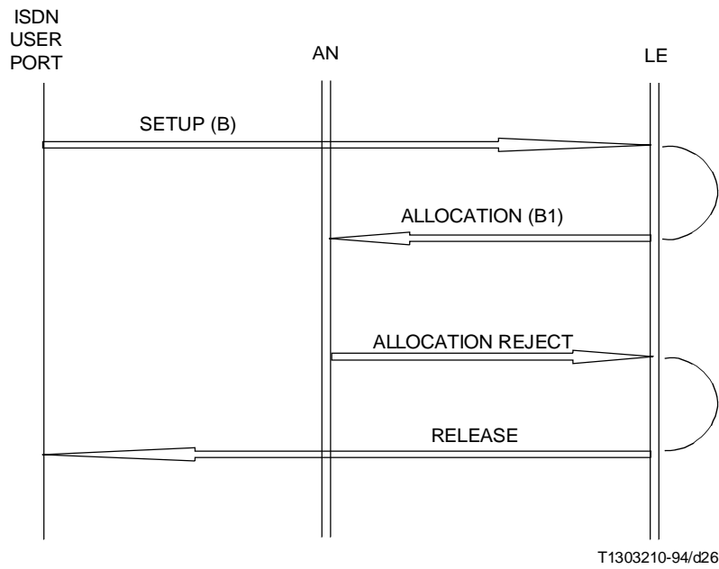
FIGURE K.2/G.965 ISDN call initiated by subscriber – Exceptional procedure
