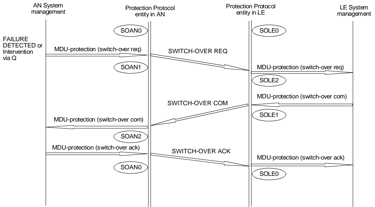
FIGURE J.2/G.965 AN-initiated autonomous switch-over
