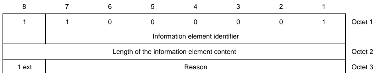
FIGURE 24/G.965 Connection Incomplete information element
